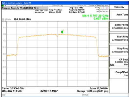
ANT1_802.11ax_HE40_UNII 3
