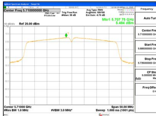
ANT2_802.11n_HT40_UNII 2C
