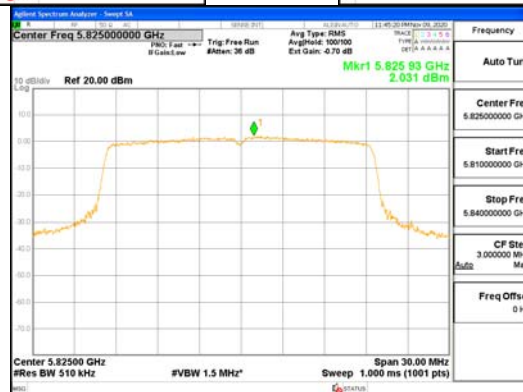
ANT2_802.11ax_HE20_UNI1 3
