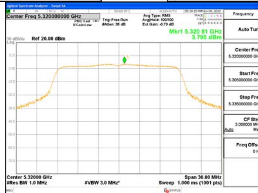
ANT2_802.11n_HT20_UNII 2A
