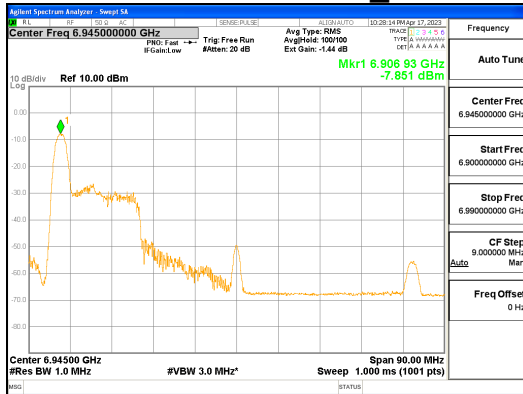
ANT0_802.11ax_HE80_26T_Low_UNII 8
