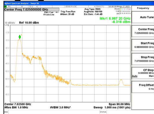
ANT0_802.11ax_HE80_26T_Low_UNII 8
