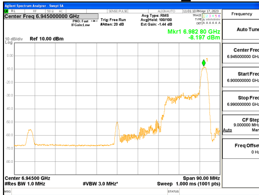
ANTO_802.11ax_HE80_26T_High_UNII 8
