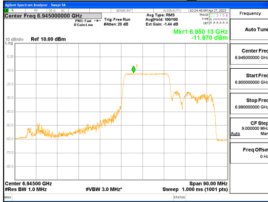
ANT1_802.11ax_HE80_242T_Mid_UNII 8
