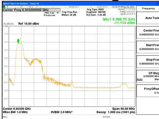
ANT1_802.11ax_HE80_52T_Low_UNII 8
