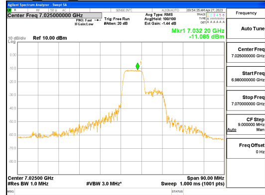
ANT1_802.11ax_HE80_106T_Mid_UNII 8
