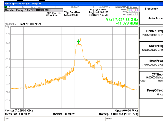
ANT1_802.11ax_HE80_52T_Mid_UNII 8
