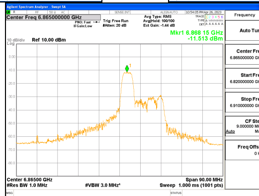
ANT1_802.11ax_HE80_52T_Mid_UNII 7
