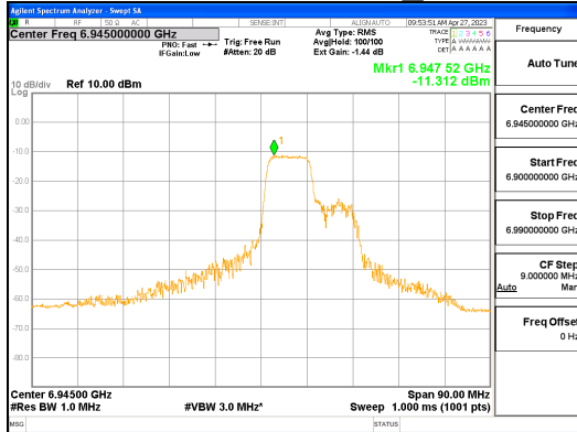
ANT1_802.11ax_HE80_106T_Mid_UNII 8
