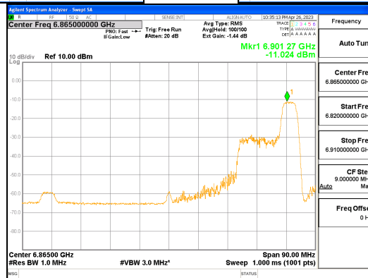
ANT1_802.11ax_HE80_52T_High_UNII 7
