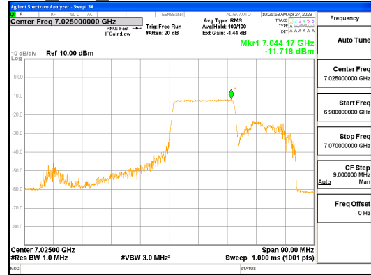
ANT1_802.11ax_HE80_242T_Mid_UNII 8
