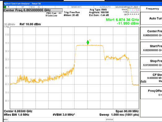
ANT1_802.11ax_HE80_242T_Mid_UNII 7
