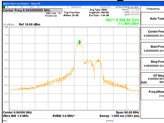
ANT1_802.11ax_HE80_52T_Mid_UNII 8
