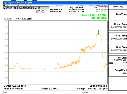
ANT1_802.11ax_HE80_52T_High_UNII 8
