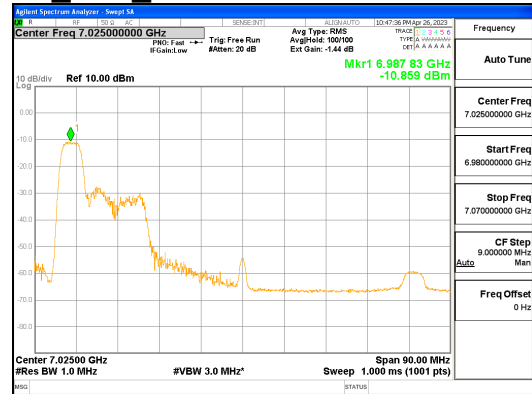
ANT1_802.11ax_HE80_52T_Low_UNII 8
