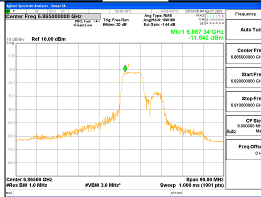
ANT1_802.11ax_HE80_106T_Mid_UNII 7
