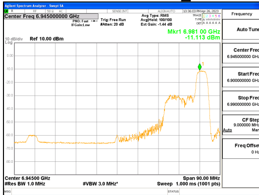
ANT1_802.11ax_HE80_52T_High_UNII 8
