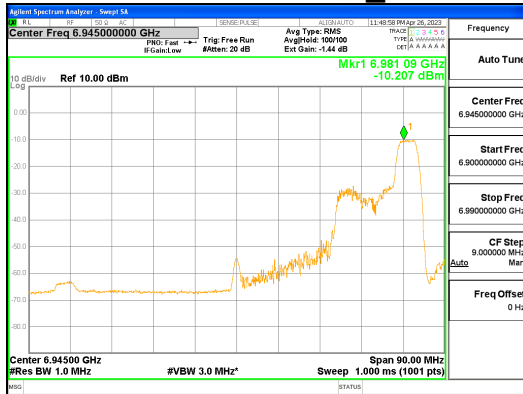
ANTO_802.11ax_HE80_52T_High_UNII 8
