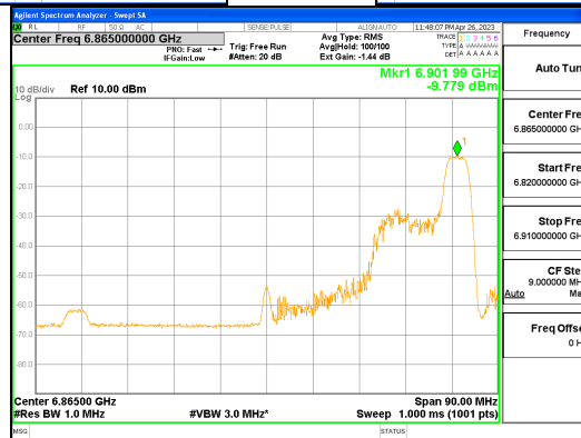
ANTO_802.11ax_HE80_52T_High_UNII 7
