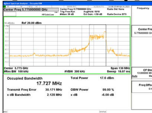
ANT1_802.11ax_HE80_26T_High_UNII 3
