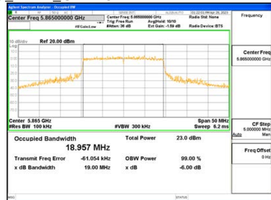
ANT1_802.11ax_HE20_242T_UNII 3
