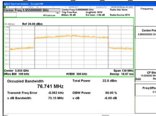
ANT1_802.11ax_HE80_996T_UNII 4
