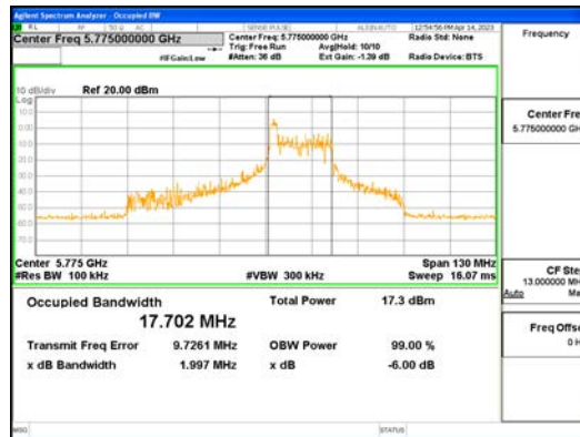
ANT0_802.11ax_HE80_26T_Mid_UNI1 3
