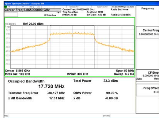
ANT1_802.11ac_VHT20_UNII 3
