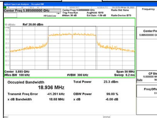
ANT1_802.11ax_HE20_242T_UNII 4
