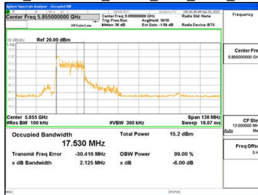
ANT1_802.11ax_HE80_26T_Low_UNII 4
