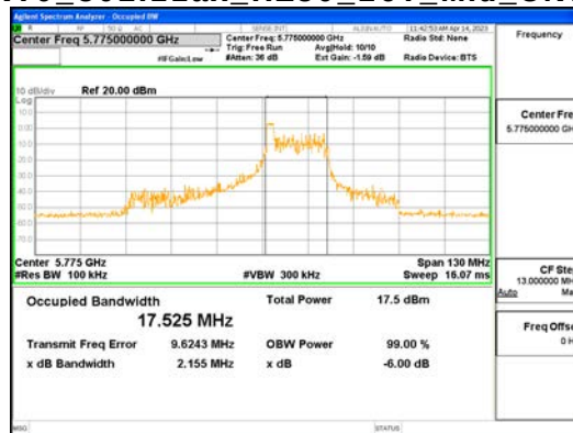
ANT1_802.11ax_HE80_26T_Mid_UNI1 3
