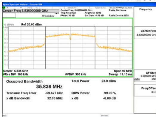
ANT1_802.11n_HT40_UNI1 4
