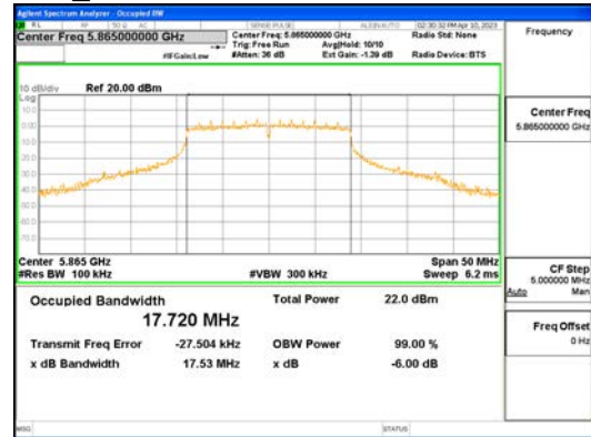
ANT0_802.11ac_VHT20_UNII 3
