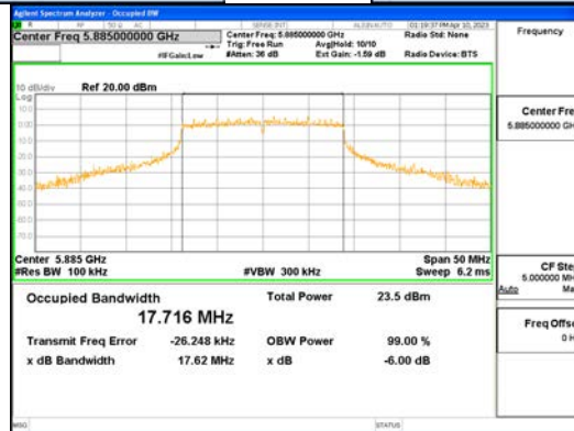
ANT1_802.11ac_VHT20_UNII 4
