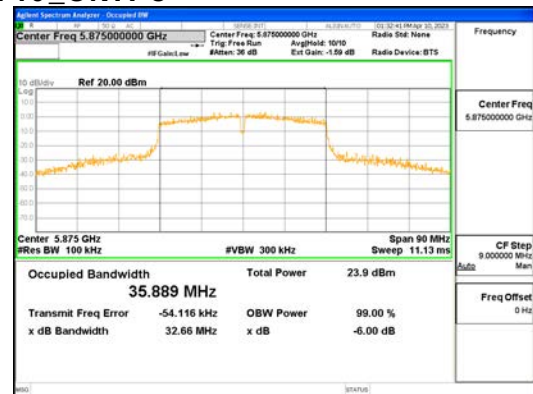
ANT1_802.11n_HT40_UNI1 4
