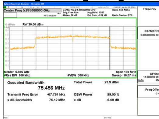
ANT1_802.11ac_VHT80_UNII 4
