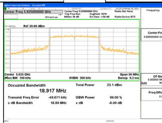
ANT1_802.11ax_HE20_242T_UNII 3
