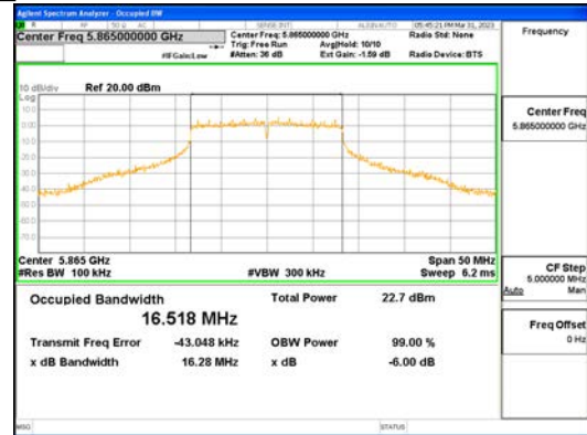
ANT1_802.11a_UNII 3
