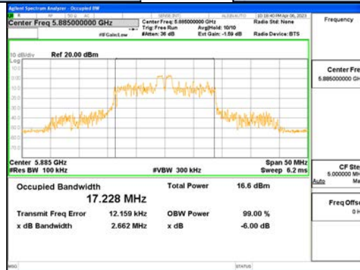
ANT1_802.11ax_HE20_26T_Mid_UNI1 4
