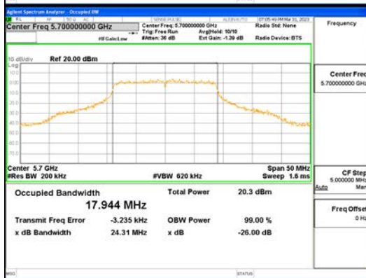
ANT0_802.11n_HT20_UNII 2C
