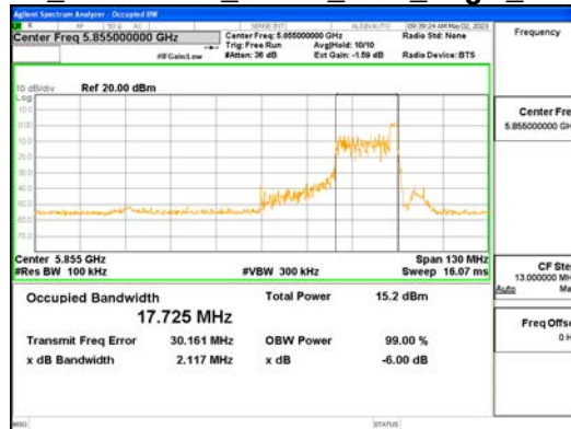
ANT1_802.11ax_HE80_26T_High_UNII 4
