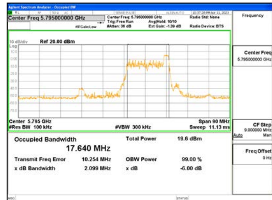
ANT0_802.11ax_HE40_26T_High_UNII 3
