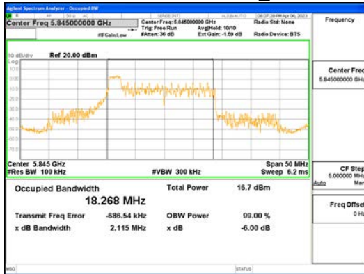
ANT1_802.11ax_HE20_26T_Low_UNII 3
