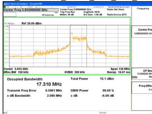
ANT1_802.11ax_HE80_26T_Mid_UNI1 4
