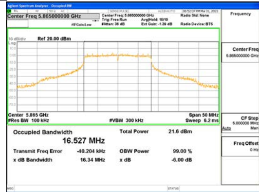
ANT0_802.11a_UNII 3
