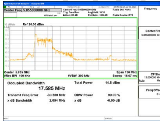
ANTO_802.11ax_HE80_26T_Low_UNII 4
