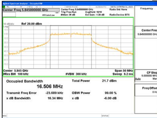
ANT0_802.11a_UNII 3
