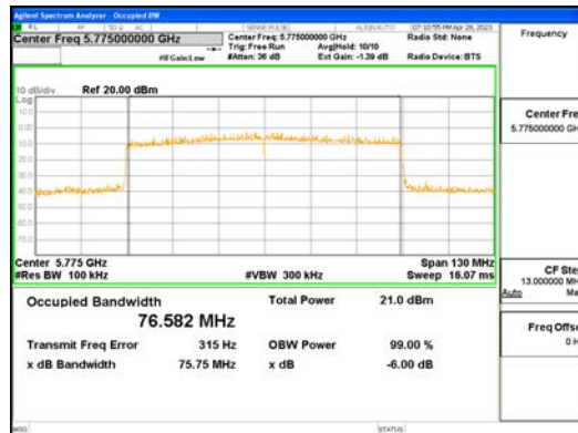
ANT0_802.11ax_HE80_996T_UNII 3
