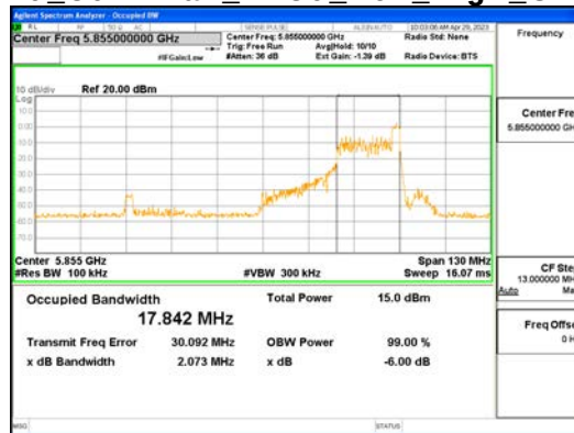
ANT0_802.11ax_HE80_26T_High_UNII 4
