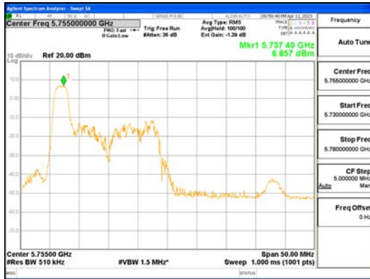
ANTO_802.11ax_HE40_26T_Low_UNII 3
