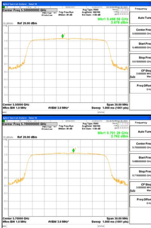
ANT1_802.11ax_HE20_242T_UNII 2C
