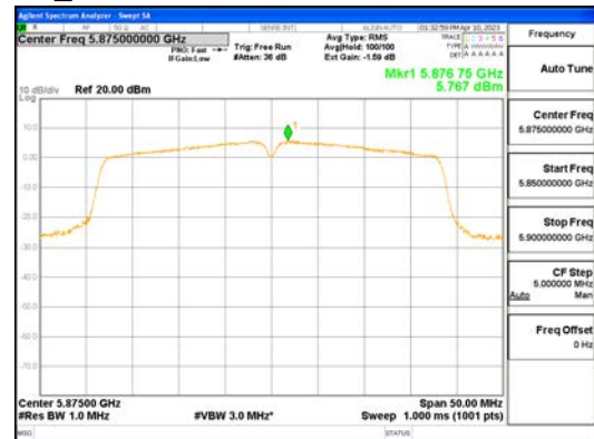
ANT1_802.11n_HT40_UNII 4
