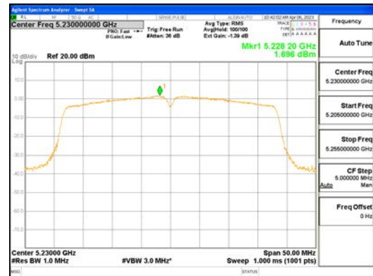
ANT0_802.11ac_VHT40_UNI1 1
