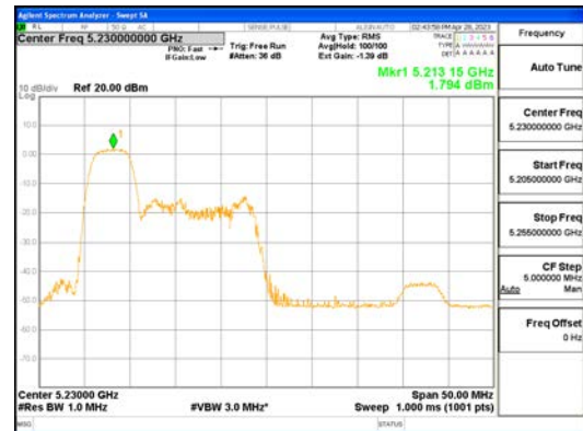
ANTO_802.11ax_HE40_52T_Low_UNII 1
