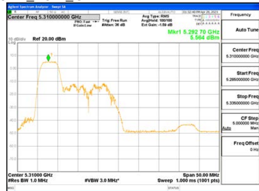
ANT1_802.11ax_HE40_52T_Low_UNII 2A
