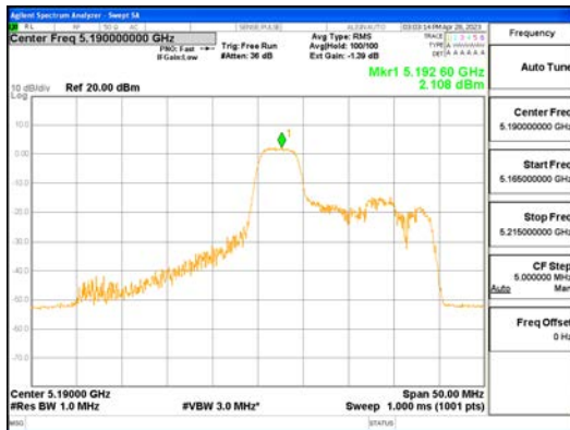
ANT0_802.11ax_HE40_52T_Mid_UNII 1
