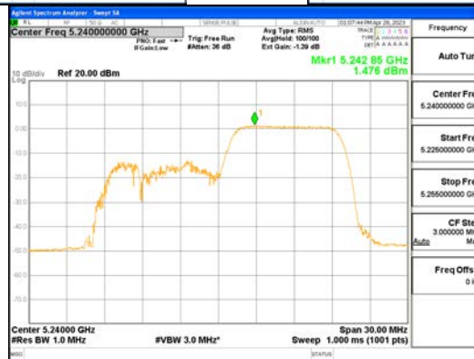
ANT0_802.11ax_HE20_106T_High_UNII 1
