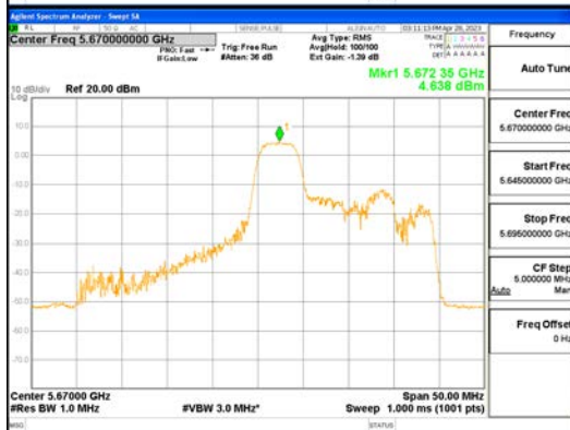
ANT0_802.11ax_HE40_52T_Mid_UNII 2C
