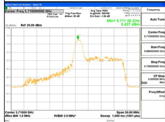
ANT0_802.11ax_HE40_26T_Mid_UNII 2C
