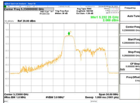
ANT0_802.11ax_HE40_52T_Mid_UNII 1
