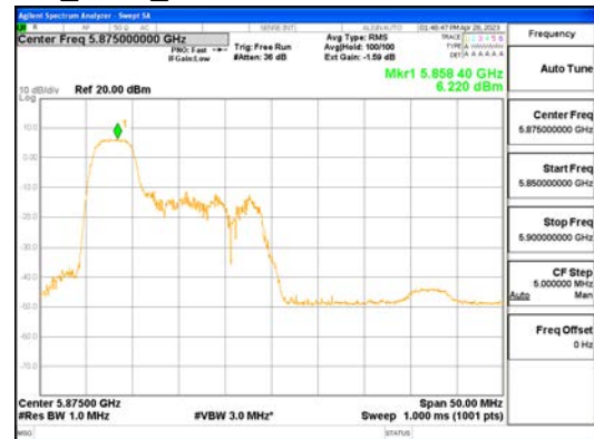
ANT1_802.11ax_HE40_52T_Low_UNII 4
