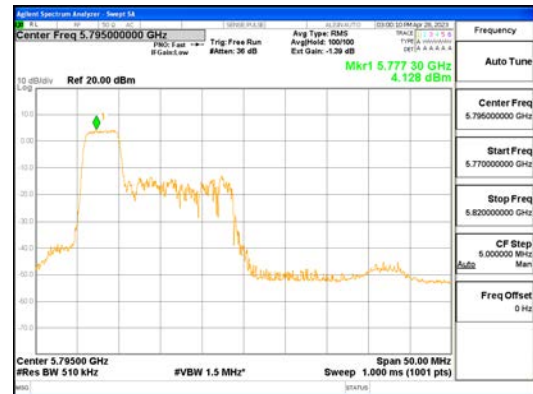
ANTO_802.11ax_HE40_52T_Low_UNII 3
