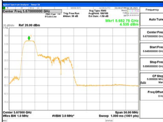
ANT1_802.11ax_HE40_52T_Low_UNII 2C
