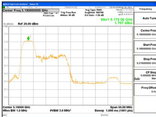
ANTO_802.11ax_HE40_52T_Low_UNII 1
