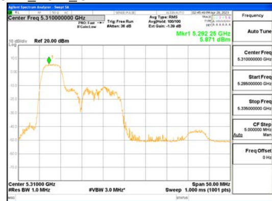
ANTO_802.11ax_HE40_52T_Low_UNII 2A
