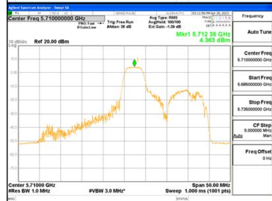
ANT0_802.11ax_HE40_52T_Mid_UNII 2C
