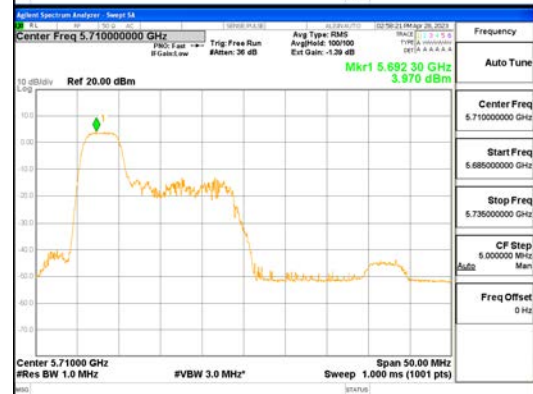
ANTO_802.11ax_HE40_52T_Low_UNII 2C
