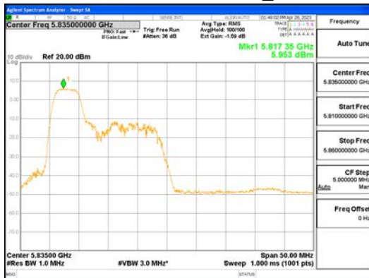
ANT1_802.11ax_HE40_52T_Low_UNII 4
