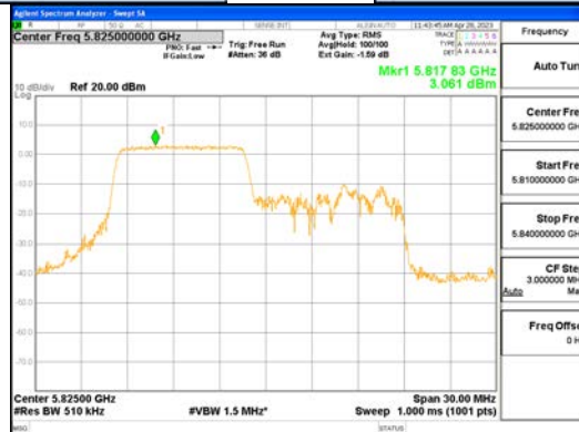
ANT1_802.11ax_HE20_106T_Low_UNII 3
