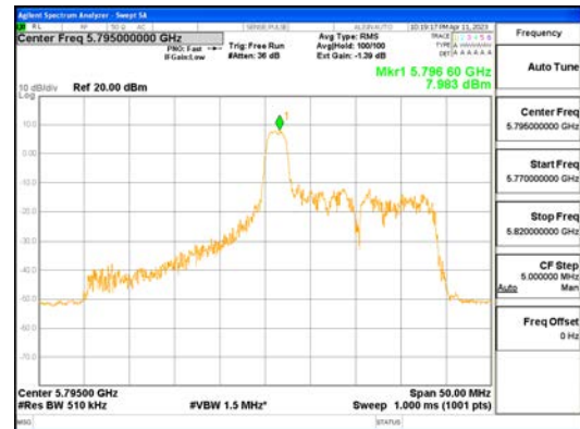
ANT0_802.11ax_HE40_26T_Mid_UNI1 3
