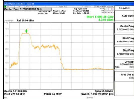
ANT1_802.11ax_HE40_52T_Low_UNII 2C
