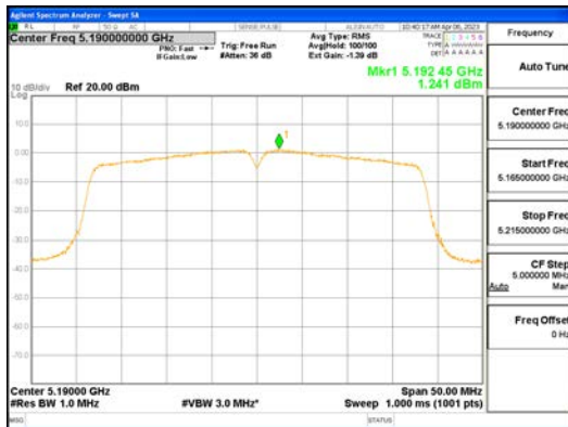
ANT0_802.11ac_VHT40_UNI1 1
