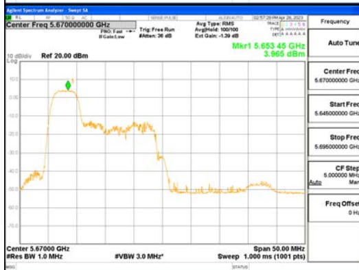
ANTO_802.11ax_HE40_52T_Low_UNII 2C
