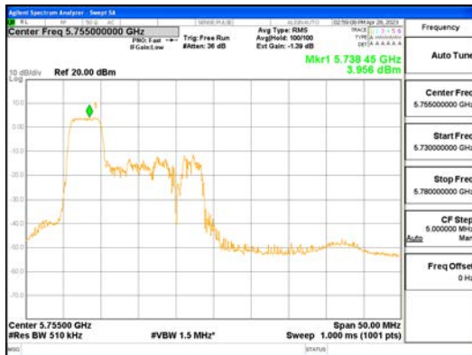
ANTO_802.11ax_HE40_52T_Low_UNII 3
