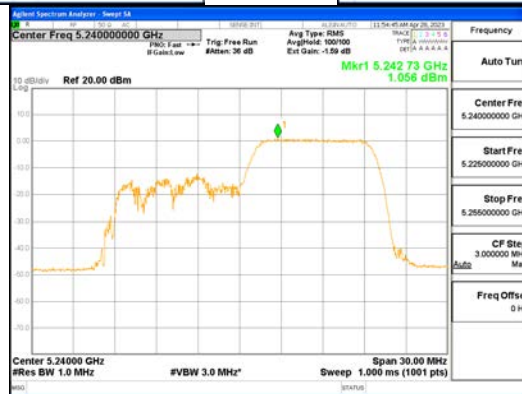
ANT1_802.11ax_HE20_106T_High_UNII 1
