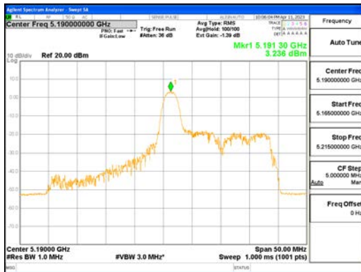
ANT0_802.11ax_HE40_26T_Mid_UNII 1
