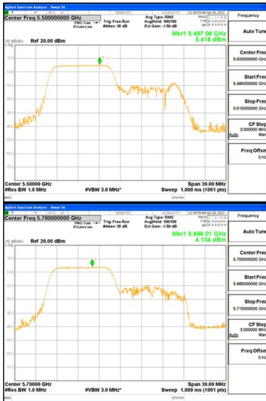
ANT1_802.11ax_HE20_106T_Low_UNII 2C
