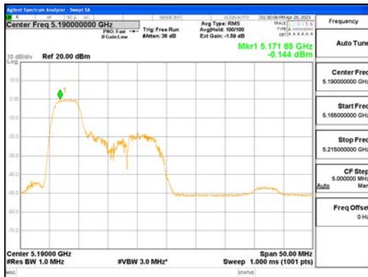
ANT1_802.11ax_HE40_52T_Low_UNII 1
