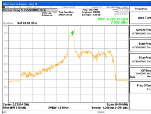
ANT0_802.11ax_HE40_26T_Mid_UNI1 3
