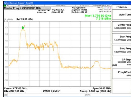
ANTO_802.11ax_HE40_26T_Low_UNII 3
