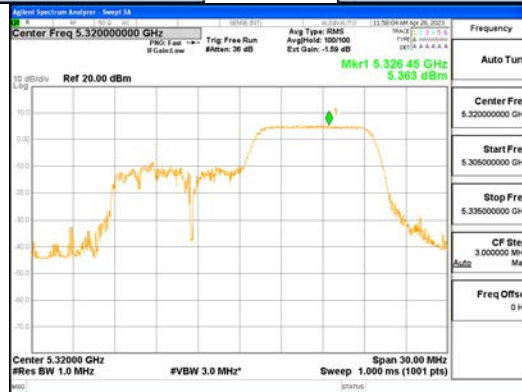
ANT1_802.11ax_HE20_106T_High_UNII 2A
