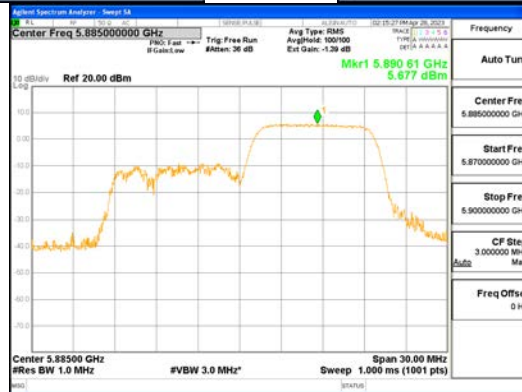
ANT0_802.11ax_HE20_106T_High_UNII 4
