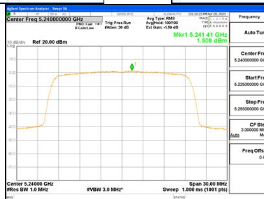
ANT1_802.11ax_HE20_242T_UNII 1
