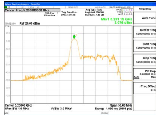
ANT1_802.11ax_HE40_26T_Mid_UNII 1
