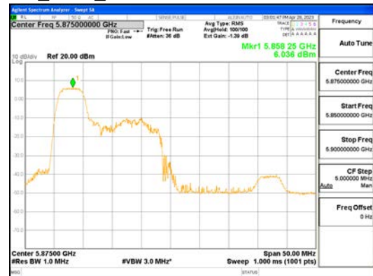
ANTO_802.11ax_HE40_52T_Low_UNII 4
