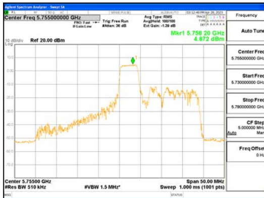
ANT0_802.11ax_HE40_52T_Mid_UNI1 3
