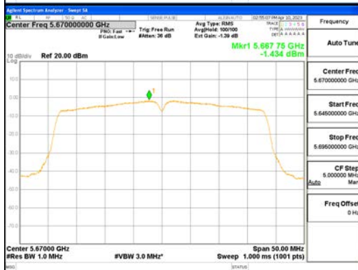
ANT0_802.11ac_VHT40_UNI1 2C
