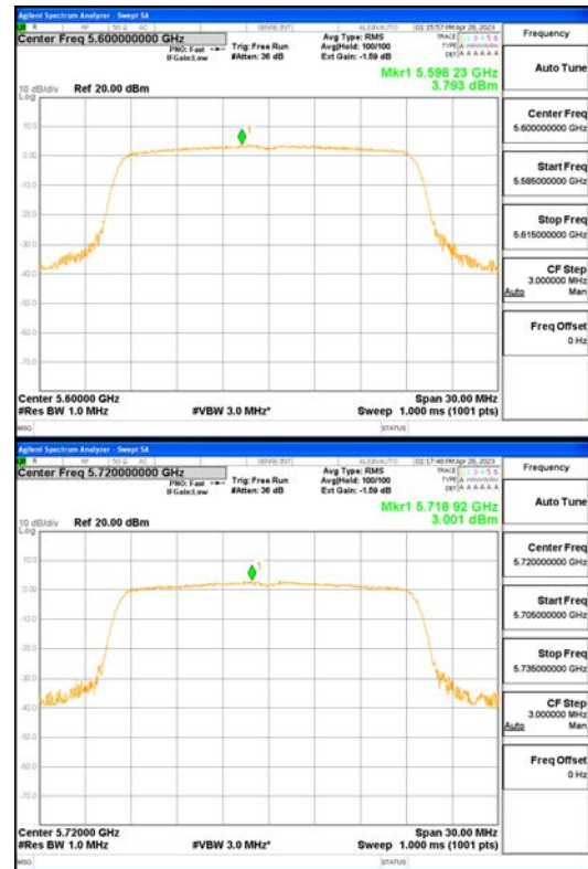
ANT1_802.11ax_HE20_242T_UNII 2C
