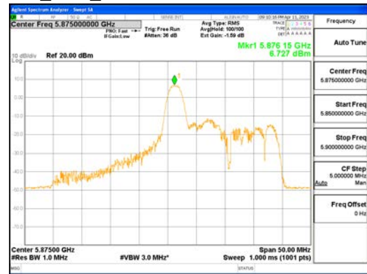
ANT1_802.11ax_HE40_26T_Mid_UNI1 4
