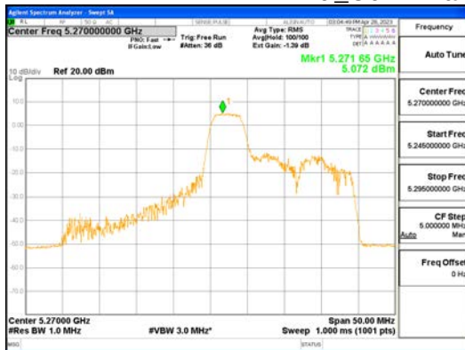
ANT0_802.11ax_HE40_52T_Mid_UNII 2A
