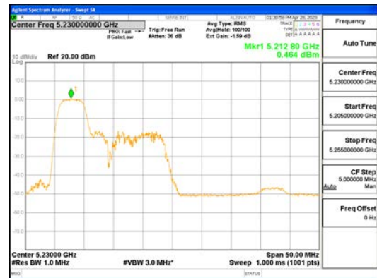
ANT1_802.11ax_HE40_52T_Low_UNII 1
