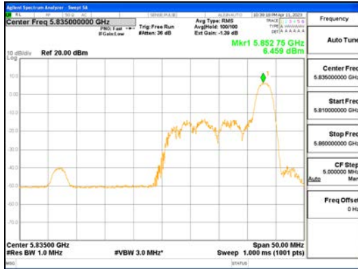
ANT0_802.11ax_HE40_26T_High_UNII 4
