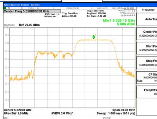
ANT0_802.11ax_HE20_106T_High_UNII 2A
