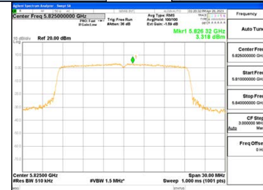
ANT1_802.11ax_HE20_242T_UNII 3
