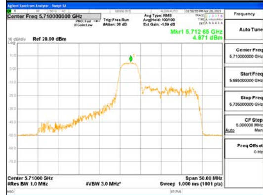
ANT1_802.11ax_HE40_52T_Mid_UNII 2C
