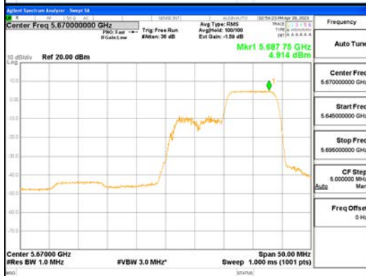
ANT1_802.11ax_HE40_106T_High_UNII 2C
