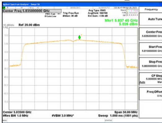
ANT1_802.11ax_HE40_484T_UNII 4
