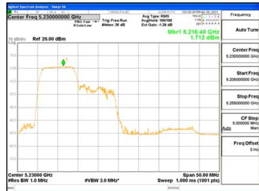
ANTO_802.11ax_HE40_106T_Low_UNII 1
