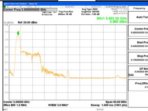
ANT1_802.11ax_HE80_26T_Low_UNII 2C
