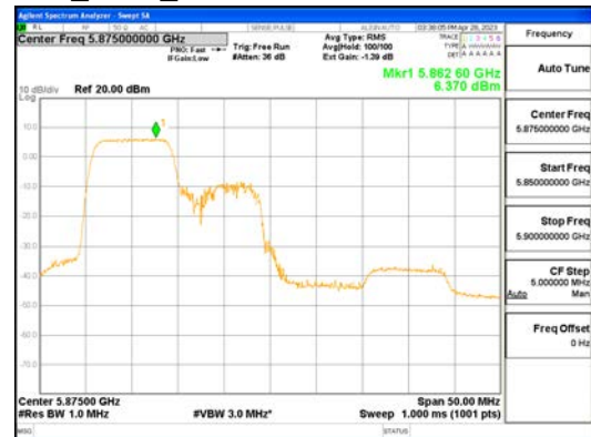
ANTO_802.11ax_HE40_106T_Low_UNII 4
