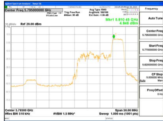
ANT0_802.11ax_HE40_52T_High_UNII 3
