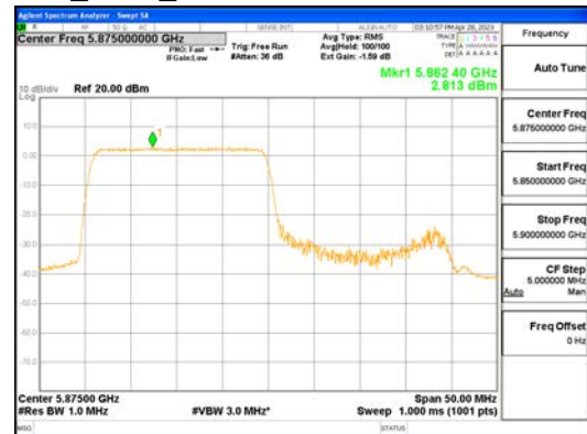
ANT1_802.11ax_HE40_242T_Low_UNII 4
