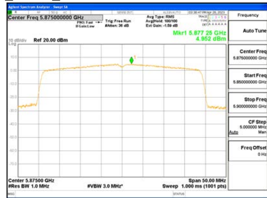
ANT1_802.11ax_HE40_484T_UNII 4
