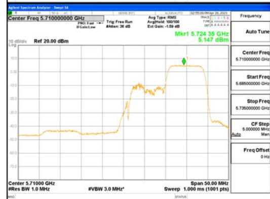
ANT1_802.11ax_HE40_106T_High_UNII 2C
