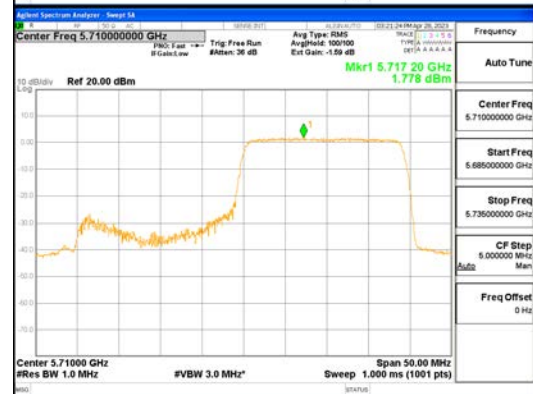
ANT1_802.11ax_HE40_242T_High_UNII 2C
