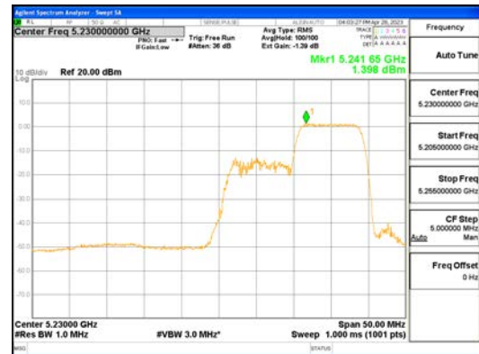
ANTO_802.11ax_HE40_106T_High_UNII 1
