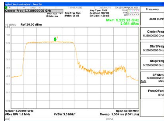
ANTO_802.11ax_HE40_242T_Low_UNII 1
