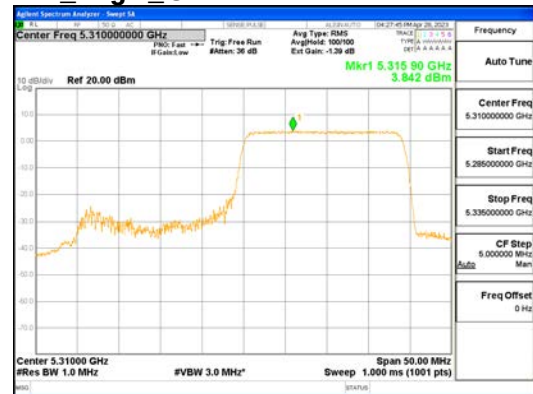
ANTO_802.11ax_HE40_242T_High_UNII 2A
