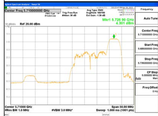
ANTO_802.11ax_HE40_52T_High_UNII 2C
