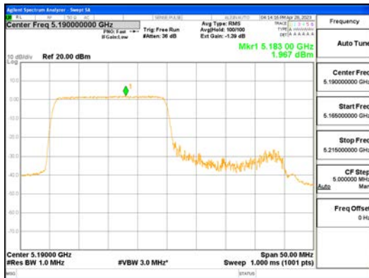
ANTO_802.11ax_HE40_242T_Low_UNII 1
