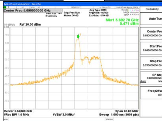
ANT1_802.11ax_HE80_26T_Mid_UNII 2C
