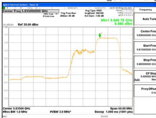
ANT1_802.11ax_HE40_106T_High_UNI I 4
