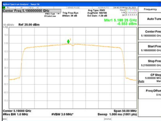
ANTO_802.11ax_HE40_484T_UNII 1
