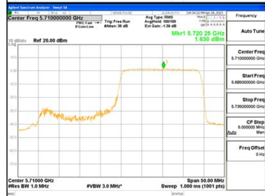
ANTO_802.11ax_HE40_242T_High_UNII 2C
