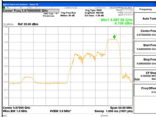
ANTO_802.11ax_HE40_52T_High_UNII 2C
