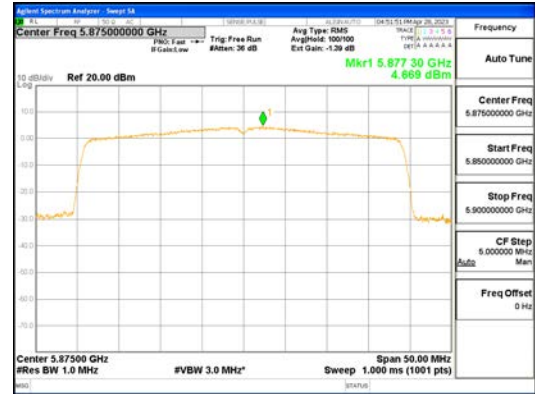
ANTO_802.11ax_HE40_484T_UNII 4
