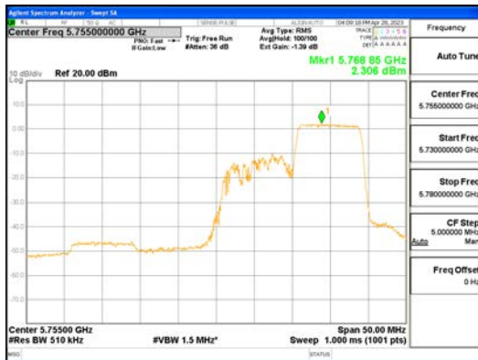
ANTO_802.11ax_HE40_106T_High_UNII 3
