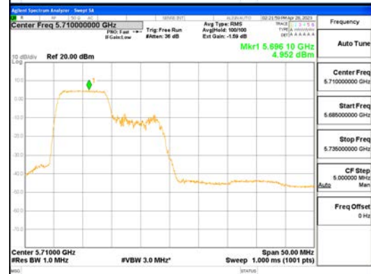
ANT1_802.11ax_HE40_106T_Low_UNII 2C
