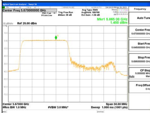
ANTO_802.11ax_HE40_242T_Low_UNII 2C
