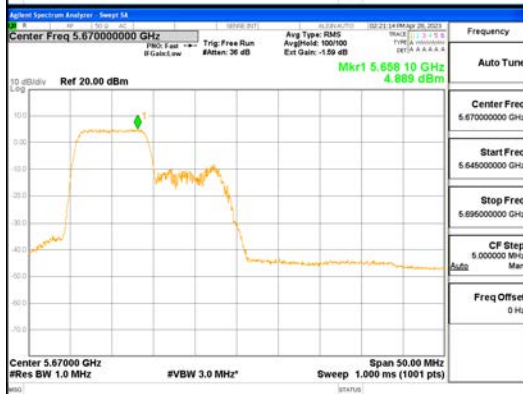
ANT1_802.11ax_HE40_106T_Low_UNII 2C
