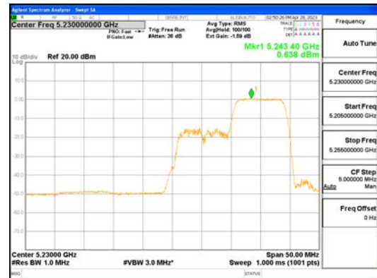
ANT1_802.11ax_HE40_106T_High_UNII 1
