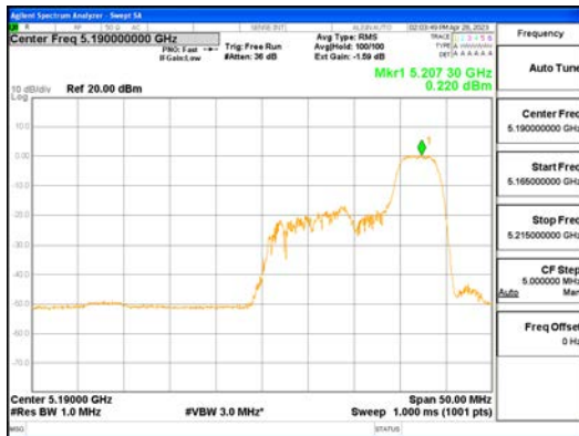
ANT1_802.11ax_HE40_52T_High_UNII 1
