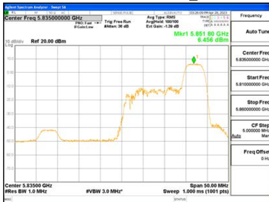
ANT0_802.11ax_HE40_52T_High_UNII 4
