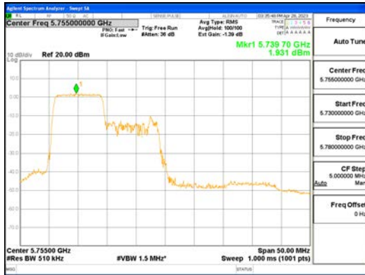
ANTO_802.11ax_HE40_106T_Low_UNII 3
