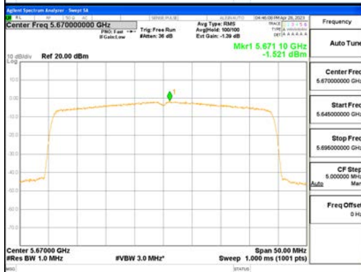
ANTO_802.11ax_HE40_484T_UNII 2C
