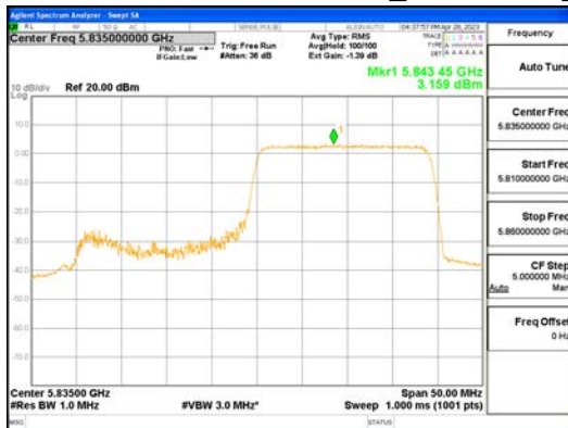
ANTO_802.11ax_HE40_242T_High_UNII 4
