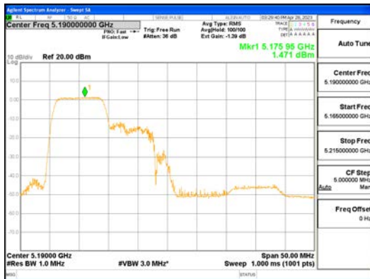
ANTO_802.11ax_HE40_106T_Low_UNII 1
