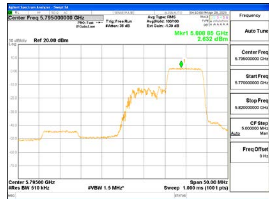
ANTO_802.11ax_HE40_106T_High_UNII 3
