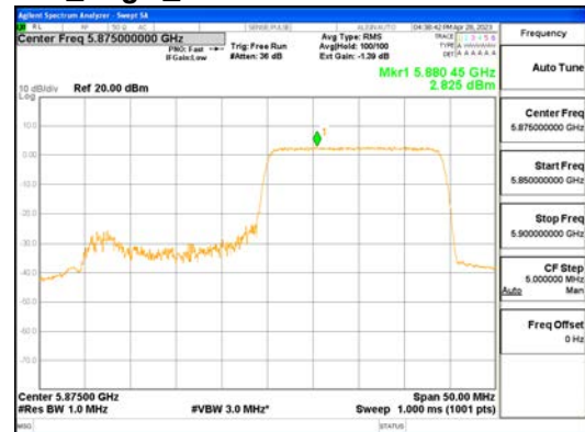
ANTO_802.11ax_HE40_242T_High_UNII 4
