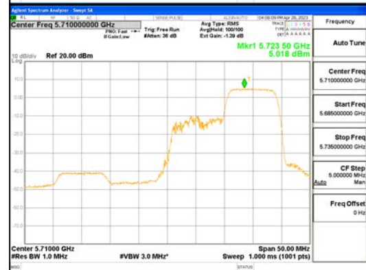
ANTO_802.11ax_HE40_106T_High_UNII 2C
