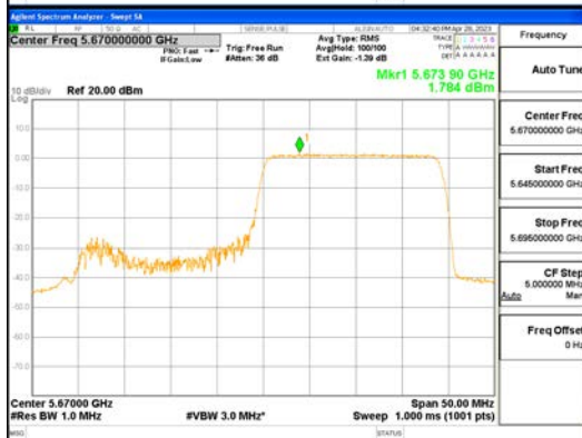
ANTO_802.11ax_HE40_242T_High_UNII 2C
