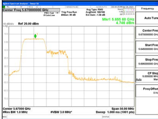
ANTO_802.11ax_HE40_106T_Low_UNII 2C
