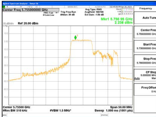
ANT1_802.11ax_HE40_106T_Mid_UNII 3
