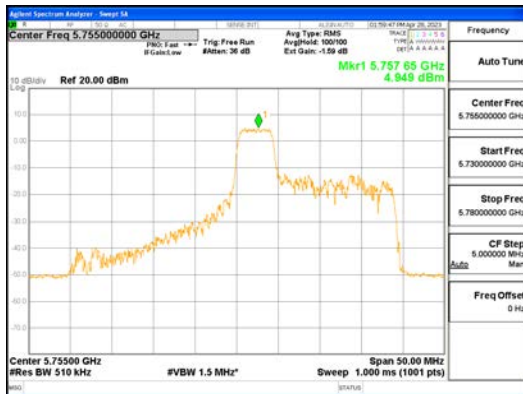
ANT1_802.11ax_HE40_52T_Mid_UNII 3
