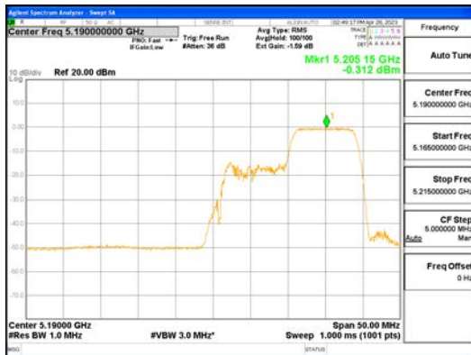
ANT1_802.11ax_HE40_106T_High_UNII 1
