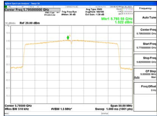
ANTO_802.11ax_HE40_484T_UNII 3
