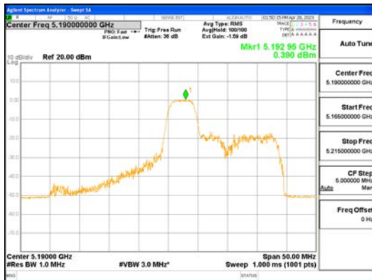
ANT1_802.11ax_HE40_52T_Mid_UNII 1
