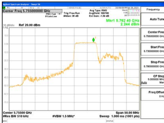
ANT0_802.11ax_HE40_106T_Mid_UNI1 3
