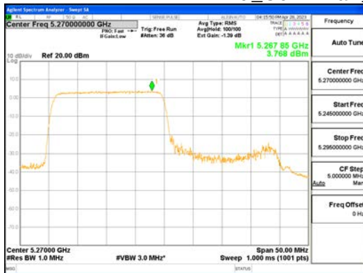
ANTO_802.11ax_HE40_242T_Low_UNII 2A
