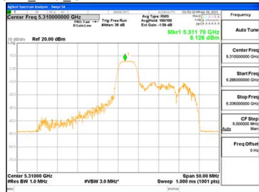
ANT1_802.11ax_HE40_52T_Mid_UNII 2A
