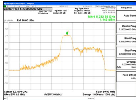
ANT1_802.11ax_HE40_52T_Mid_UNII 1
