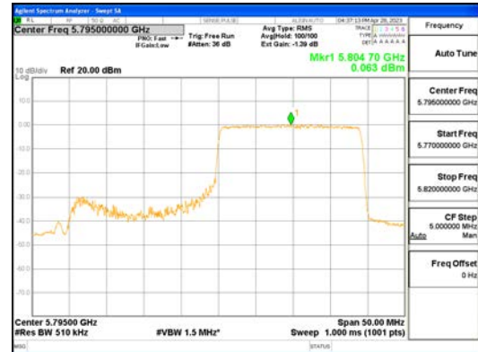
ANTO_802.11ax_HE40_242T_High_UNII 3
