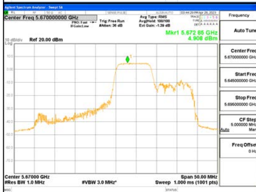
ANTO_802.11ax_HE40_106T_Mid_UNII 2C
