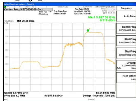
ANTO_802.11ax_HE40_106T_High_UNII 4
