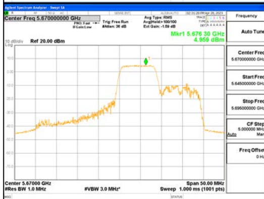
ANT1_802.11ax_HE40_106T_Mid_UNII 2C
