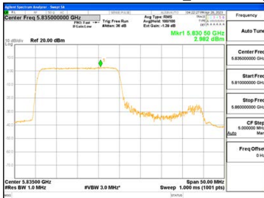
ANTO_802.11ax_HE40_242T_Low_UNII 4
