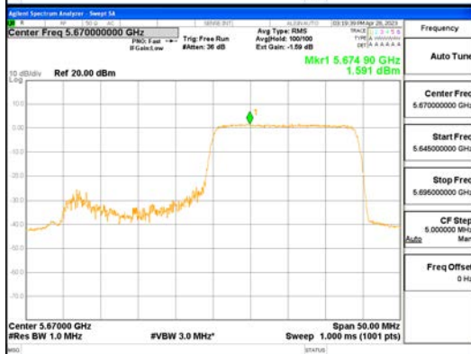
ANT1_802.11ax_HE40_242T_High_UNII 2C
