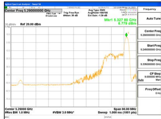
ANTO_802.11ax_HE80_26T_High_UNII 2A
