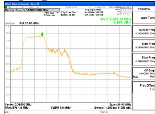
ANTO_802.11ax_HE40_106T_Low_UNII 2A
