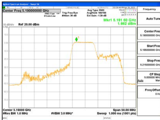
ANTO_802.11ax_HE40_106T_Mid_UNII 1
