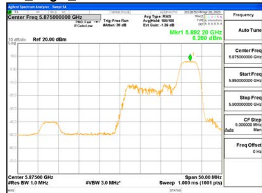
ANT0_802.11ax_HE40_52T_High_UNII 4
