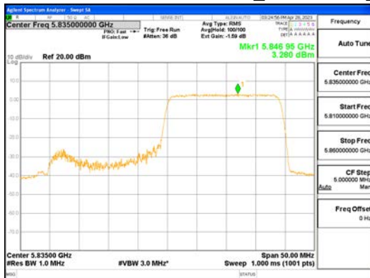
ANT1_802.11ax_HE40_242T_High_UNII 4
