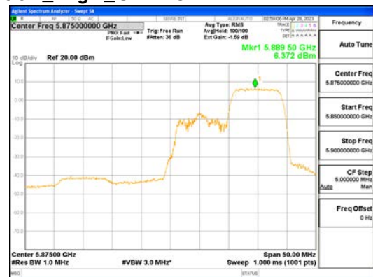
ANT1_802.11ax_HE40_106T_High_UNI I 4
