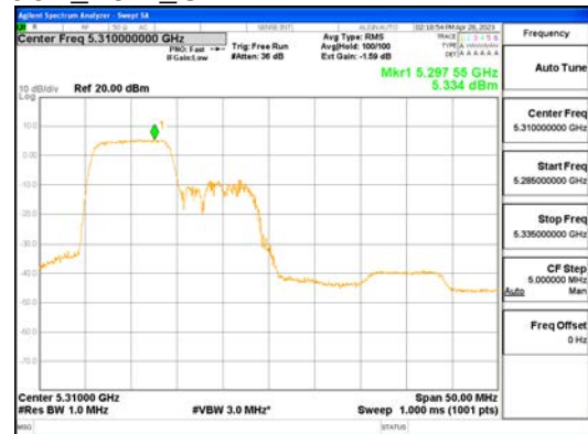
ANT1_802.11ax_HE40_106T_Low_UNII 2A
