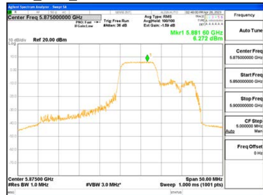
ANT1_802.11ax_HE40_106T_Mid_UNII 4
