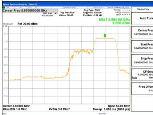
ANTO_802.11ax_HE40_106T_High_UNII 2C
