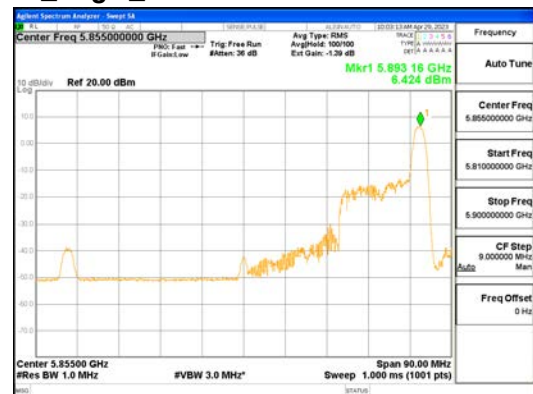
ANTO_802.11ax_HE80_26T_High_UNII 4
