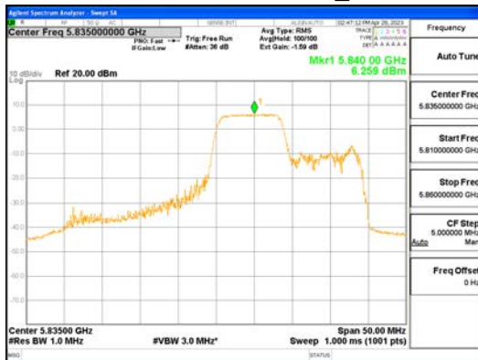
ANT1_802.11ax_HE40_106T_Mid_UNII 4
