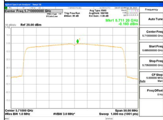
ANTO_802.11ax_HE40_484T_UNII 2C
