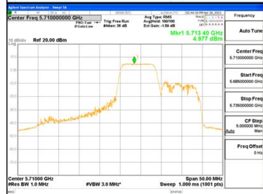
ANT1_802.11ax_HE40_106T_Mid_UNII 2C
