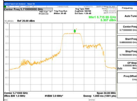
ANTO_802.11ax_HE40_106T_Mid_UNII 2C
