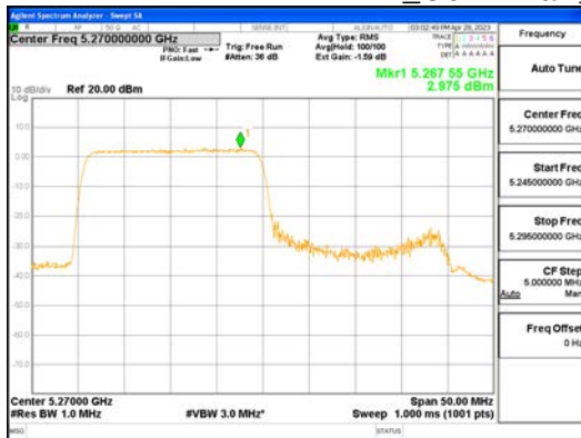
ANT1_802.11ax_HE40_242T_Low_UNII 2A
