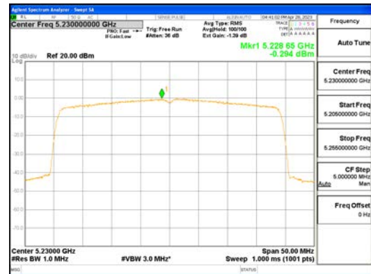
ANTO_802.11ax_HE40_484T_UNII 1
