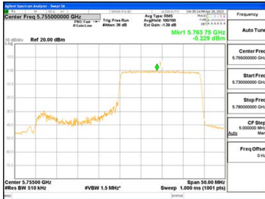
ANTO_802.11ax_HE40_242T_High_UNII 3
