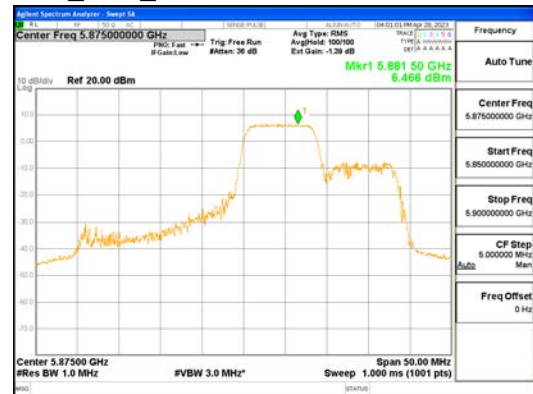
ANT0_802.11ax_HE40_106T_Mid_UNI1 4
