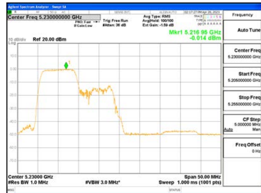
ANT1_802.11ax_HE40_106T_Low_UNII 1
