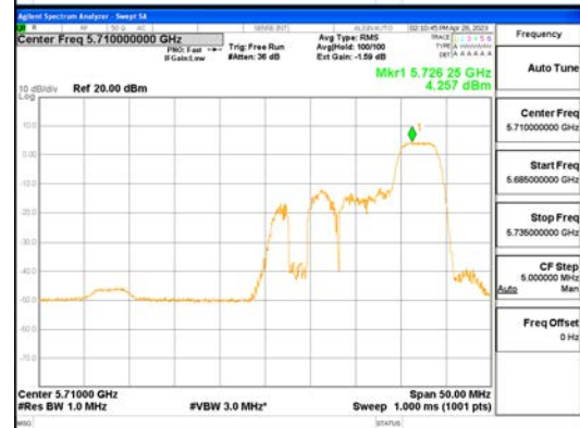
ANT1_802.11ax_HE40_52T_High_UNII 2C
