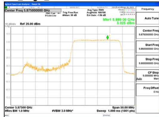
ANT1_802.11ax_HE40_242T_High_UNII 4
