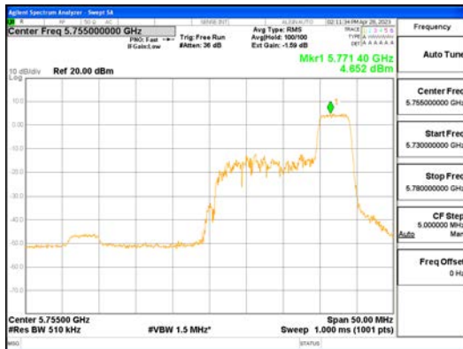
ANT1_802.11ax_HE40_52T_High_UNII 3
