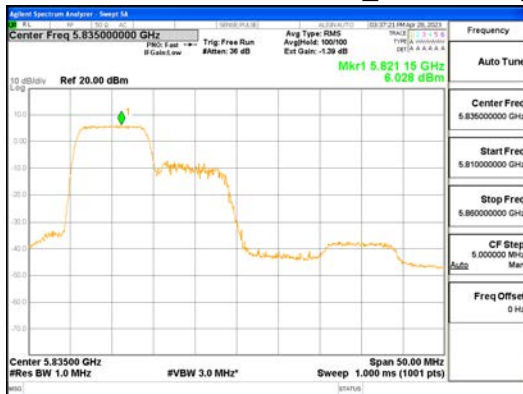
ANTO_802.11ax_HE40_106T_Low_UNII 4
