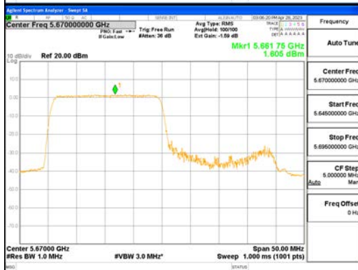
ANT1_802.11ax_HE40_242T_Low_UNII 2C
