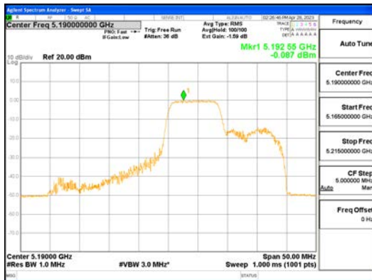
ANT1_802.11ax_HE40_106T_Mid_UNII 1
