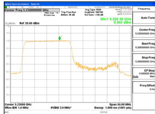
ANT1_802.11ax_HE40_242T_Low_UNII 1
