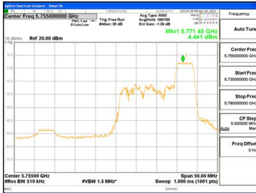
ANT0_802.11ax_HE40_52T_High_UNII 3
