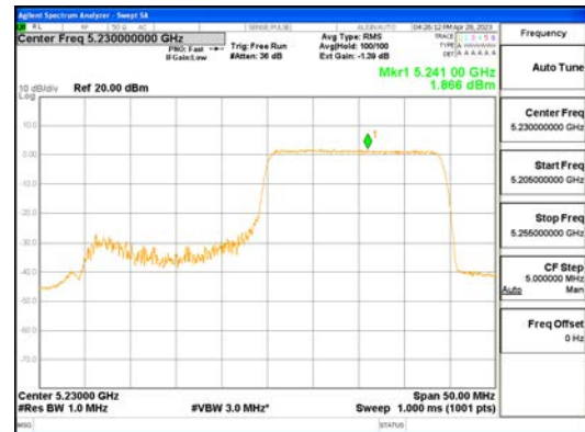
ANTO_802.11ax_HE40_242T_High_UNII 1
