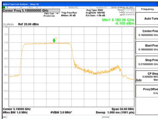
ANT1_802.11ax_HE40_242T_Low_UNII 1
