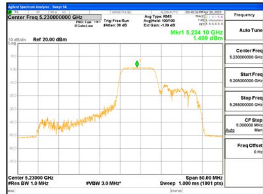
ANTO_802.11ax_HE40_106T_Mid_UNII 1
