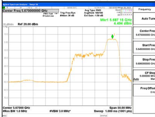
ANT1_802.11ax_HE40_52T_High_UNII 2C
