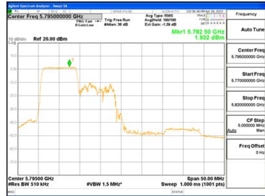
ANTO_802.11ax_HE40_106T_Low_UNII 3
