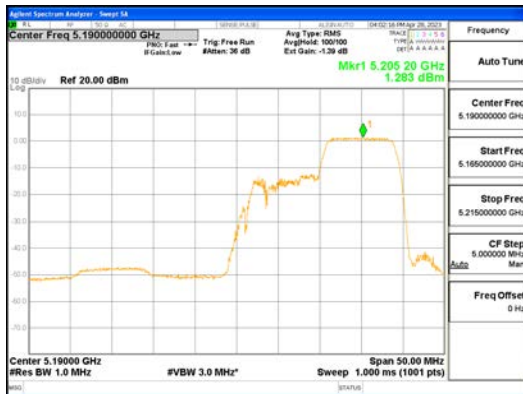
ANTO_802.11ax_HE40_106T_High_UNII 1
