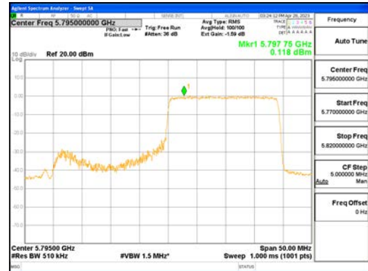
ANT1_802.11ax_HE40_242T_High_UNII 3
