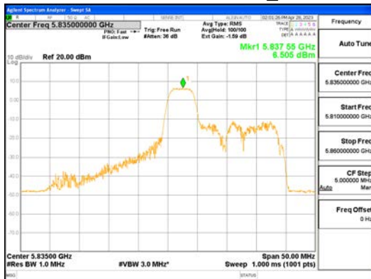
ANT1_802.11ax_HE40_52T_Mid_UNII 4
