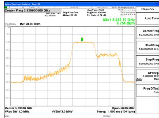
ANT1_802.11ax_HE40_106T_Mid_UNII 1
