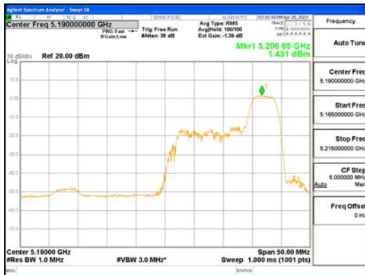
ANTO_802.11ax_HE40_52T_High_UNII 1
