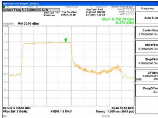
ANTO_802.11ax_HE40_242T_Low_UNII 3
