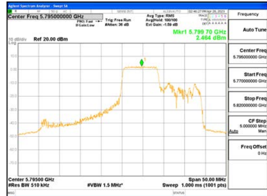
ANT1_802.11ax_HE40_106T_Mid_UNII 3
