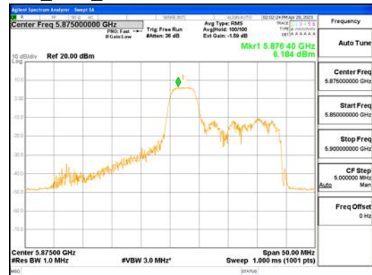
ANT1_802.11ax_HE40_52T_Mid_UNII 4
