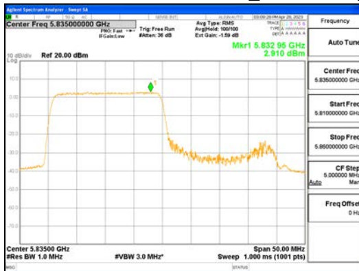
ANT1_802.11ax_HE40_242T_Low_UNII 4
