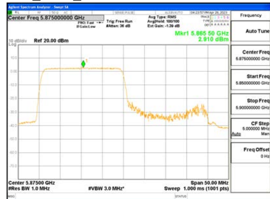
ANTO_802.11ax_HE40_242T_Low_UNII 4
