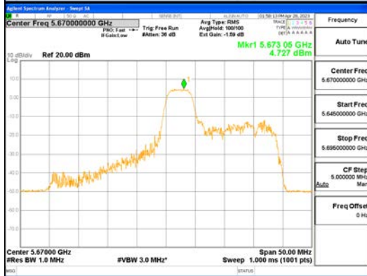
ANT1_802.11ax_HE40_52T_Mid_UNII 2C
