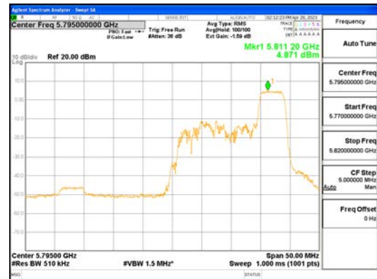
ANT1_802.11ax_HE40_52T_High_UNII 3
