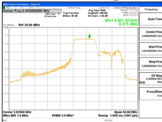
ANT0_802.11ax_HE40_106T_Mid_UNI1 4
