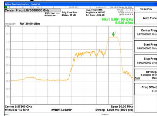
ANT1_802.11ax_HE40_52T_High_UNII 4
