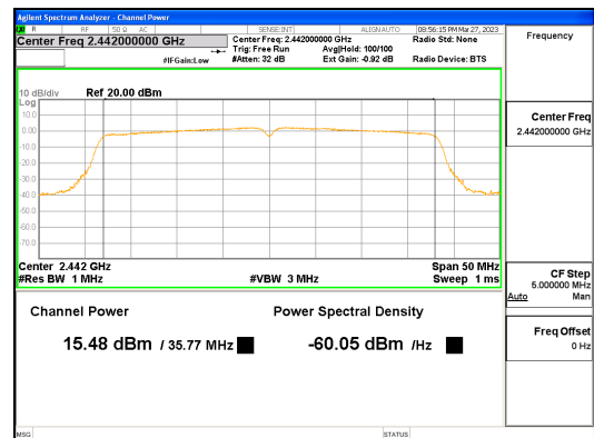
ANT0, 802.11n_HT40
