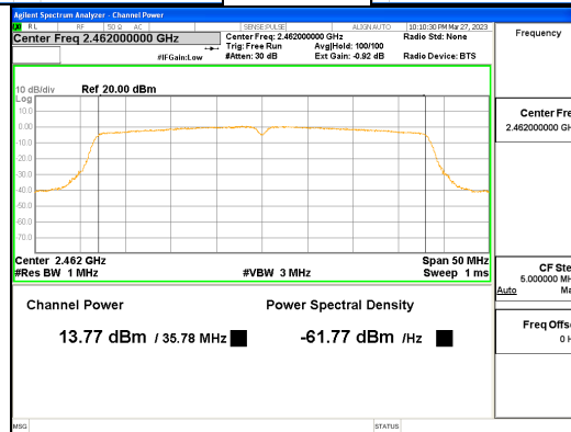
ANT0, 802.11n_HT40
