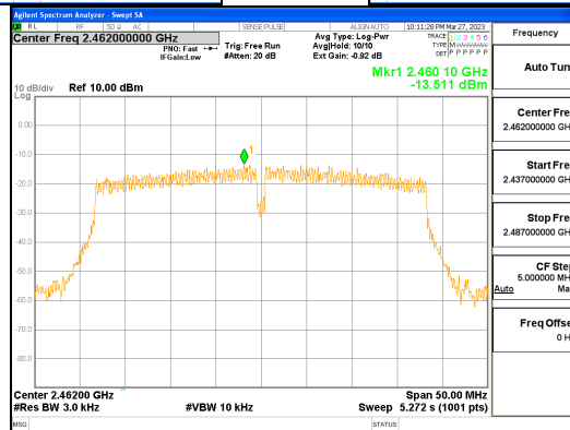
ANT0, 802.11n_HT40
