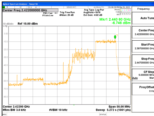
ANT0, 802.11ax_HE40_106T_High
