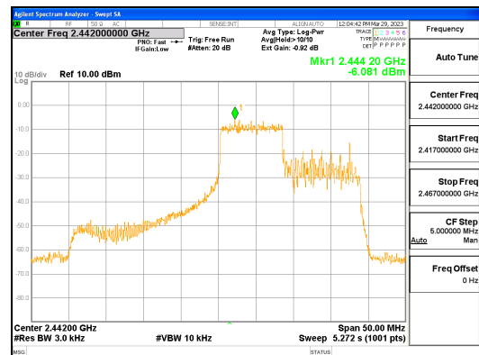
ANT0, 802.11ax_HE40_106T_Mid
