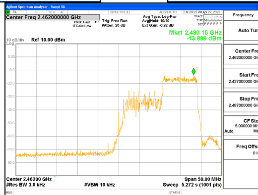
ANT0, 802.11ax_HE40_106T_High
