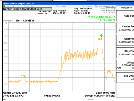
ANT0, 802.11ax_HE40_26T_High
