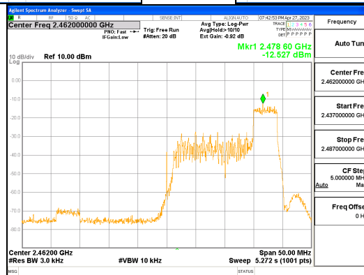
ANT1, 802.11ax_HE40_52T_High
