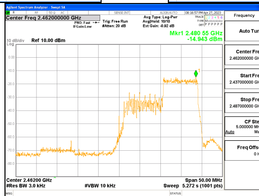
ANT1, 802.11ax_HE40_106T_High
