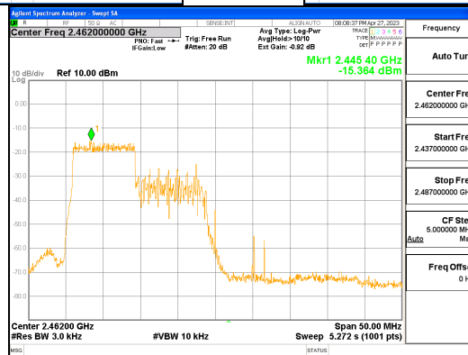
ANT1, 802.11ax_HE40_106T_Low
