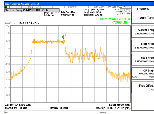
ANT0, 802.11ax_HE20_106T_Low
