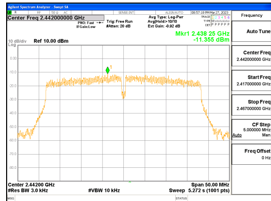
ANT0, 802.11n_HT40
