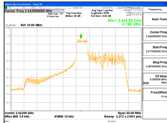
ANT0, 802.11ax_HE40_52T_Mid
