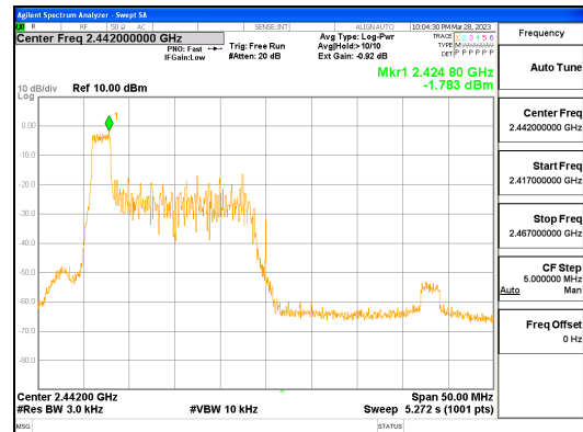
ANT0, 802.11ax_HE40_26T_Low
