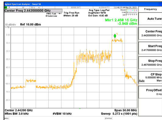
ANT0, 802.11ax_HE40_52T_High
