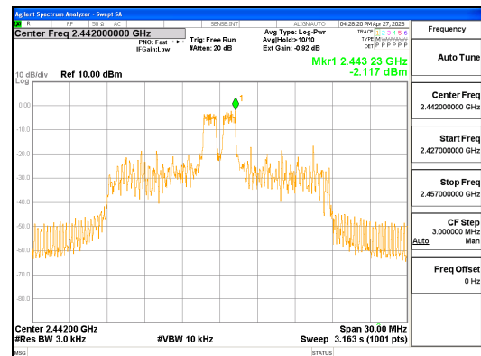
ANT0, 802.11ax_HE20_26T_Mid
