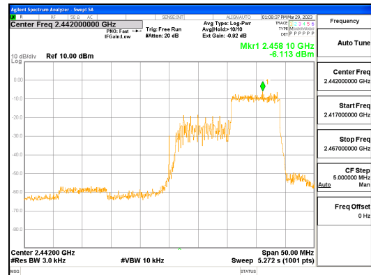
ANT0, 802.11ax_HE40_106T_High
