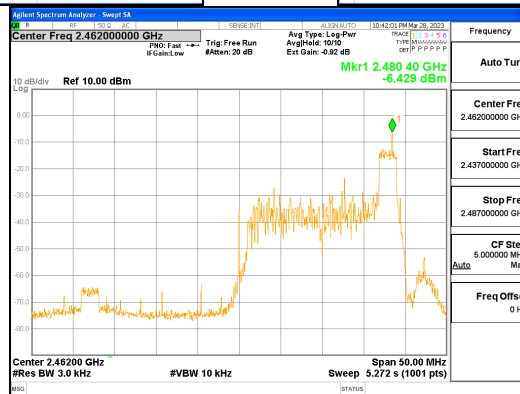
ANT1, 802.11ax_HE40_26T_High
