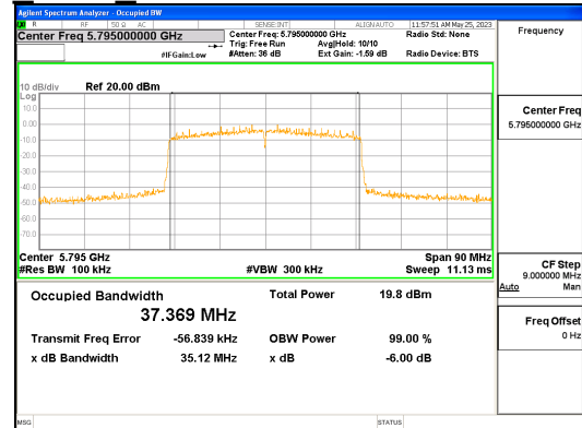
ANT R 802.11ax HE40_484T UNII 3
