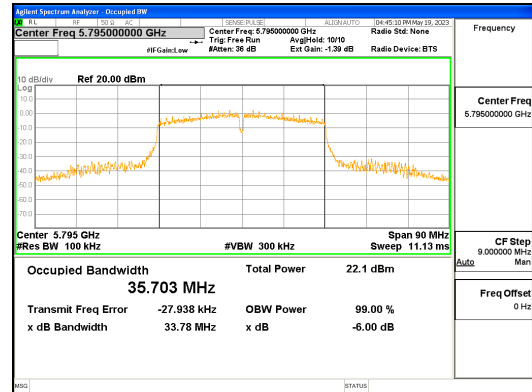
ANT L_802.11n_HT40_UNII 3
