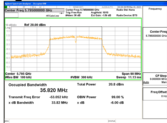
ANT R_802.11n_HT40_UNII 3
