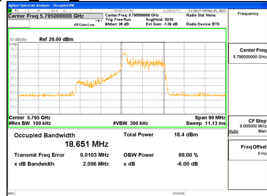
ANT L 802.11ax_HE40_26T_Mid_UNII 3
