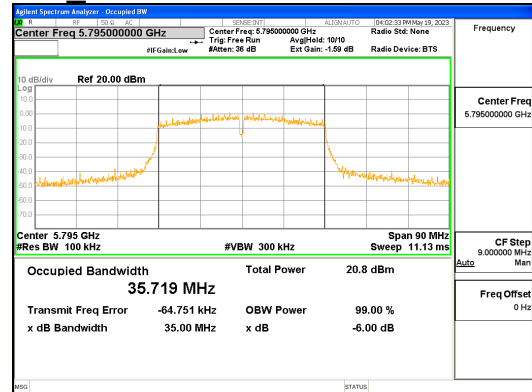
ANT R_802.11ac_VHT40_UNII 3
