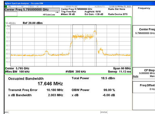
ANT L 802.11ax HE40_26T High_UNII 3
