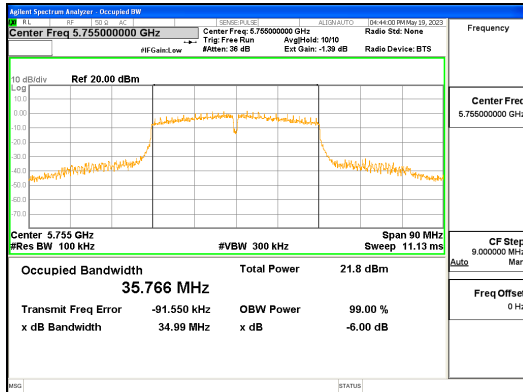
ANT L_802.11n_HT40_UNII 3
