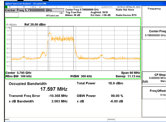
ANT R 802.11ax_HE40_26T_Low_UNII 3
