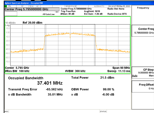
ANT L 802.11ax HE40_484T UNII 3
