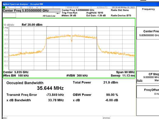
ANT L_802.11ac_VHT40_UNII 4
