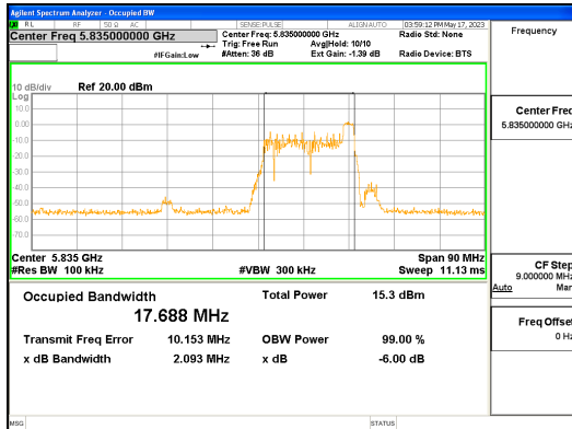
ANT L_802.11ax_HE40_26T_High_UNII 4
