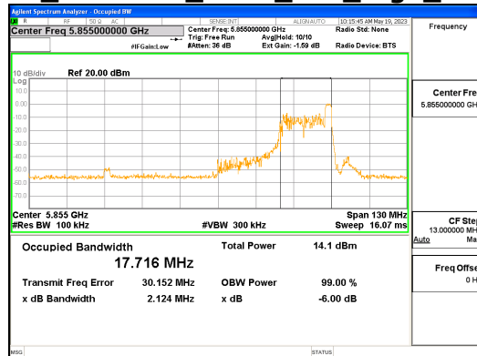
ANT R_802.11ax_HE80_26T_High_UNII 4
