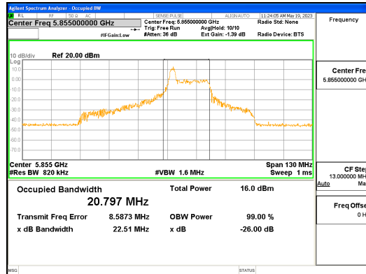
ANT L_802.11ax_HE80_26T_Mid_UNII 4
