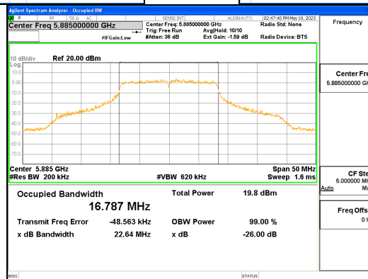
ANT R_802.11a_UNII 4
