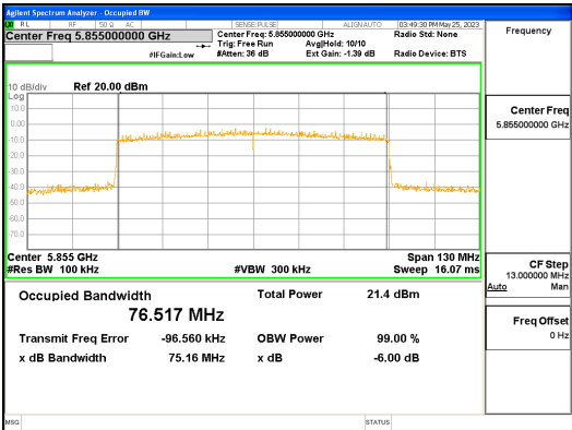
ANT L_802.11ax_HE80_996T_UNII 4
