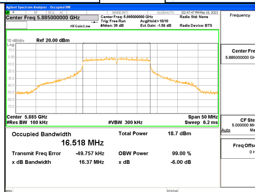
ANT R_802.11a_UNII 4
