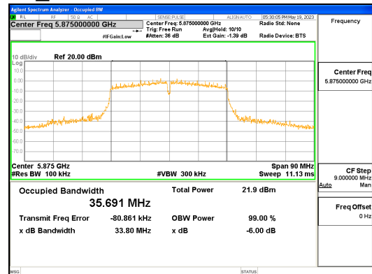
ANT L_802.11ac_VHT40_UNII 4
