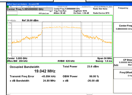
ANT L_802.11ax_HE20_242T_UNII 4
