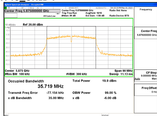
ANT R_802.11ac_VHT40_UNII 4
