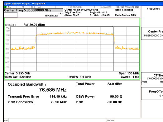
ANT L_802.11ax_HE80_996T_UNII 4
