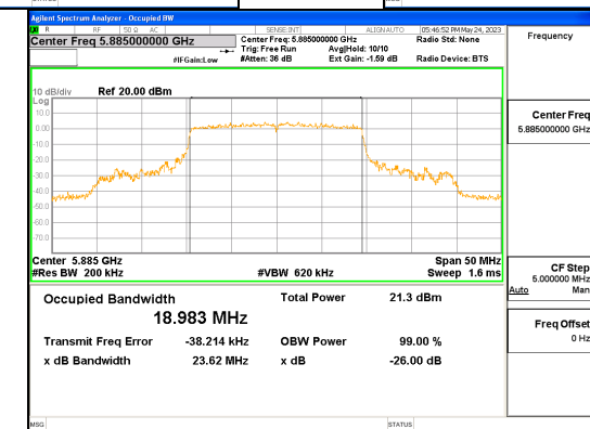
ANT R_802.11ax_HE20_242T_UNII 4
