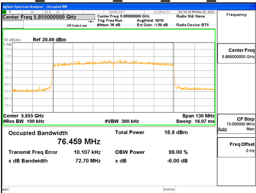
ANT R_802.11ax_HE80_996T_UNII 4
