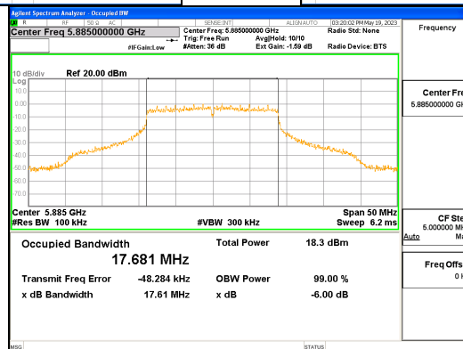
ANT R_802.11ac_VHT20_UNII 4
