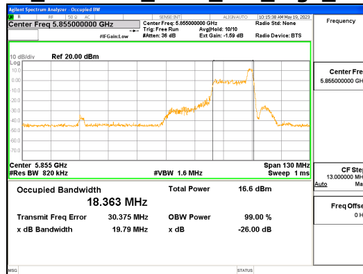
ANT R_802.11ax_HE80_26T_High_UNII 4
