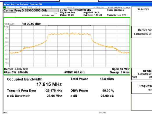
ANT R_802.11ac_VHT20_UNII 4
