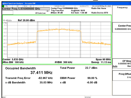
ANT L_802.11ax_HE40_484T_UNII 4
