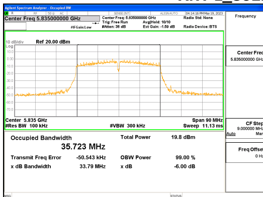
ANT R_802.11ac_VHT40_UNII 4
