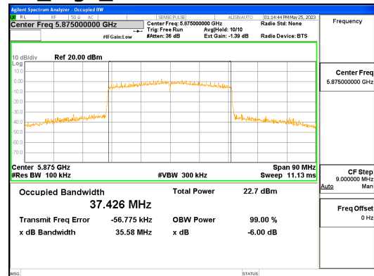
ANT L_802.11ax_HE40_484T_UNII 4
