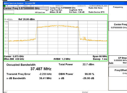
ANT R_802.11ax_HE40_484T_UNII 4
