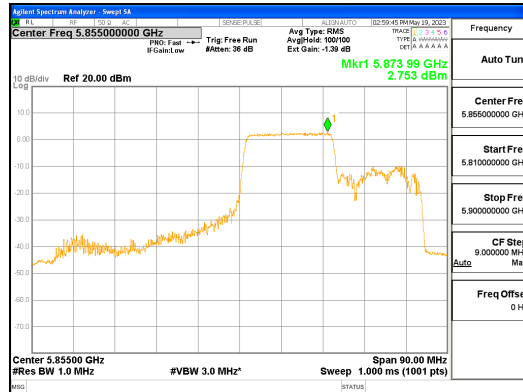
ANT L_802.11ax_HE80_242T_High_UNII 4
