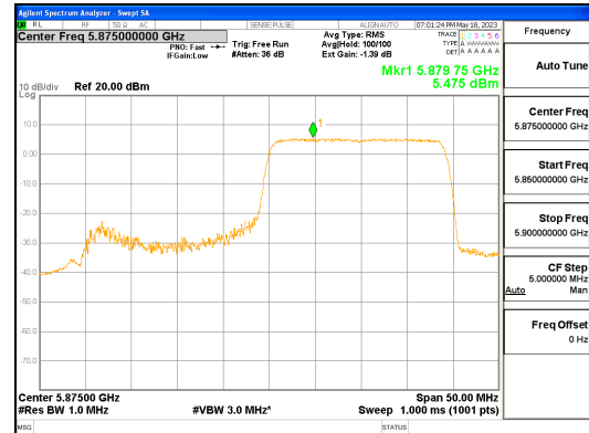
ANT L_802.11ax_HE40_242T_High_UNII 4
