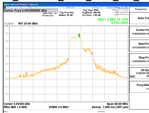
ANT R_802.11ax_HE80_106T_Mid_UNII 4
