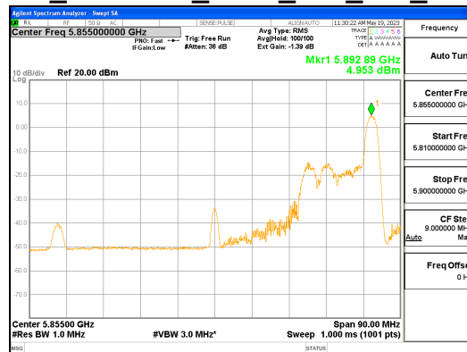
ANT L_802.11ax_HE80_26T_High_UNII 4
