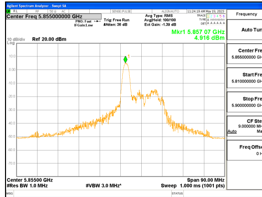
ANT L_802.11ax_HE80_26T_Mid_UNII 4
