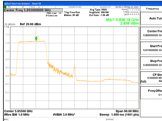
ANT L_802.11ax_HE80_242T_Low_UNII 4
