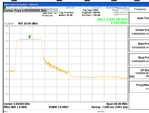
ANT R_802.11ax_HE80_242T_Low_UNII 4
