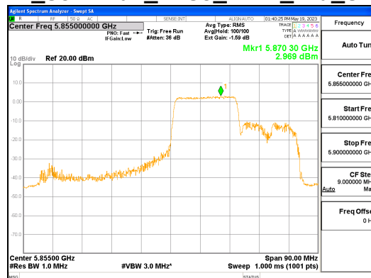
ANT R_802.11ax_HE80_242T_Mid_UNII 4
