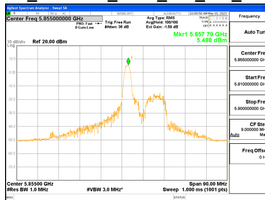
ANT R_802.11ax_HE80_26T_Mid_UNII 4
