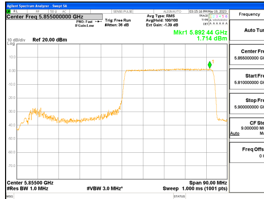
ANT L_802.11ax_HE80_484T_High_UNII 4
