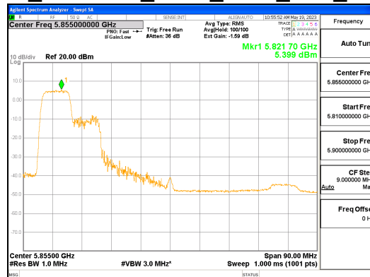
ANT R_802.11ax_HE80_106T_Low_UNII 4
