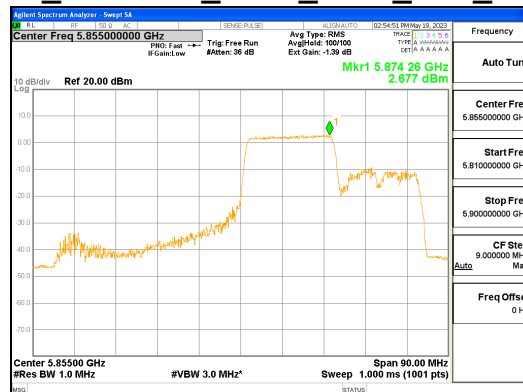
ANT L_802.11ax_HE80_242T_Mid_UNII 4
