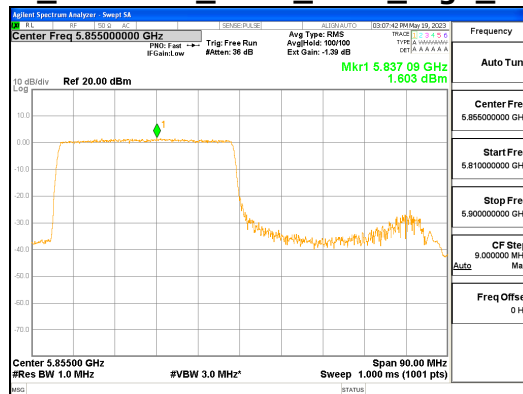
ANT L_802.11ax_HE80_484T_Low_UNII 4
