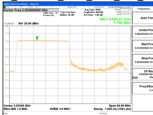
ANT R_802.11ax_HE80_484T_Low_UNII 4
