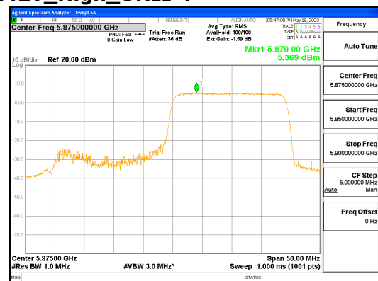
ANT R_802.11ax_HE40_242T_High_UNII 4
