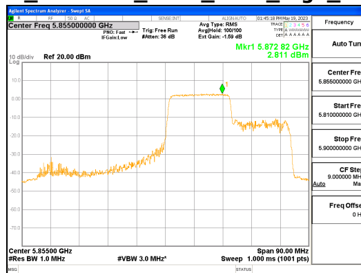
ANT R_802.11ax_HE80_242T_High_UNII 4
