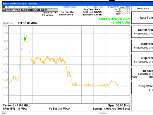
ANT L_802.11ax_HE40_26T_Low_UNII 6
