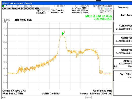
ANT R_802.11ax_HE40_26T_Mid_UNII 6
