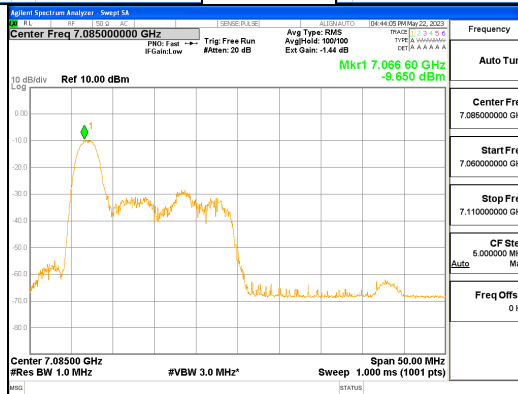
ANT L_802.11ax_HE40_26T_Low_UNII 8
