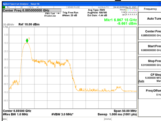
ANT L_802.11ax_HE40_26T_Low_UNII 7
