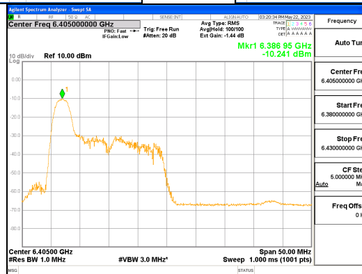
ANT R_802.11ax_HE40_26T_Low_UNII 5
