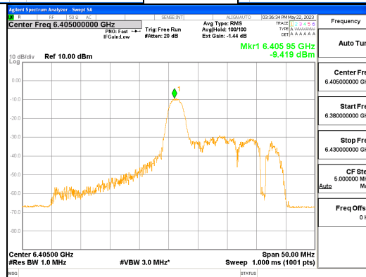
ANT R_802.11ax_HE40_26T_Mid_UNII 5
