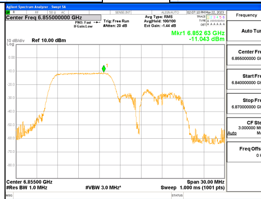
ANT R_802.11ax_HE20_106T_Low_UNII 7
