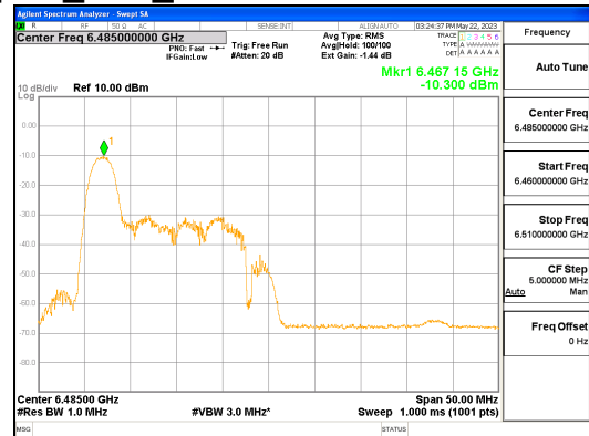
ANT R_802.11ax_HE40_26T_Low_UNII 6
