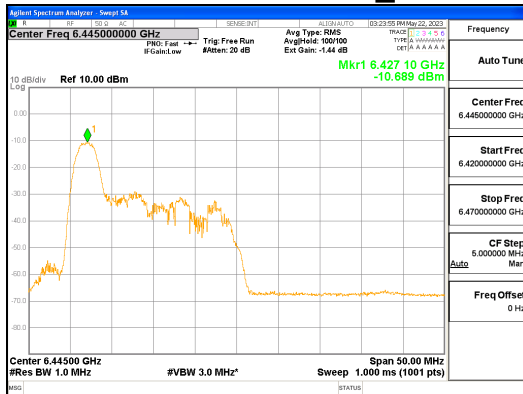
ANT R_802.11ax_HE40_26T_Low_UNII 6
