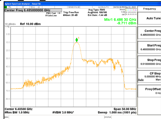
ANT L_802.11ax_HE40_26T_Mid_UNII 6
