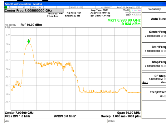
ANT L_802.11ax_HE40_26T_Low_UNII 7
