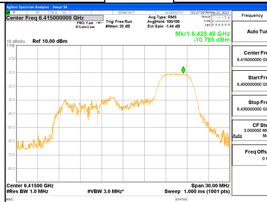
ANT R_802.11ax_HE20_52T_High_UNII 5
