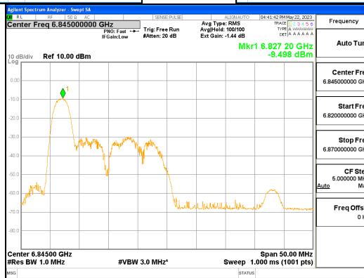
ANT L_802.11ax_HE40_26T_Low_UNII 7
