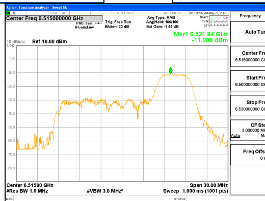
ANT R_802.11ax_HE20_52T_High_UNII 6
