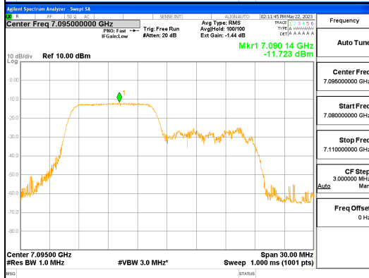
ANT R_802.11ax_HE20_106T_Low_UNII 8
