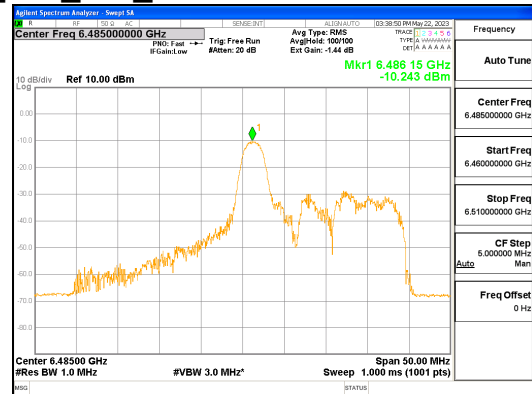
ANT R_802.11ax_HE40_26T_Mid_UNII 6
