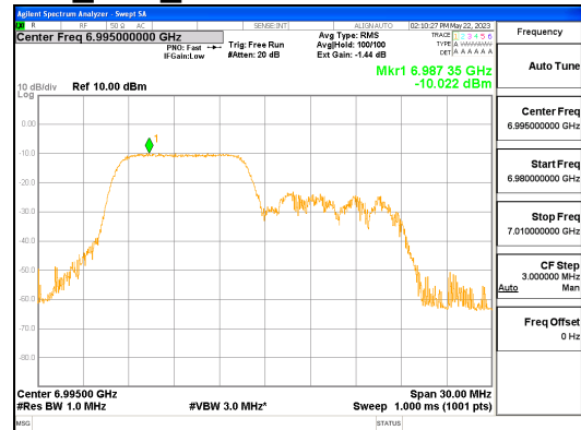
ANT R_802.11ax_HE20_106T_Low_UNII 7
