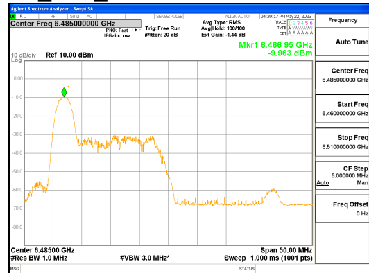
ANT L_802.11ax_HE40_26T_Low_UNII 6
