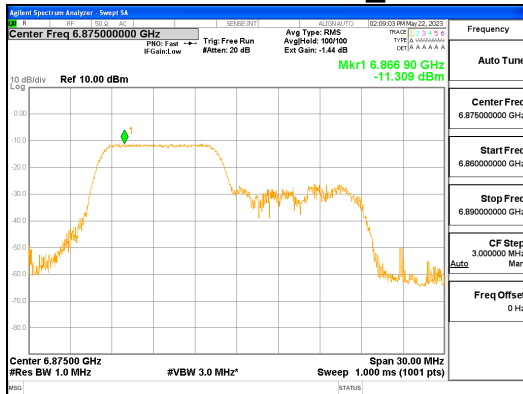
ANT R_802.11ax_HE20_106T_Low_UNII 7
