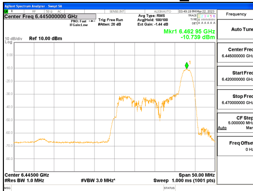
ANT R_802.11ax_HE40_26T_High_UNII 6
