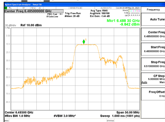
ANT L_802.11ax_HE40_106T_Mid_UNII 6
