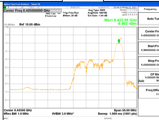
ANT R_802.11ax_HE40_26T_High_UNII 5
