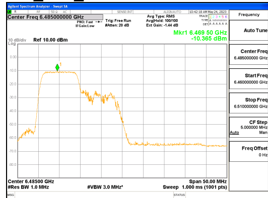
ANT R_802.11ax_HE40_106T_Low_UNII 6
