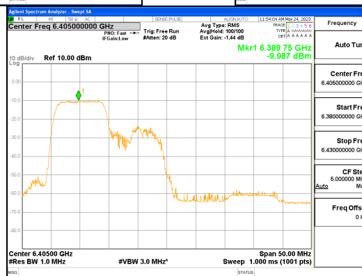
ANT L_802.11ax_HE40_106T_Low_UNII 5
