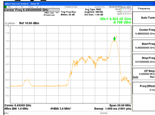
ANT L_802.11ax_HE40_26T_High_UNII 6
