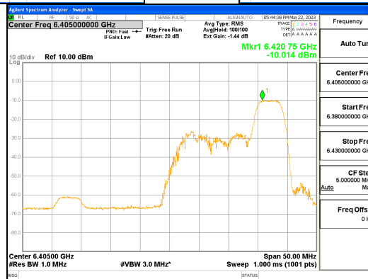
ANT L_802.11ax_HE40_52T_High_UNII 5
