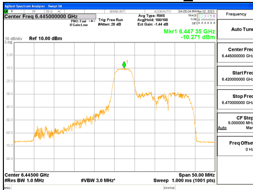
ANT_R_802.11ax_HE40_52T_Mid_UNII 6
