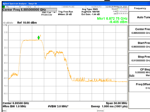
ANT L_802.11ax_HE40_106T_Low_UNII 7
