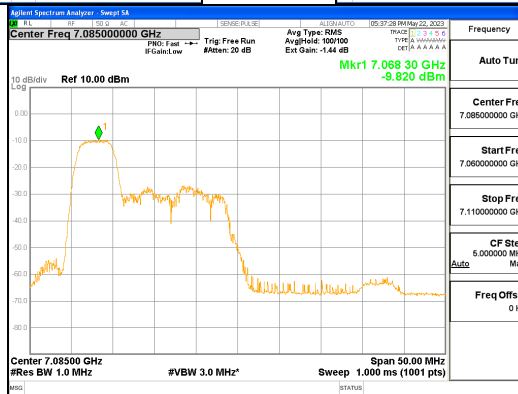
ANT L_802.11ax_HE40_52T_Low_UNII 8
