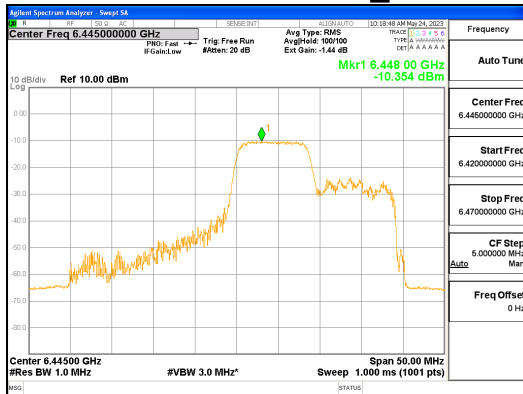
ANT R_802.11ax_HE40_106T_Mid_UNII 6
