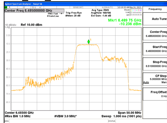
ANT R_802.11ax_HE40_106T_Mid_UNII 6
