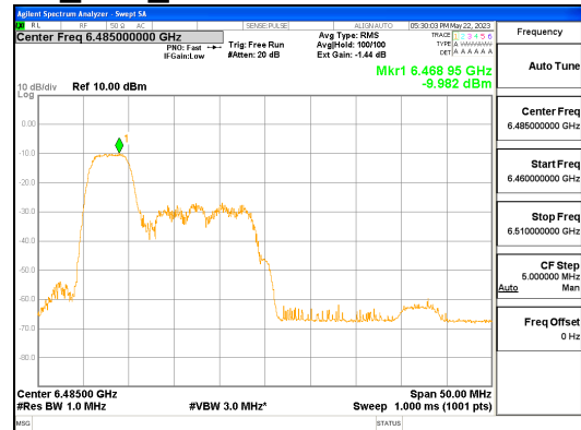
ANT L_802.11ax_HE40_52T_Low_UNII 6
