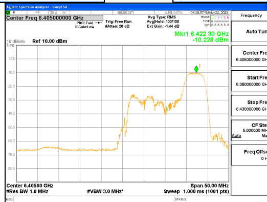
ANT R_802.11ax_HE40_52T_High_UNII 5
