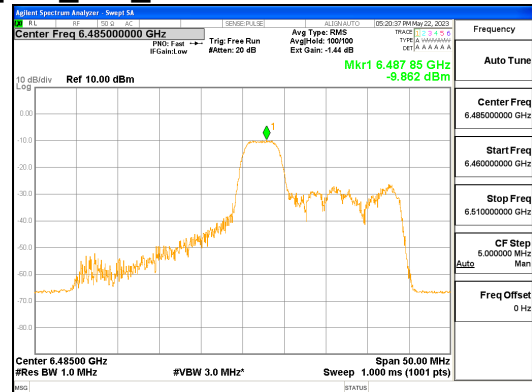
ANT L_802.11ax_HE40_52T_Mid_UNII 6
