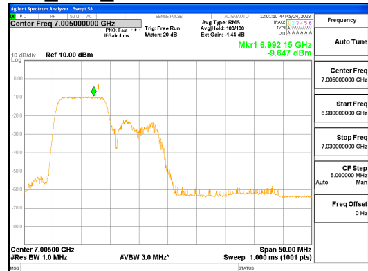
ANT L_802.11ax_HE40_106T_Low_UNII 7
