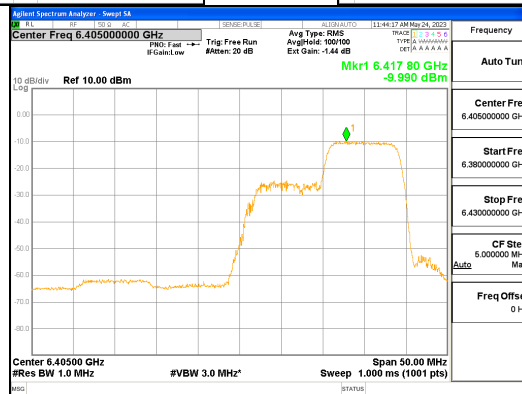
ANT L_802.11ax_HE40_106T_High_UNII 5
