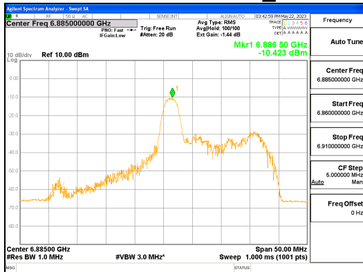
ANT R_802.11ax_HE40_26T_Mid_UNII 7
