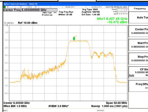
ANT R_802.11ax_HE40_106T_Mid_UNII 5
