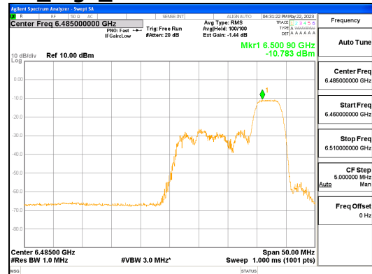
ANT R_802.11ax_HE40_52T_High_UNII 6
