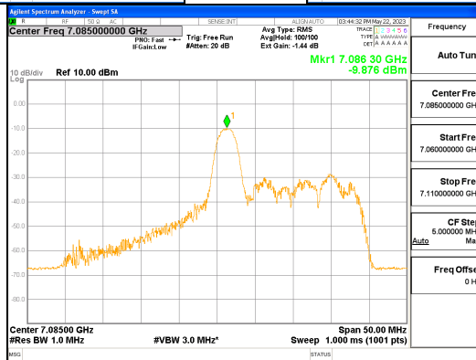
ANT R_802.11ax_HE40_26T_Mid_UNII 8
