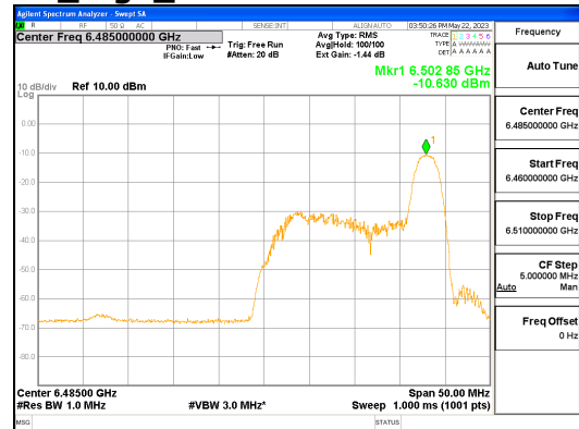
ANT R_802.11ax_HE40_26T_High_UNII 6
