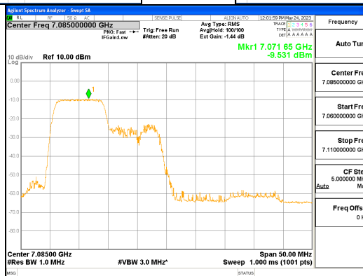
ANT L_802.11ax_HE40_106T_Low_UNII 8
