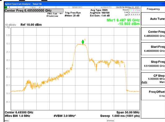
ANT_R_802.11ax_HE40_52T_Mid_UNII 6
