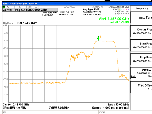
ANT L_802.11ax_HE40_106T_High_UNII 6
