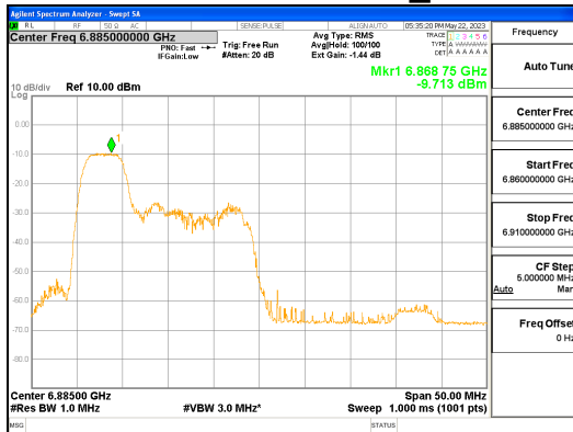
ANT L_802.11ax_HE40_52T_Low_UNII 7
