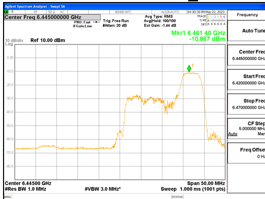
ANT R_802.11ax_HE40_52T_High_UNII 6
