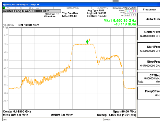
ANT L_802.11ax_HE40_106T_Mid_UNII 6
