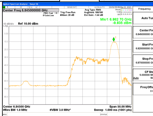
ANT R_802.11ax_HE40_26T_High_UNII 7
