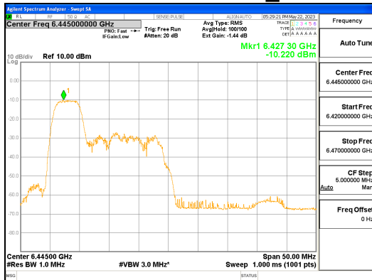
ANT L_802.11ax_HE40_52T_Low_UNII 6
