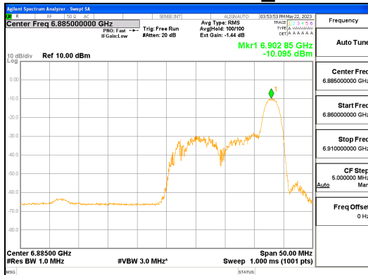
ANT R_802.11ax_HE40_26T_High_UNII 7
