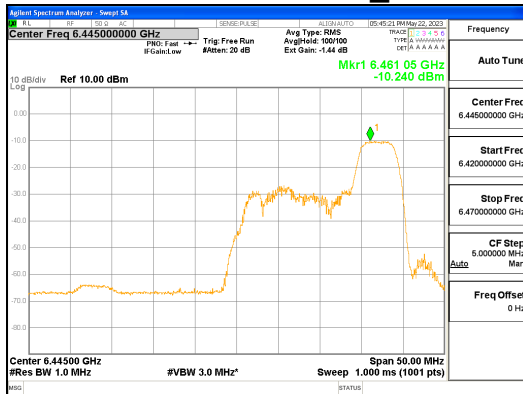
ANT L_802.11ax_HE40_52T_High_UNII 6
