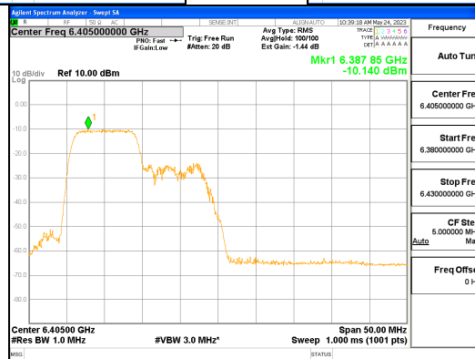
ANT R_802.11ax_HE40_106T_Low_UNII 5
