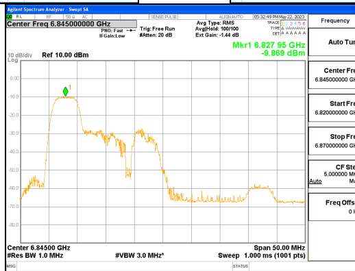
ANT L_802.11ax_HE40_52T_Low_UNII 7
