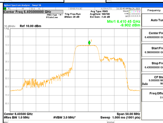
ANT L_802.11ax_HE40_106T_Mid_UNII 5
