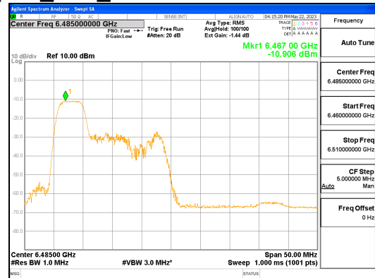
ANT R_802.11ax_HE40_52T_Low_UNII 6
