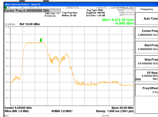
ANT L_802.11ax_HE40_106T_Low_UNII 6
