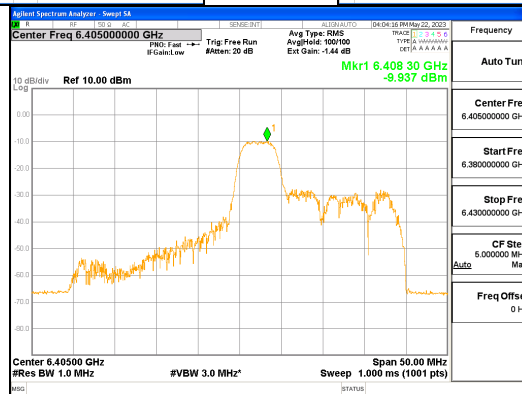
ANT_R_802.11ax_HE40_52T_Mid_UNII 5
