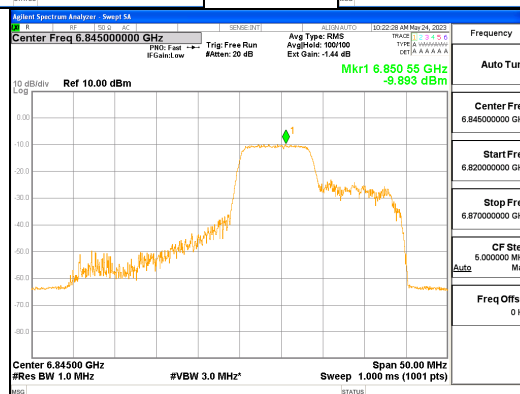
ANT R_802.11ax_HE40_106T_Mid_UNII 7
