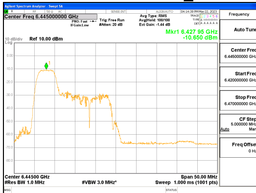
ANT R_802.11ax_HE40_52T_Low_UNII 6
