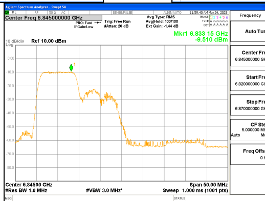
ANT L_802.11ax_HE40_106T_Low_UNII 7
