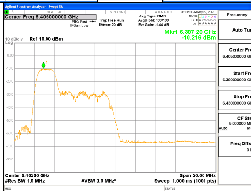
ANT R_802.11ax_HE40_52T_Low_UNII 5
