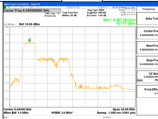
ANT L_802.11ax_HE40_52T_Low_UNII 5
