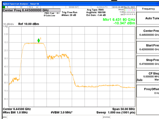
ANT R_802.11ax_HE40_106T_Low_UNII 6
