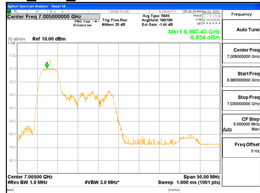
ANT L_802.11ax_HE40_52T_Low_UNII 7
