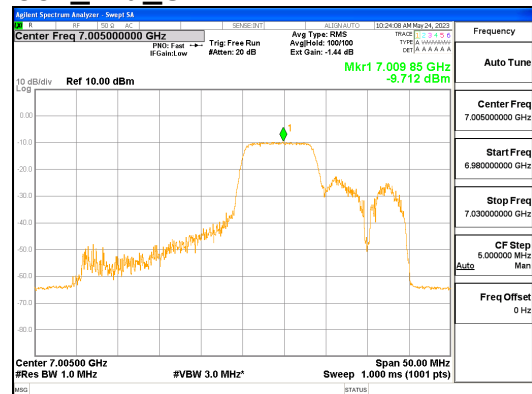
ANT R_802.11ax_HE40_106T_Mid_UNII 7
