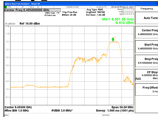
ANT L_802.11ax_HE40_52T_High_UNII 6
