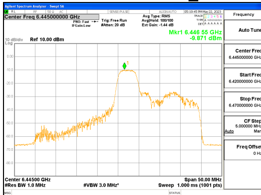
ANT L_802.11ax_HE40_52T_Mid_UNII 6
