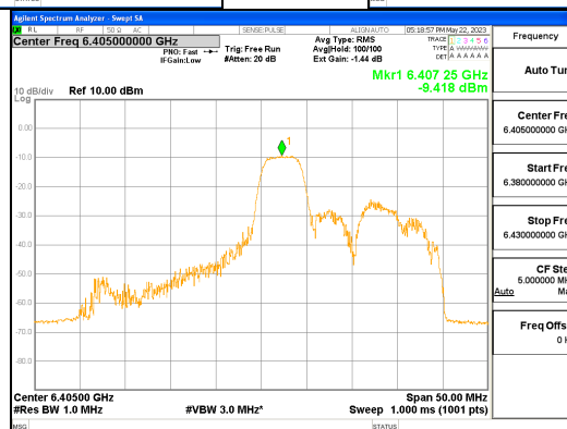
ANT L_802.11ax_HE40_52T_Mid_UNII 5
