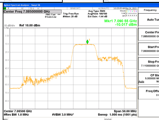
ANT R_802.11ax_HE40_106T_Mid_UNII 8
