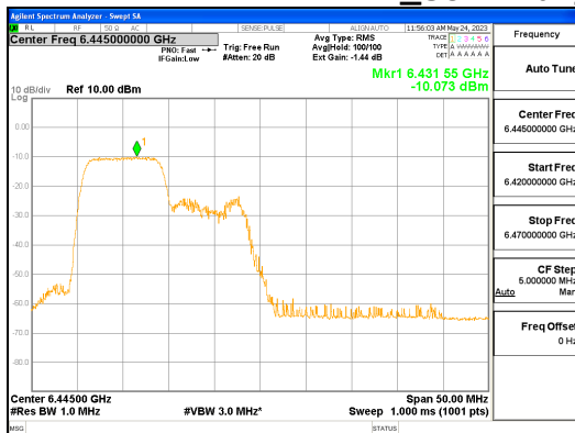
ANT L_802.11ax_HE40_106T_Low_UNII 6
