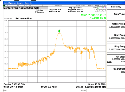
ANT R_802.11ax_HE40_26T_Mid_UNII 7
