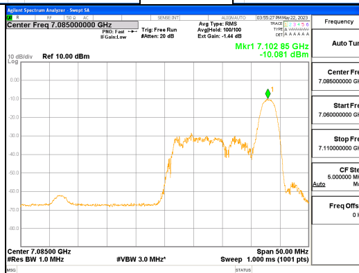
ANT R_802.11ax_HE40_26T_High_UNII 8
