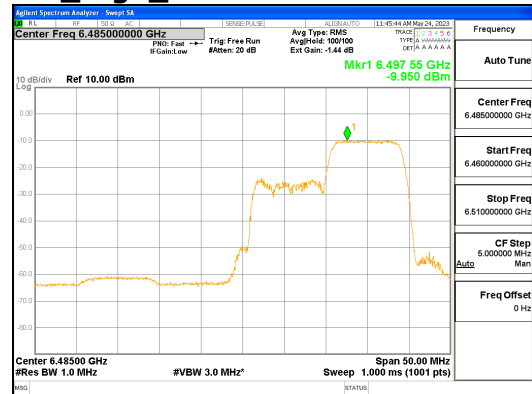
ANT L_802.11ax_HE40_106T_High_UNII 6
