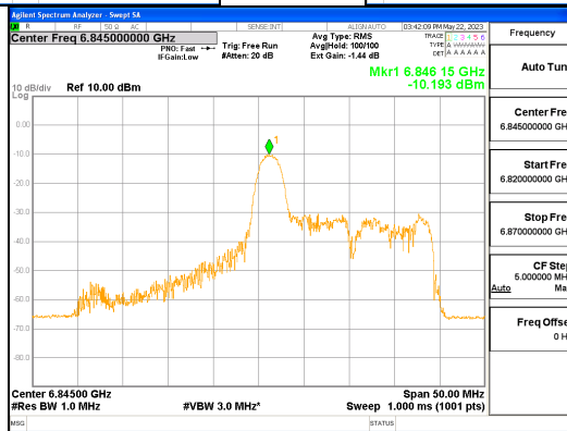
ANT R_802.11ax_HE40_26T_Mid_UNII 7
