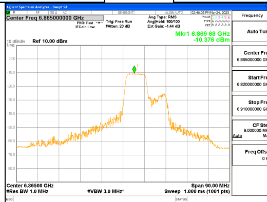
ANT R_802.11ax_HE80_106T_Mid_UNII 7
