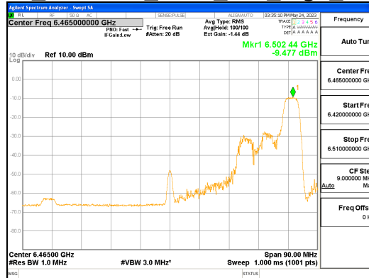
ANT L_802.11ax_HE80_52T_High_UNII 6
