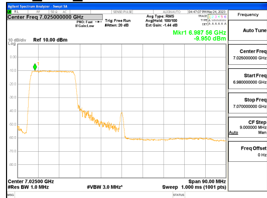
ANT L_802.11ax_HE80_242T_Low_UNII 8
