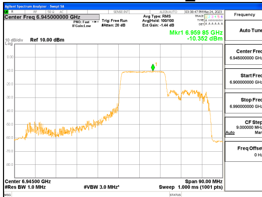
ANT R_802.11ax_HE80_242T_Mid_UNII 8
