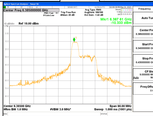
ANT R_802.11ax_HE80_52T_Mid_UNII 5
