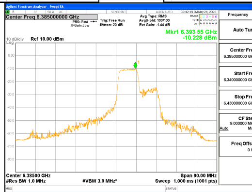
ANT R_802.11ax_HE80_106T_Mid_UNII 5
