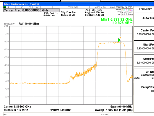
ANT R_802.11ax_HE80_242T_High_UNII 7
