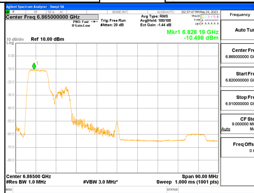
ANT R_802.11ax_HE80_106T_Low_UNII 7
