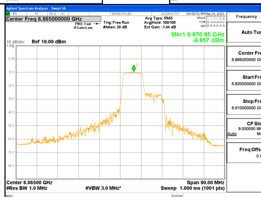
ANT L_802.11ax_HE80_106T_Mid_UNII 7
