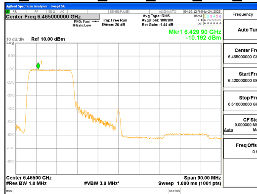
ANT L_802.11ax_HE80_242T_Low_UNII 6
