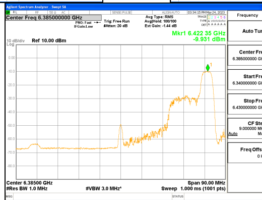
ANT L_802.11ax_HE80_52T_High_UNII 5
