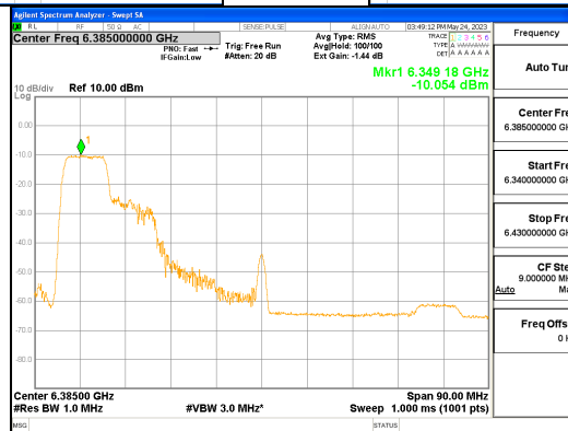
ANT L_802.11ax_HE80_106T_Low_UNII 5
