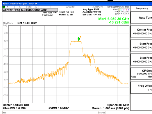
ANT R_802.11ax_HE80_106T_Mid_UNII 8
