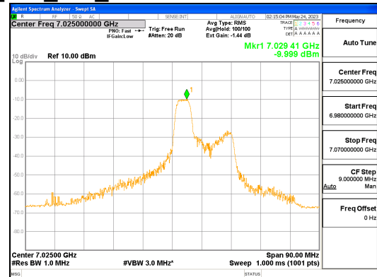
ANT R_802.11ax_HE80_52T_Mid_UNII 8
