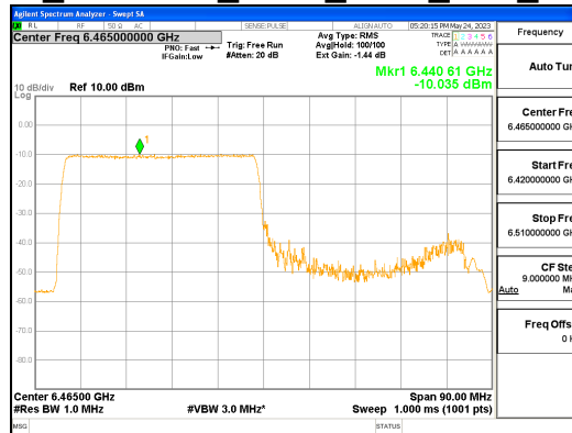
ANT L_802.11ax_HE80_484T_Low_UNII 6
