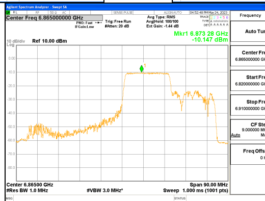
ANT L_802.11ax_HE80_242T_Mid_UNII 7
