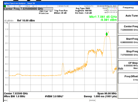
ANT L_802.11ax_HE80_52T_High_UNII 8
