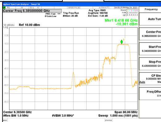
ANT L_802.11ax_HE80_106T_High_UNII 5
