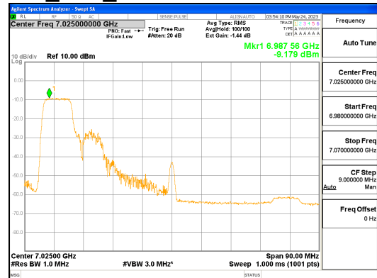
ANT L_802.11ax_HE80_106T_Low_UNII 8
