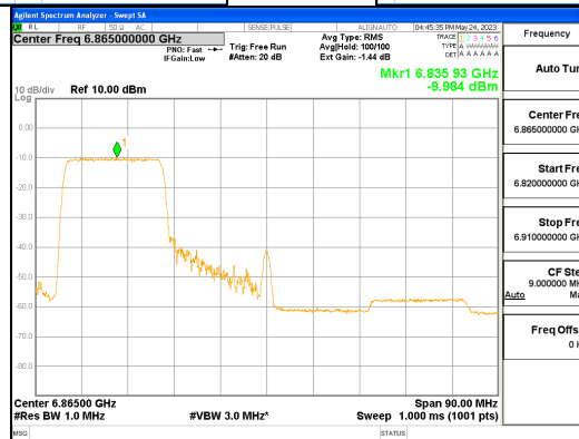
ANT L_802.11ax_HE80_242T_Low_UNII 7
