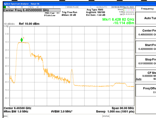
ANT L_802.11ax_HE80_106T_Low_UNII 6
