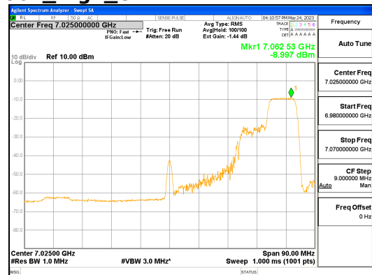
ANT L_802.11ax_HE80_106T_High_UNII 8
