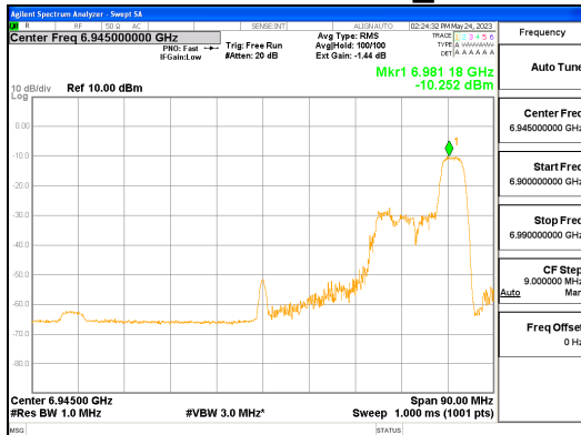
ANT R_802.11ax_HE80_52T_High_UNII 8
