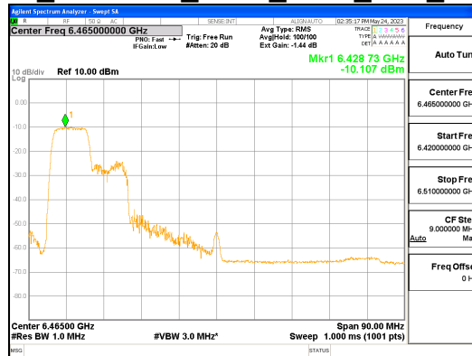
ANT R_802.11ax_HE80_106T_Low_UNII 6
