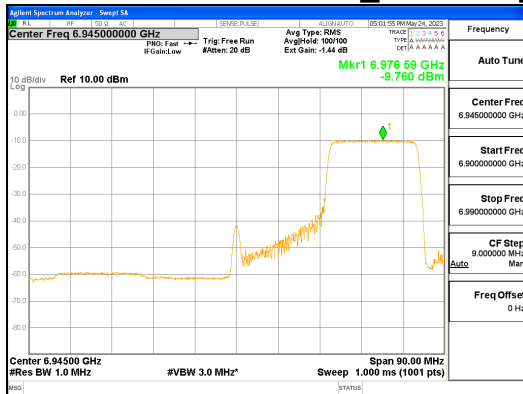
ANT L_802.11ax_HE80_242T_High_UNII 8
