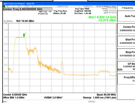
ANT L_802.11ax_HE80_106T_Low_UNII 7
