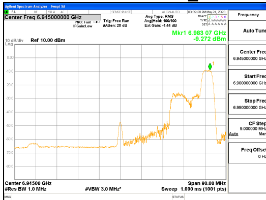
ANT L_802.11ax_HE80_52T_High_UNII 8
