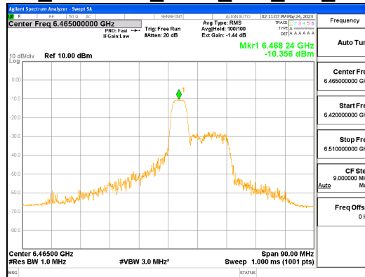
ANT R_802.11ax_HE80_52T_Mid_UNII 6
