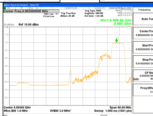
ANT L_802.11ax_HE80_106T_High_UNII 7
