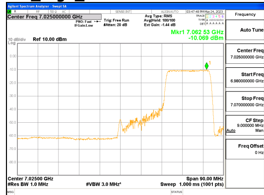
ANT R_802.11ax_HE80_242T_High_UNII 8
