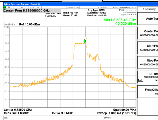
ANT L_802.11ax_HE80_106T_Mid_UNII 5
