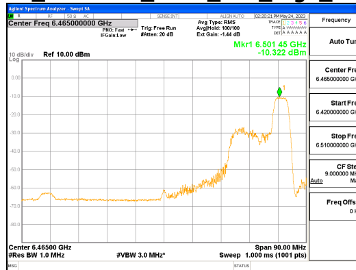
ANT R_802.11ax_HE80_52T_High_UNII 6
