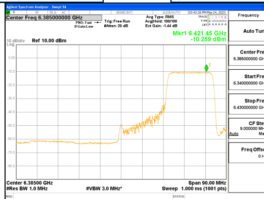
ANT R_802.11ax_HE80_242T_High_UNII 5
