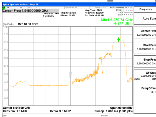
ANT L_802.11ax_HE80_106T_High_UNII 8
