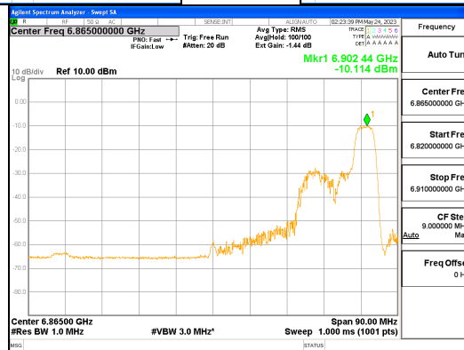
ANT R_802.11ax_HE80_52T_High_UNII 7
