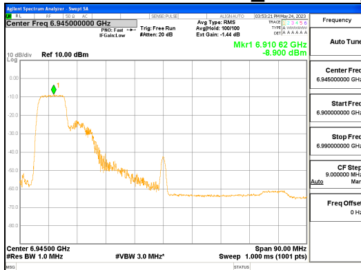
ANT L_802.11ax_HE80_106T_Low_UNII 8
