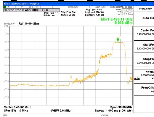
ANT R_802.11ax_HE80_106T_High_UNII 6
