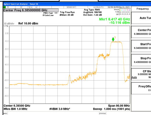
ANT R_802.11ax_HE80_106T_High_UNII 5
