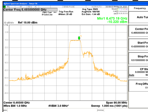
ANT L_802.11ax_HE80_106T_Mid_UNII 6
