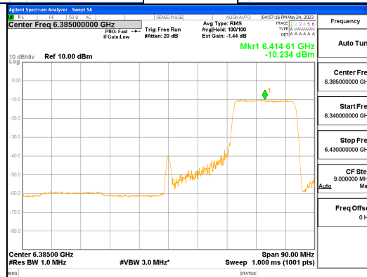
ANT L_802.11ax_HE80_242T_High_UNII 5
