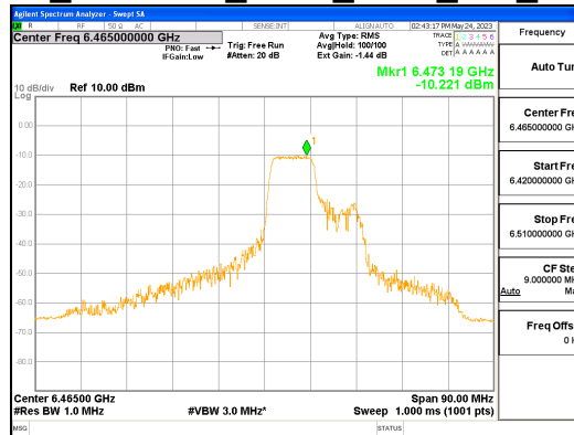
ANT R_802.11ax_HE80_106T_Mid_UNII 6
