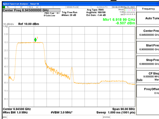
ANT L_802.11ax_HE80_242T_Low_UNII 8
