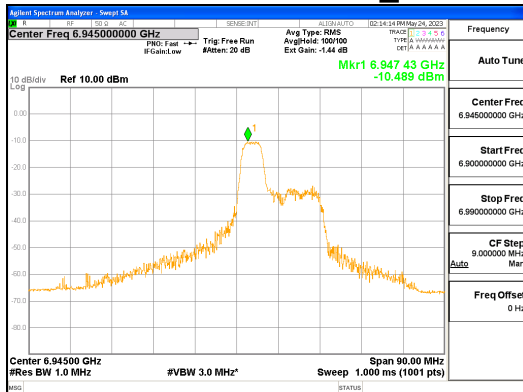
ANT R_802.11ax_HE80_52T_Mid_UNII 8
