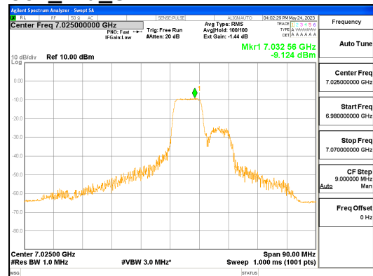
ANT L_802.11ax_HE80_106T_Mid_UNII 8
