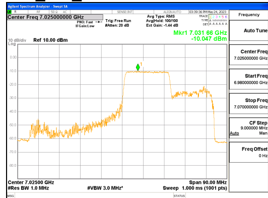
ANT R_802.11ax_HE80_242T_Mid_UNII 8
