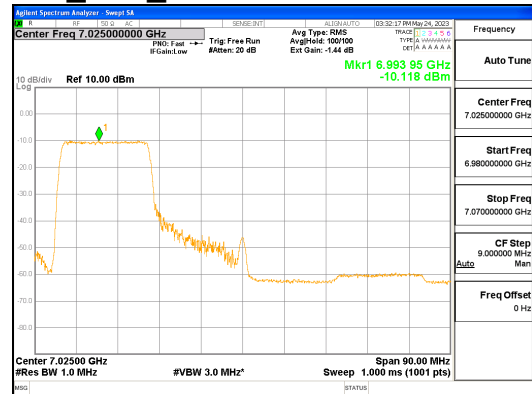
ANT R_802.11ax_HE80_242T_Low_UNII 8
