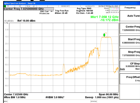
ANT R_802.11ax_HE80_106T_High_UNII 8
