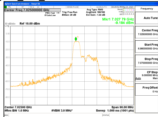
ANT L_802.11ax_HE80_52T_Mid_UNII 8
