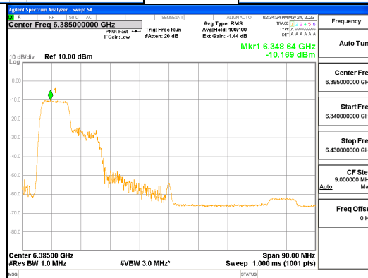
ANT R_802.11ax_HE80_106T_Low_UNII 5
