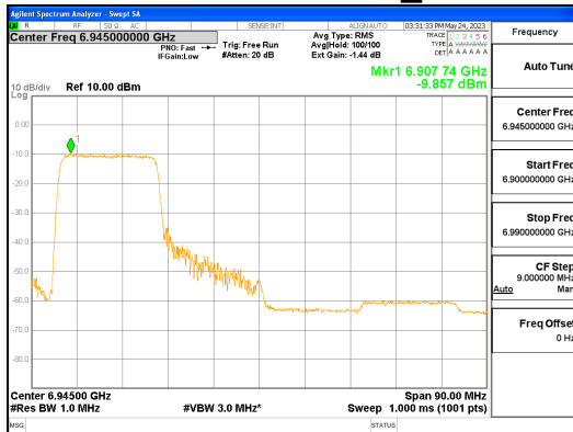
ANT R_802.11ax_HE80_242T_Low_UNII 8
