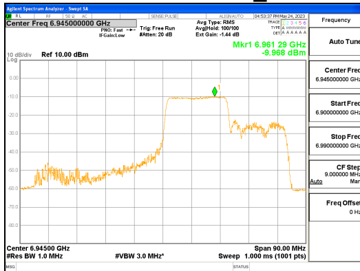
ANT L_802.11ax_HE80_242T_Mid_UNII 8
