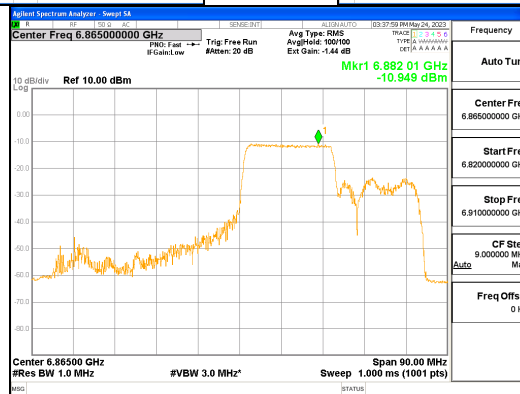
ANT R_802.11ax_HE80_242T_Mid_UNII 7
