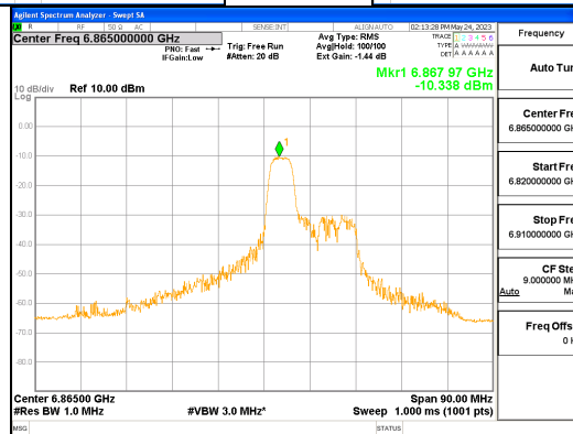
ANT R_802.11ax_HE80_52T_Mid_UNII 7
