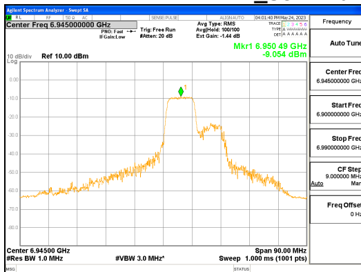
ANT L_802.11ax_HE80_106T_Mid_UNII 8
