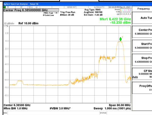
ANT R_802.11ax_HE80_52T_High_UNII 5
