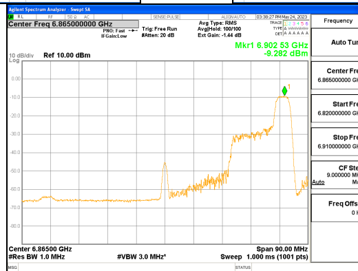
ANT L_802.11ax_HE80_52T_High_UNII 7
