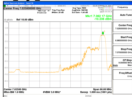
ANT R_802.11ax_HE80_52T_High_UNII 8
