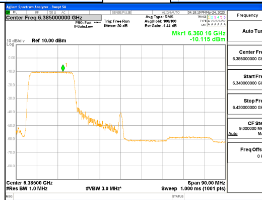
ANT L_802.11ax_HE80_242T_Low_UNII 5
