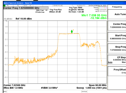
ANT L_802.11ax_HE80_242T_Mid_UNII 8
