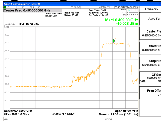
ANT R_802.11ax_HE80_242T_High_UNII 6
