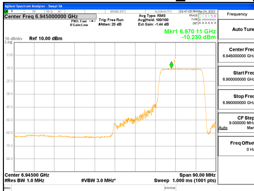
ANT R_802.11ax_HE80_242T_High_UNII 8
