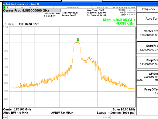
ANT L_802.11ax_HE80_52T_Mid_UNII 7
