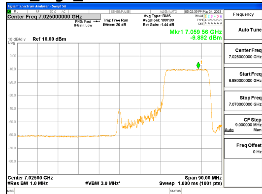
ANT L_802.11ax_HE80_242T_High_UNII 8
