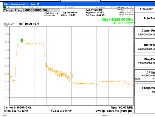
ANT R_802.11ax_HE80_242T_Low_UNII 7
