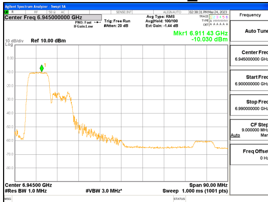
ANT R_802.11ax_HE80_106T_Low_UNII 8
