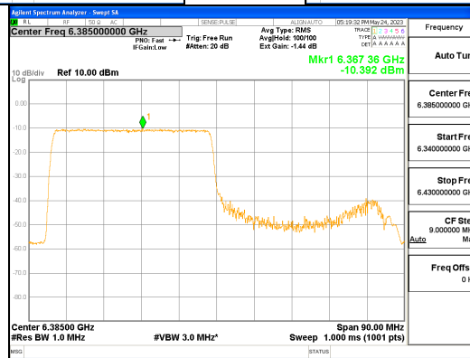
ANT L_802.11ax_HE80_484T_Low_UNII 5
