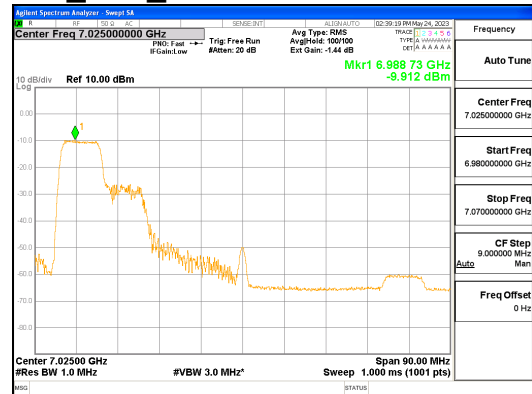
ANT R_802.11ax_HE80_106T_Low_UNII 8
