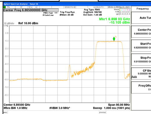
ANT L_802.11ax_HE80_242T_High_UNII 7
