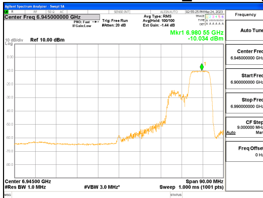
ANT R_802.11ax_HE80_106T_High_UNII 8
