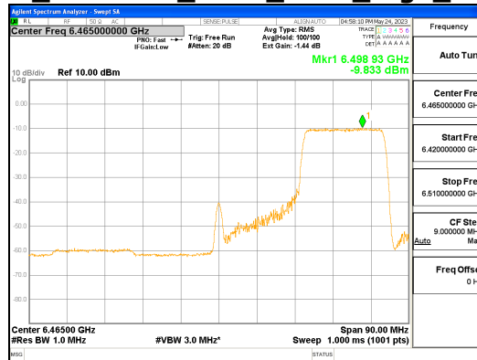
ANT L_802.11ax_HE80_242T_High_UNII 6
