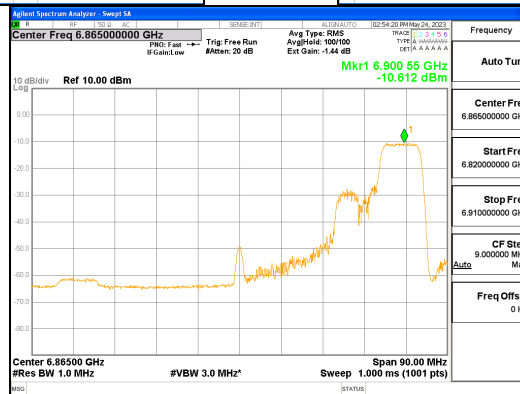
ANT R_802.11ax_HE80_106T_High_UNII 7
