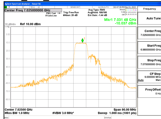
ANT R_802.11ax_HE80_106T_Mid_UNII 8
