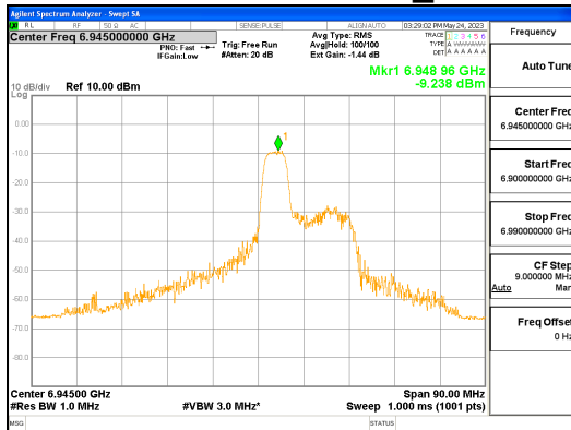
ANT L_802.11ax_HE80_52T_Mid_UNII 8
