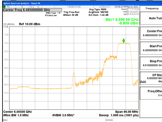
ANT L_802.11ax_HE80_106T_High_UNII 6
