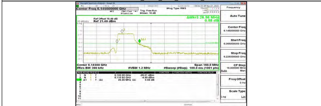
11AX80MIMO_ANT1_6145_242Tone_RU61
