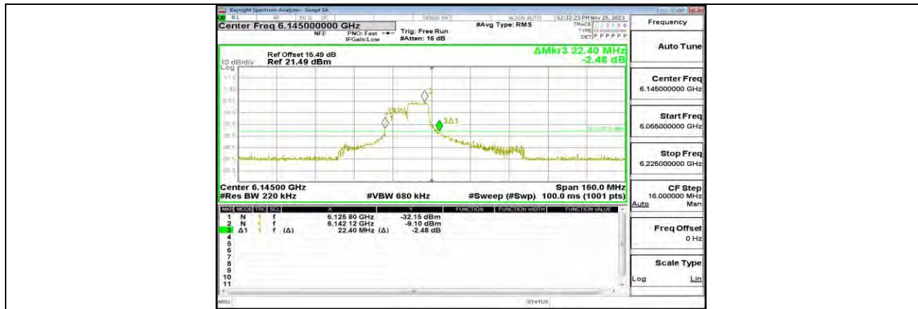
11AX80MIMO_ANT1_6145_106Tone_RU56
