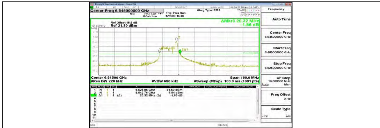
11AX80MIMO_ANT1_6545_26Tone_RU17
