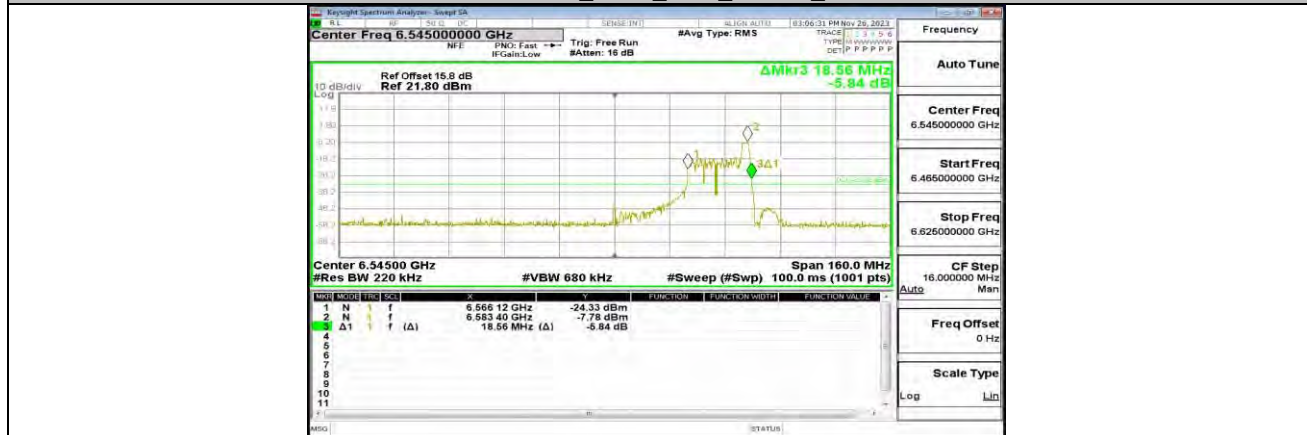
11AX80MIMO_ANT1_6545_26Tone_RU36
