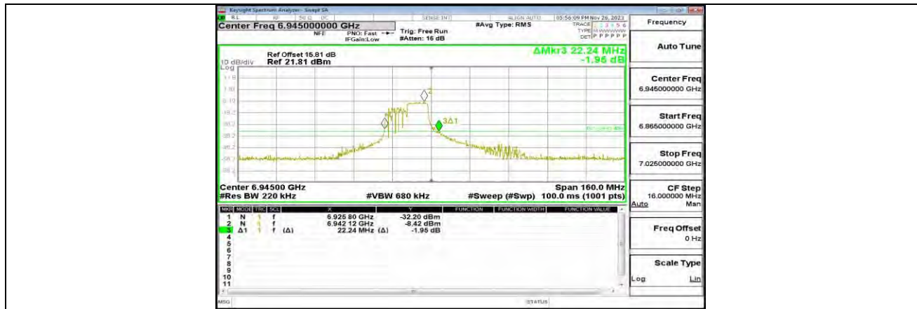
11AX80MIMO_ANT1_6945_106Tone_RU56
