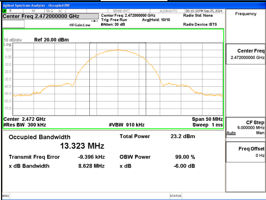
ANT R, 802.11b, 99% Bandwidth
