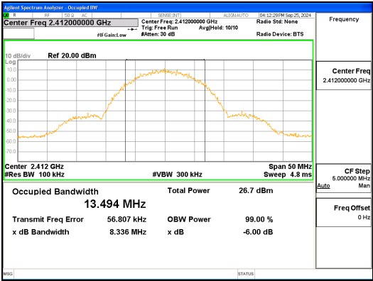
ANT L, 802.11b, 6dB Bandwidth
