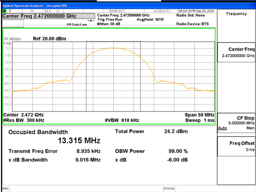
ANT L, 802.11b, 99% Bandwidth
