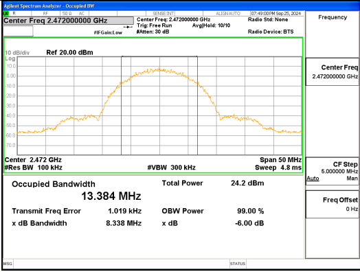
ANT R, 802.11b, 6dB Bandwidth
