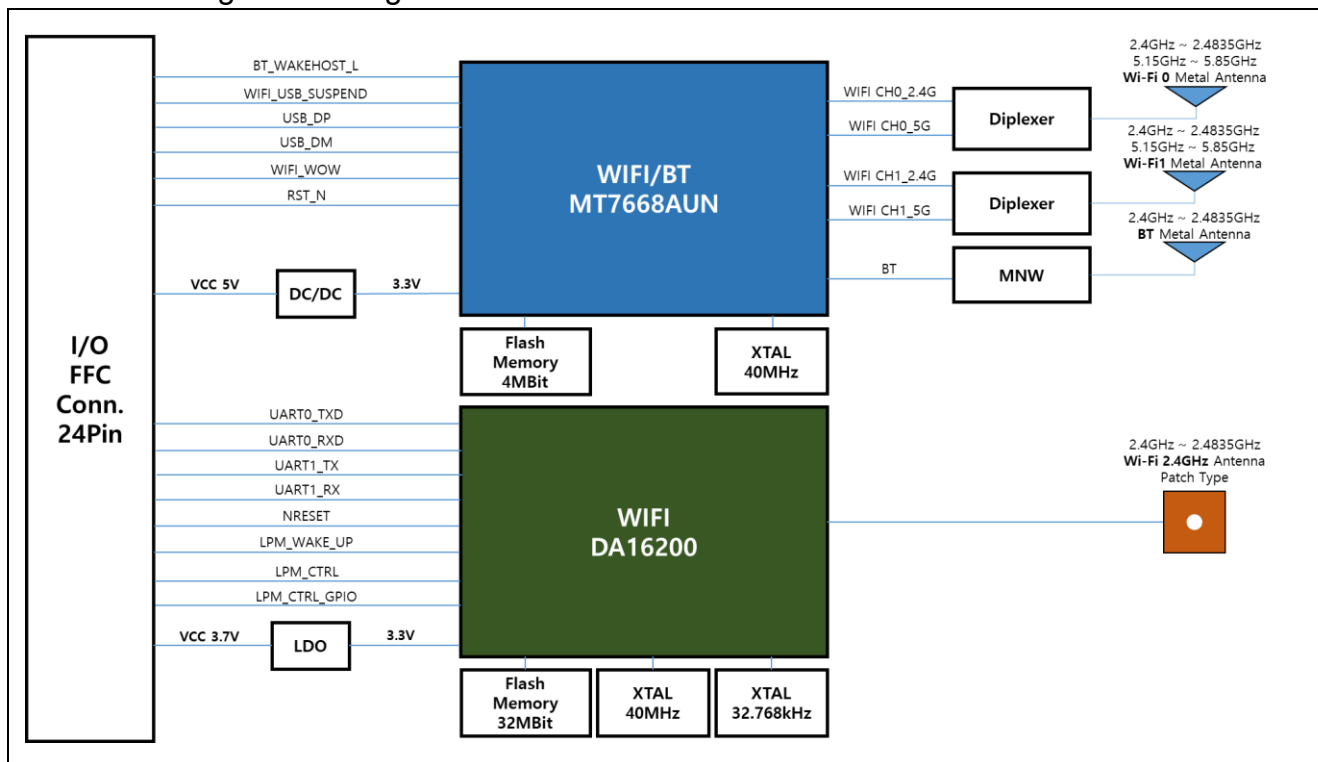
Figure 1-1 Block Diagram and Interface
