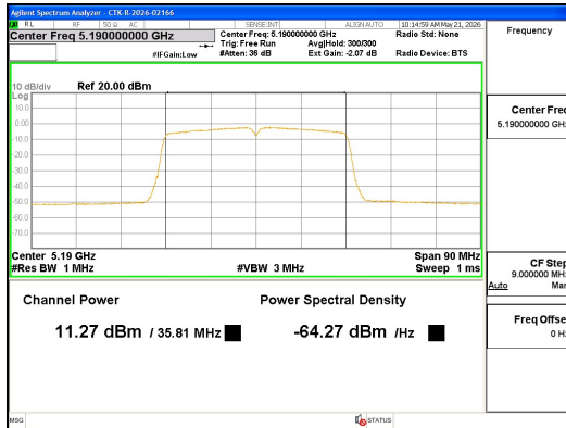
ANT0_802.11ac_VHT40_UNI1
