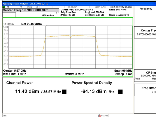
ANT0_802.11ac_VHT40_UNI1 2C
