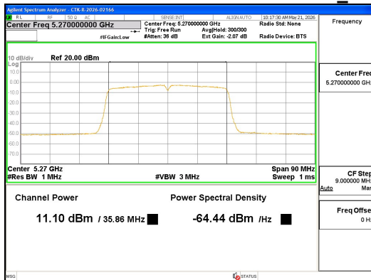
ANT0_802.11ac_VHT40_UNI1 2A
