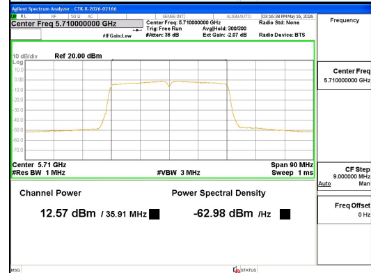
ANT0_802.11ac_VHT40_UNI1 2C
