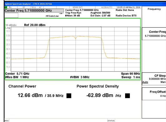
ANT1_802.11n_HT40_UNII 2C
