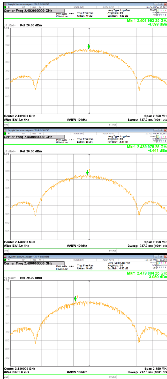
Bluetooth LE 1 Mbps
