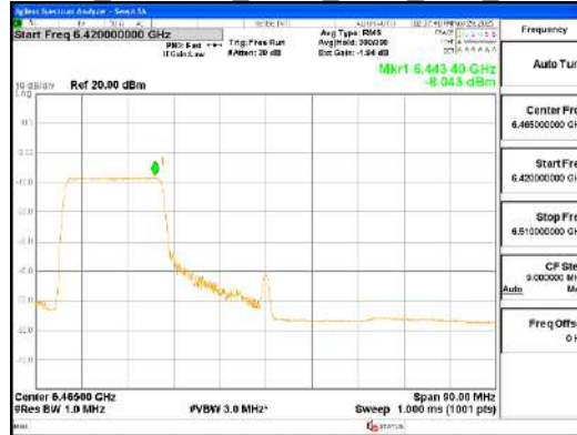
ANT0_802.11ax_HE80_242T_Low_UNII 6
