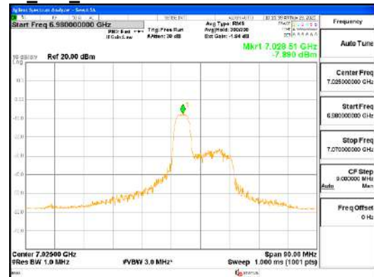
ANT0_802.11ax_HE80_52T_Mid_UNII 8
