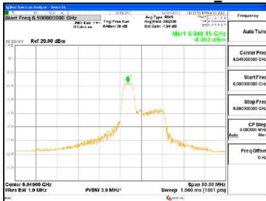
ANT0_802.11ax_HE80_52T_Mid_UNII 8
