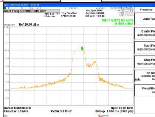
ANTO_802.11ax_HE80_106T_Mid_UNII 7
