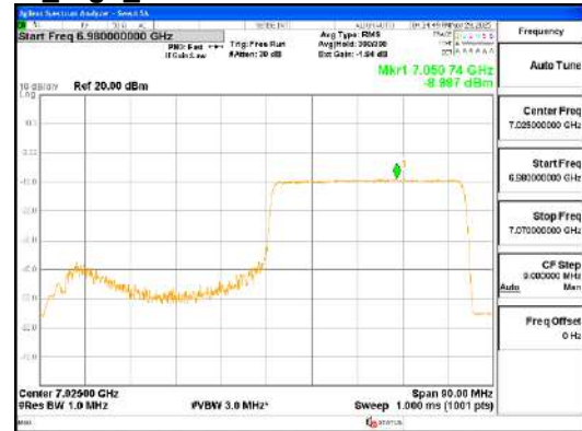
ANT0_802.11ax_HE80_484T_High_UNII 8
