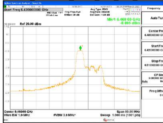
ANT1_802.11ax_HE80_52T_Mid_UNII 6
