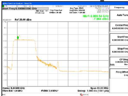
ANT0_802.11ax_HE80_242T_Low_UNII 8
