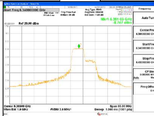
ANT1_802.11ax_HE80_106T_Mid_UNII 5
