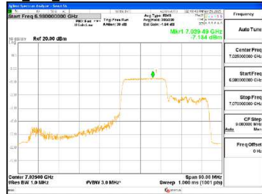
ANTO_802.11ax_HE80_242T_Mid_UNII 8
