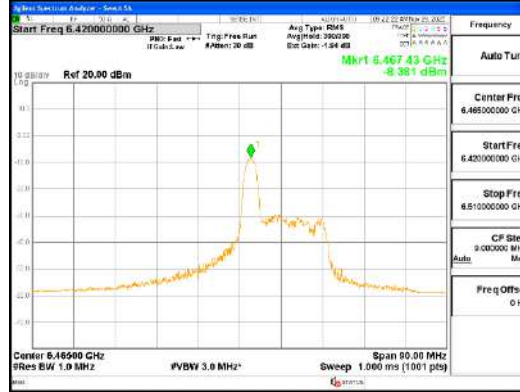
ANT1_802.11ax_HE80_26T_Mid_UNII 6
