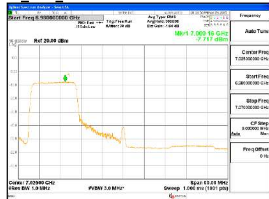
ANT1_802.11ax_HE80_242T_Low_UNII 8
