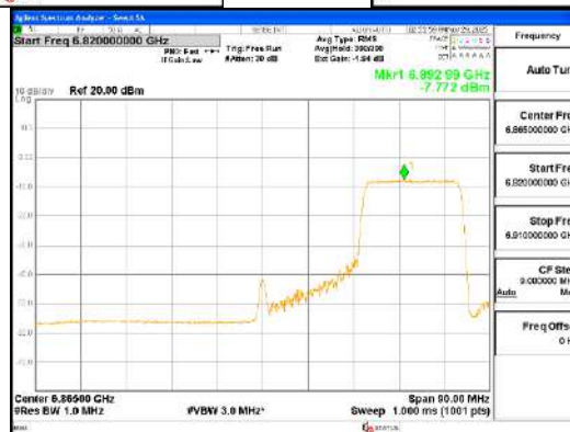
ANT0_802.11ax_HE80_242T_High_UNII 7
