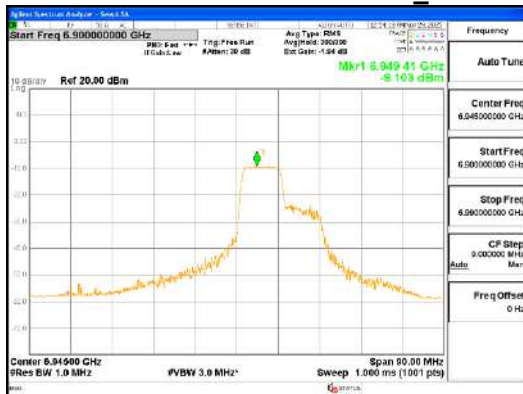
ANTO_802.11ax_HE80_106T_Mid_UNII 8
