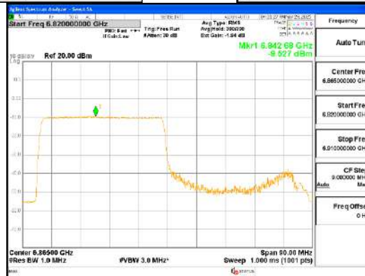
ANT1_802.11ax_HE80_484T_Low_UNII 7
