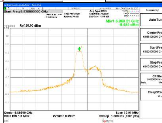
ANT1_802.11ax_HE80_52T_Mid_UNII 7
