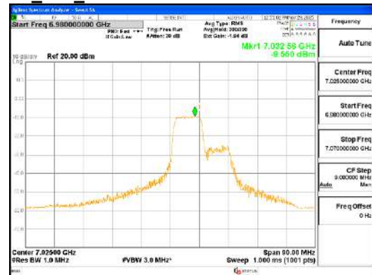
ANTO_802.11ax_HE80_106T_Mid_UNII 8
