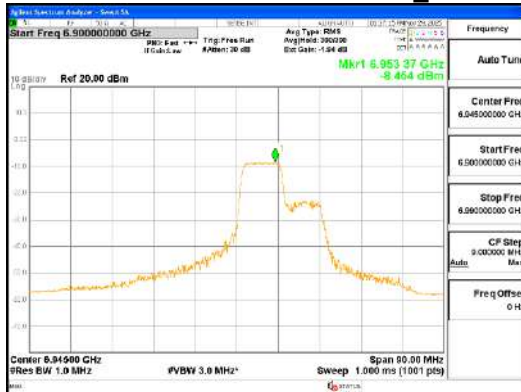
ANT1_802.11ax_HE80_106T_Mid_UNII 8
