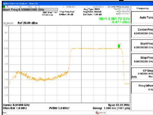
ANT0_802.11ax_HE80_484T_High_UNII 8
