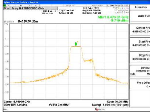
ANT1_802.11ax_HE80_106T_Mid_UNII 6
