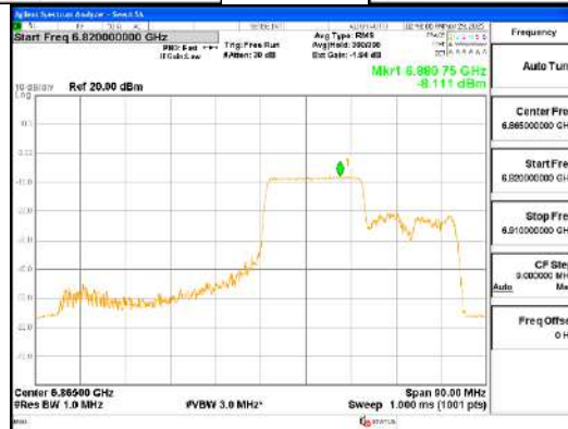
ANTO_802.11ax_HE80_242T_Mid_UNII 7
