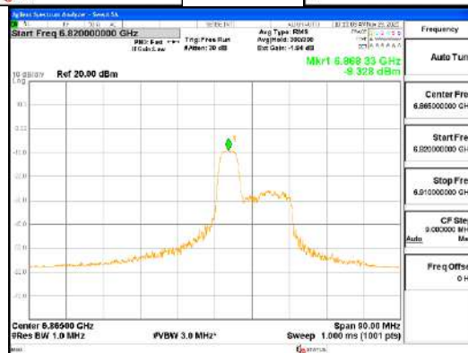
ANT0_802.11ax_HE80_52T_Mid_UNII 7
