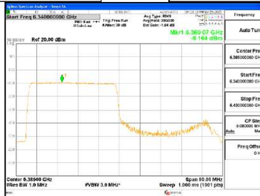
ANT1_802.11ax_HE80_484T_Low_UNII 5
