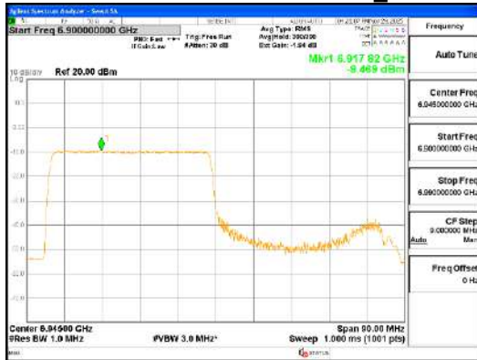
ANT0_802.11ax_HE80_484T_Low_UNII 8
