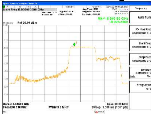
ANTO_802.11ax_HE80_242T_Mid_UNII 8
