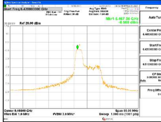
ANT0_802.11ax_HE80_52T_Mid_UNII 6
