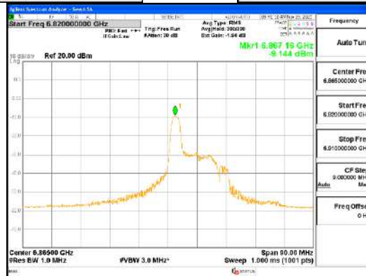
ANT0_802.11ax_HE80_26T_Mid_UNII 7
