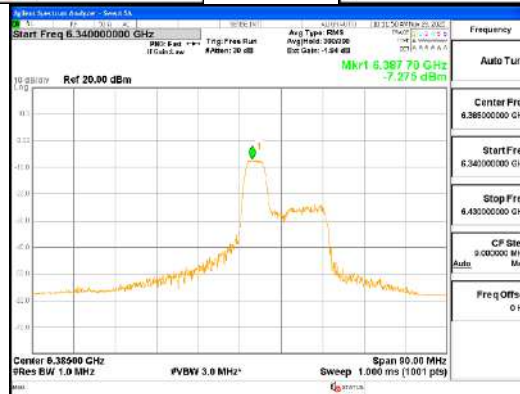
ANT0_802.11ax_HE80_52T_Mid_UNII 5
