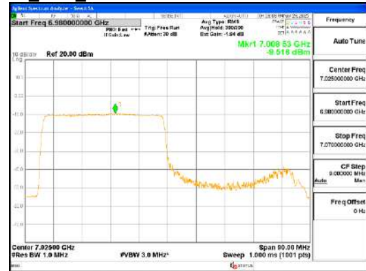
ANT1_802.11ax_HE80_484T_Low_UNII 8
