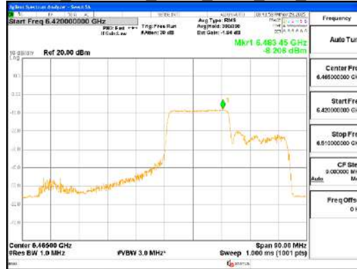
ANT1_802.11ax_HE80_242T_Mid_UNII 6
