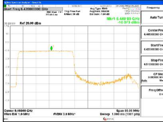
ANT1_802.11ax_HE80_484T_Low_UNII 6
