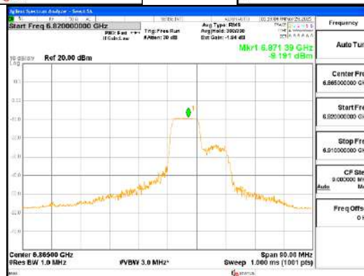
ANT1_802.11ax_HE80_106T_Low_UNII 7
