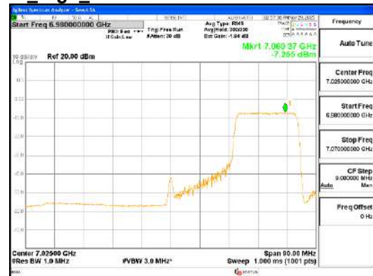
ANT0_802.11ax_HE80_242T_High_UNII 8
