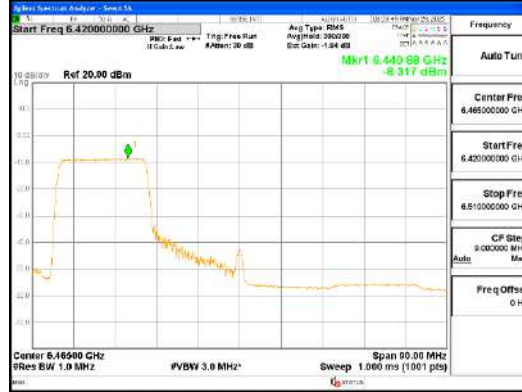
ANT1_802.11ax_HE80_242T_Low_UNII 6
