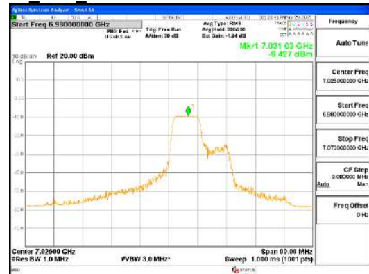
ANT1_802.11ax_HE80_106T_Low_UNII 8
