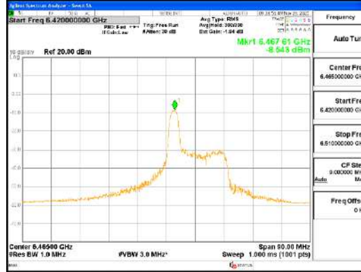
ANT0_802.11ax_HE80_26T_Mid_UNII 6
