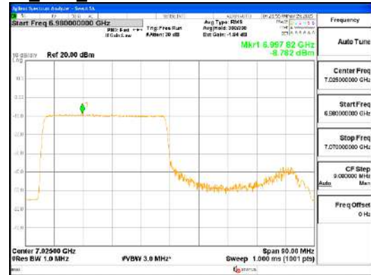
ANT0_802.11ax_HE80_484T_Low_UNII 8
