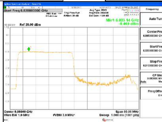
ANT0_802.11ax_HE80_484T_Low_UNII 7
