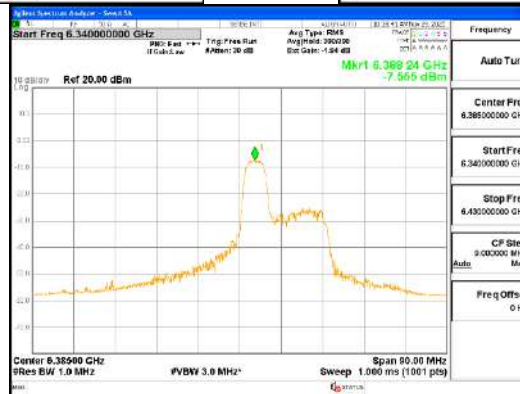
ANT1_802.11ax_HE80_52T_Mid_UNII 5
