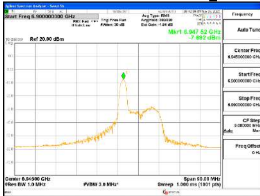
ANT0_802.11ax_HE80_26T_Mid_UNII 8
