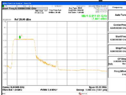
ANT1_802.11ax_HE80_242T_Low_UNII 8
