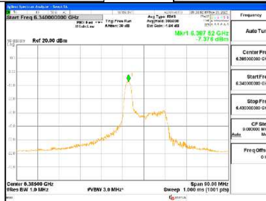
ANT0_802.11ax_HE80_26T_Mid_UNII 5
