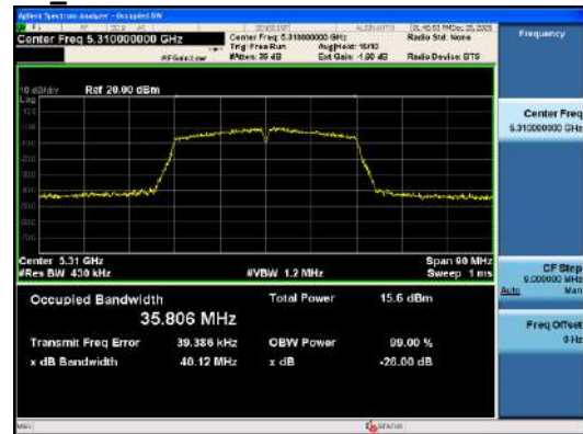
ANT0_802.11ac_VHT40_UNI 2A
