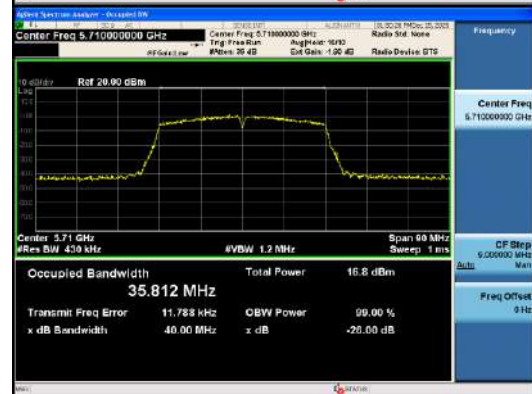
ANT0_802.11ac_VHT40_UNI 2C
