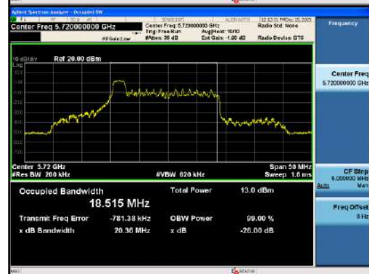
ANT1_802.11ax_HE20_26T_Low_UNII 2C
