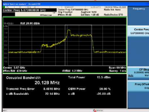
ANT0_802.11ax_HE40_26T_Mid_UNII 2C
