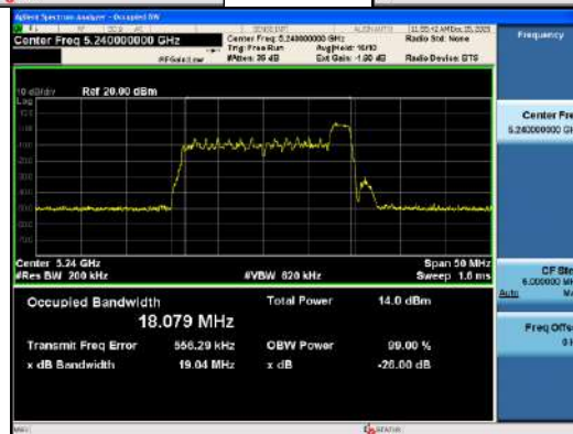
ANT0_802.11ax_HE20_26T_High_UNII 1
