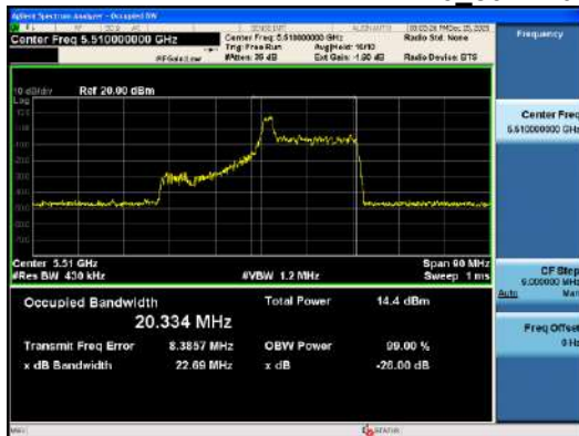
ANT0_802.11ax_HE40_26T_Mid_UNII 2A
