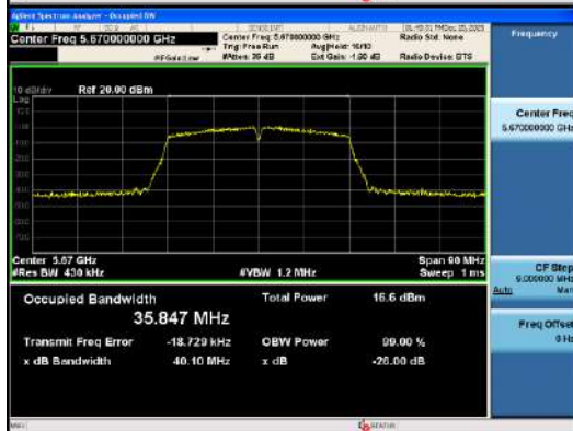
ANT0_802.11ac_VHT40_UNI 2C
