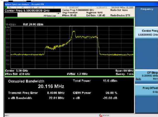
ANT0_802.11ax_HE40_26T_Mid_UNII 2A
