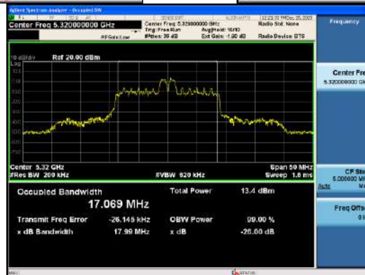
ANT1_802.11ax_HE20_26T_Mid_UNI1 2A
