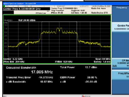
ANT0_802.11ax_HE20_26T_Mid_UNII 2A
