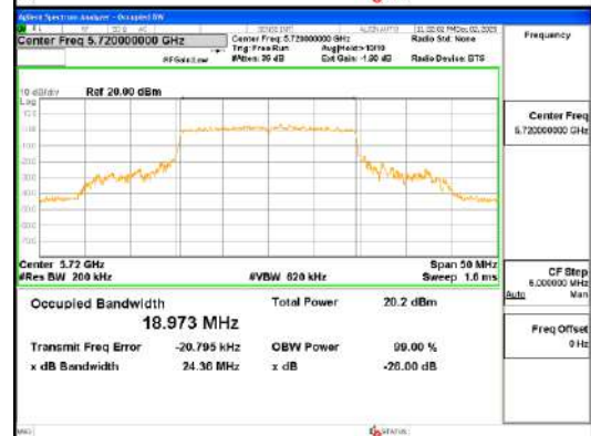
ANT1_802.11ax_HE20_242T_UNII 2C
