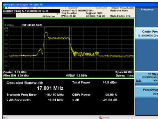
ANT0_802.11ax_HE40_26T_Low_UNII 1
