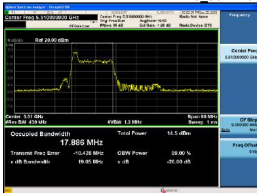
ANT0_802.11ax_HE40_26T_Low_UNII 2A
