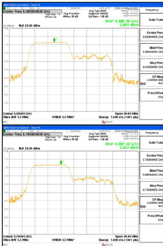
ANT0_802.11ax_HE20_106T_Low_UNII 2C
