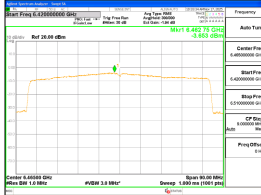
802.11ax_HE80_SU_UNII 6
