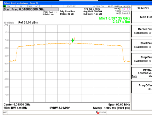
802.11ax_HE80_SU_UNII 5
