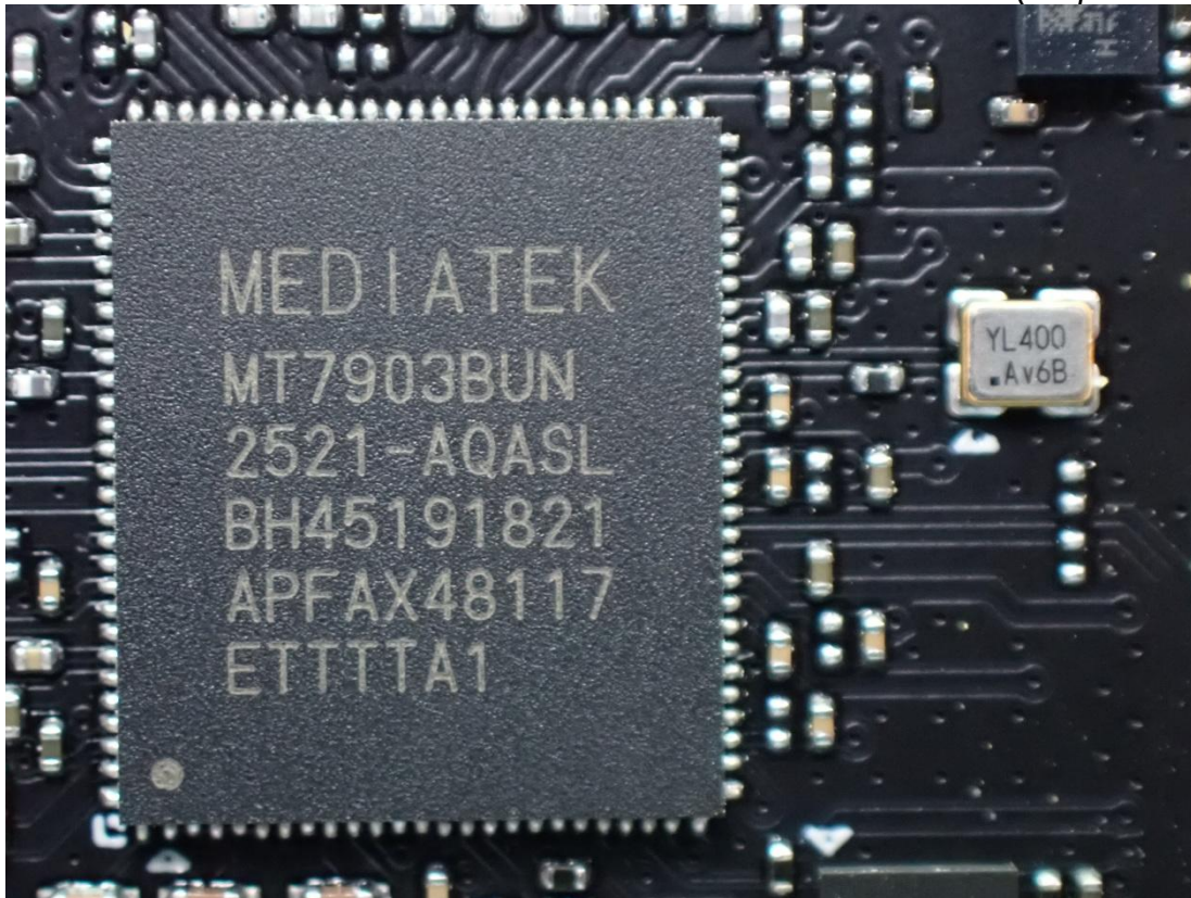
Figure 9 Internal View (Chip MT7921AUN)
