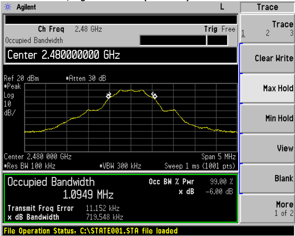
6 dB Bandwidth, Highest Channel (2480 MHz)
