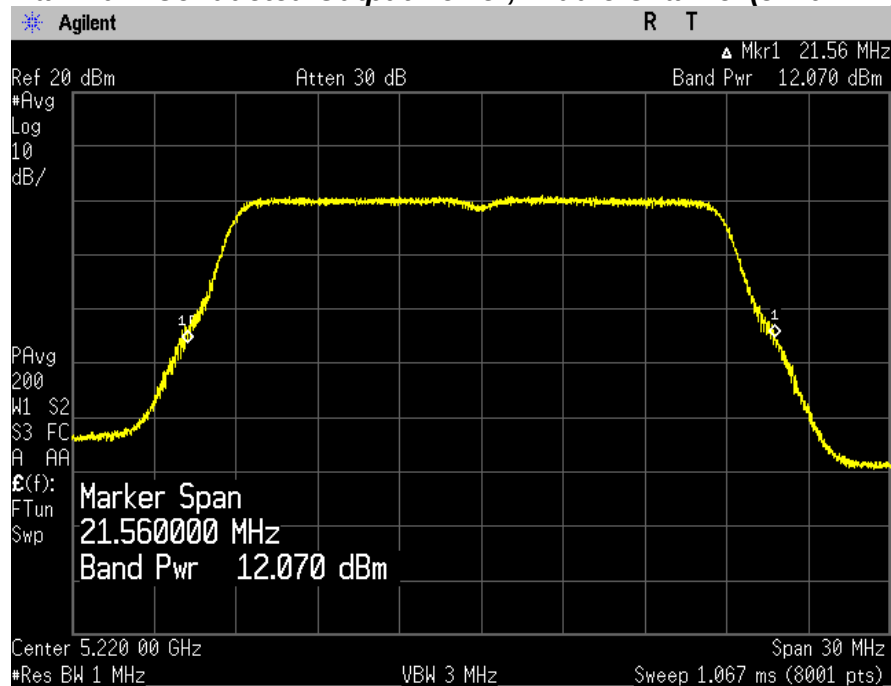
Maximum Conducted Output Power, Middle Channel (5220 MHz)
