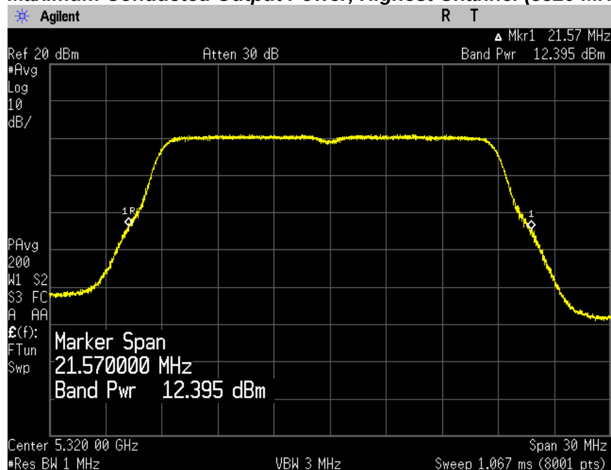
Maximum Conducted Output Power, Highest Channel (5320 MHz)
