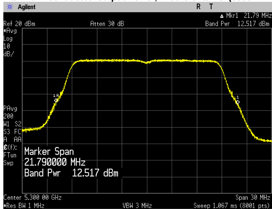
Maximum Conducted Output Power, Middle Channel (5300 MHz)
