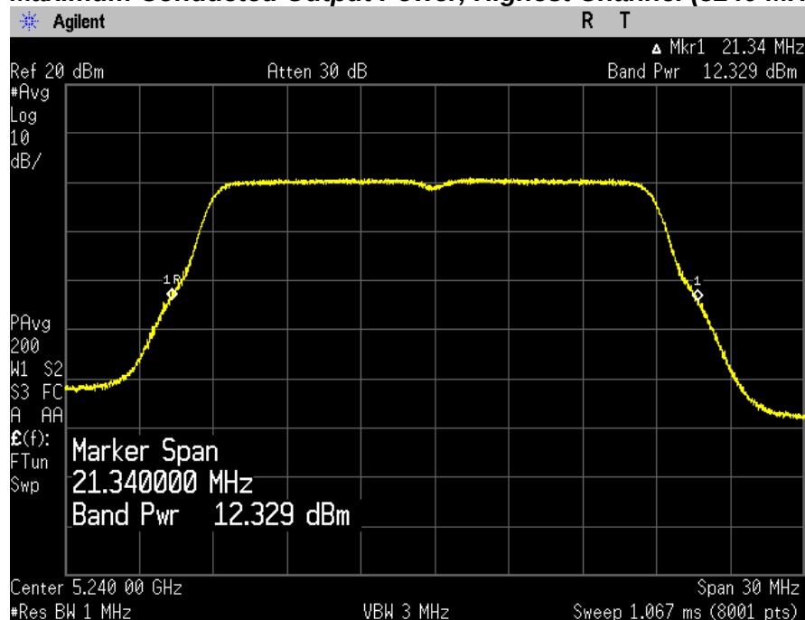
Maximum Conducted Output Power, Highest Channel (5240 MHz)
