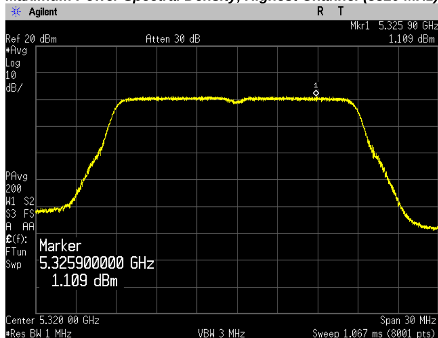
Maximum Power Spectral Density, Highest Channel (5320 MHz)
