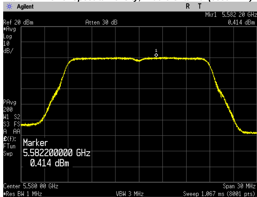
Maximum Power Spectral Density, Middle Channel (5580 MHz)
