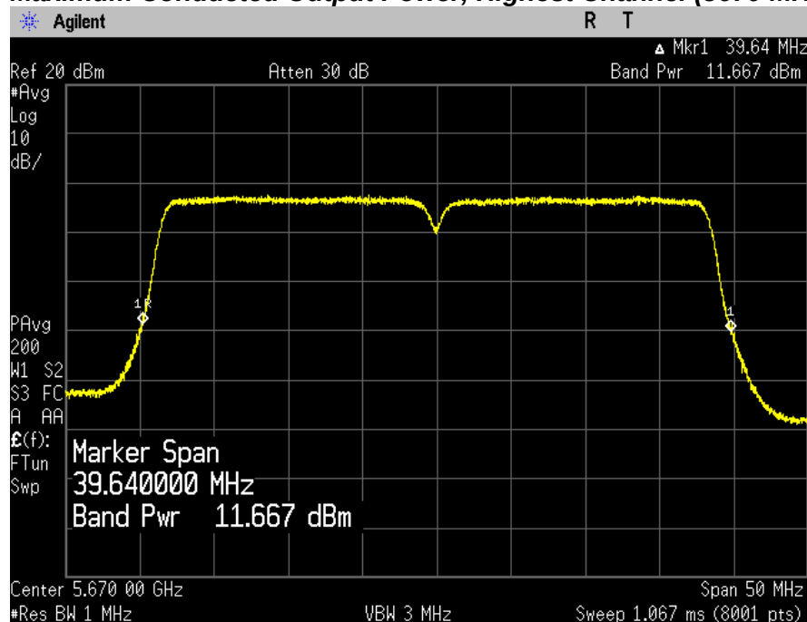
Maximum Conducted Output Power, Highest Channel (5670 MHz)
