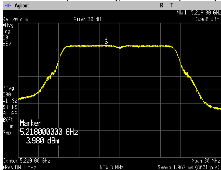
Maximum Power Spectral Density, Middle Channel (5220 MHz)
