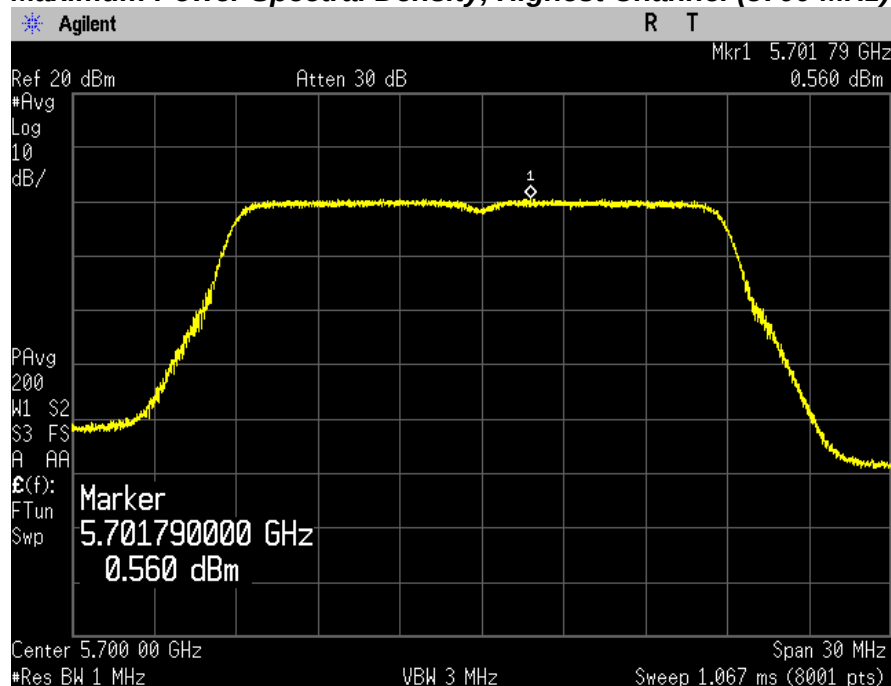
Maximum Power Spectral Density, Highest Channel (5700 MHz)
