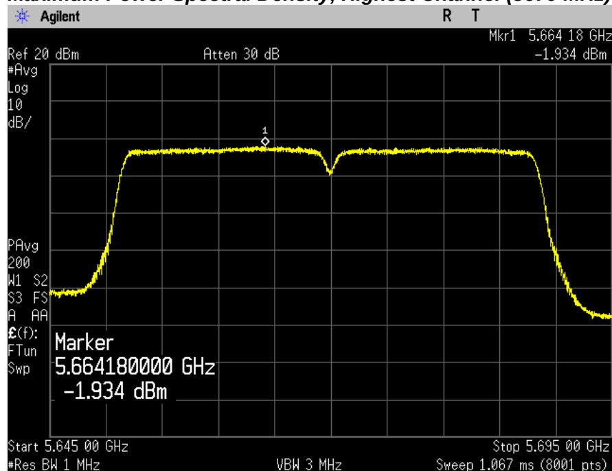
Maximum Power Spectral Density, Highest Channel (5670 MHz)
