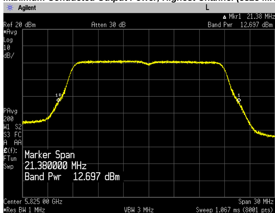
Maximum Conducted Output Power, Highest Channel (5825 MHz)
