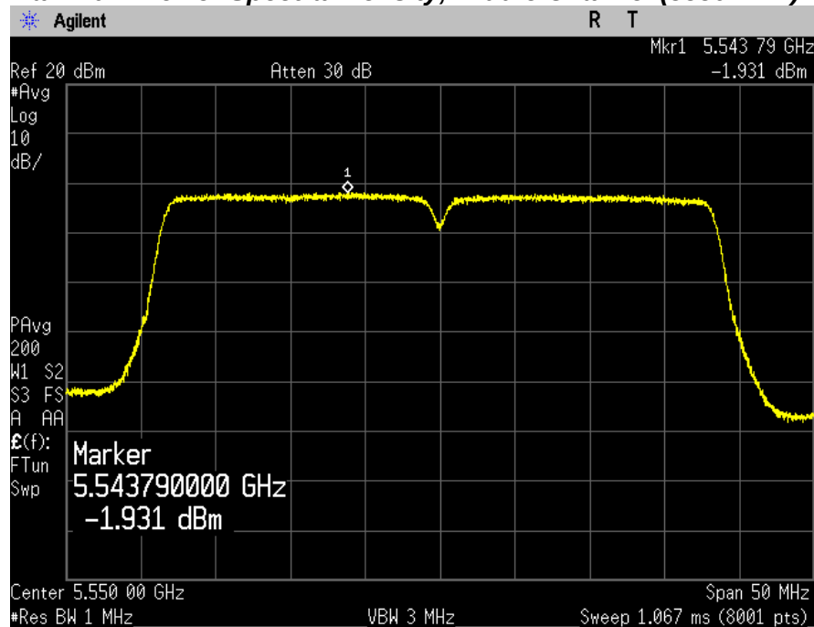
Maximum Power Spectral Density, Middle Channel (5550 MHz)
