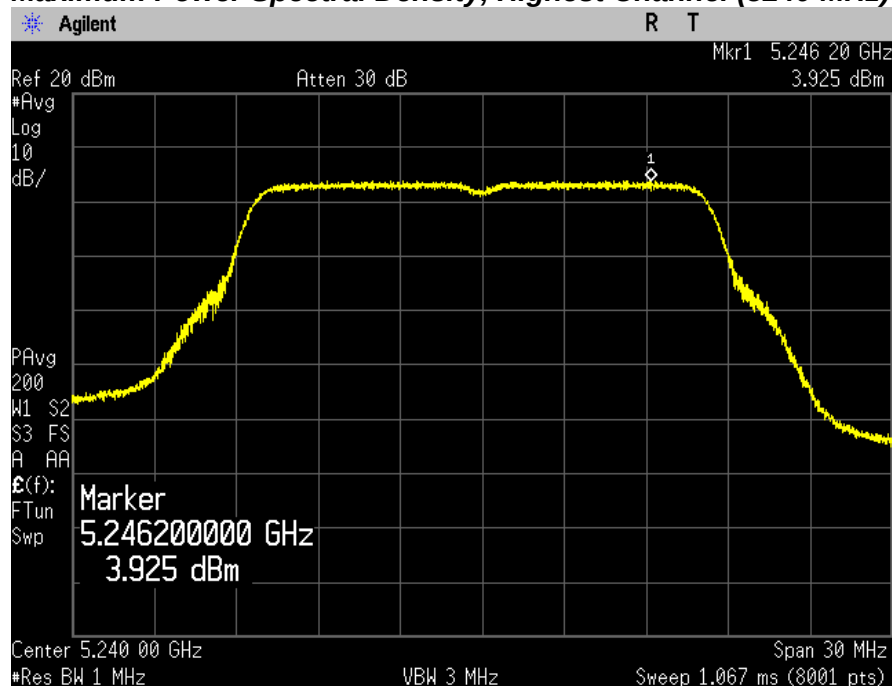
Maximum Power Spectral Density, Highest Channel (5240 MHz)
