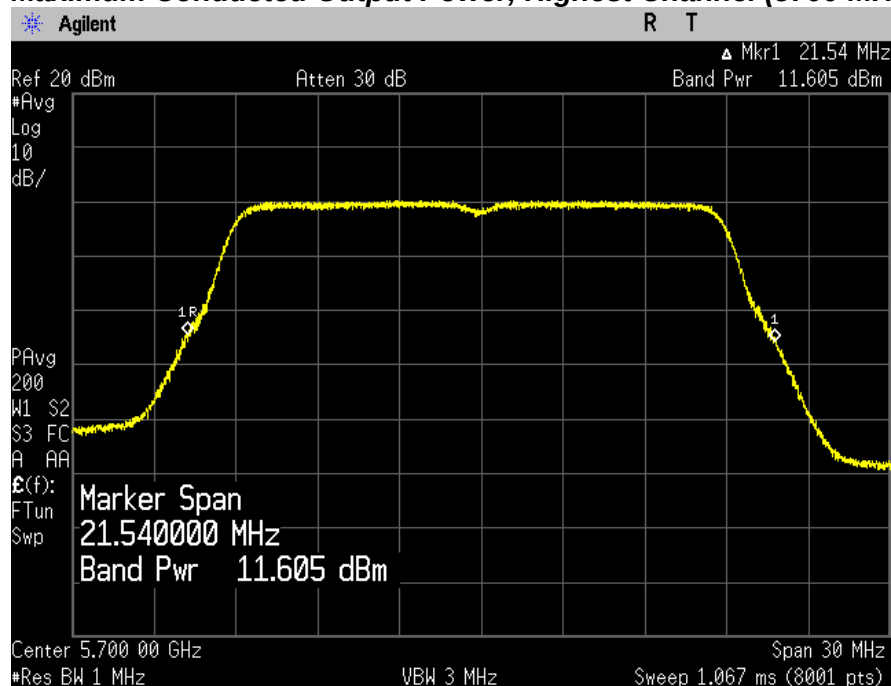
Maximum Conducted Output Power, Highest Channel (5700 MHz)
