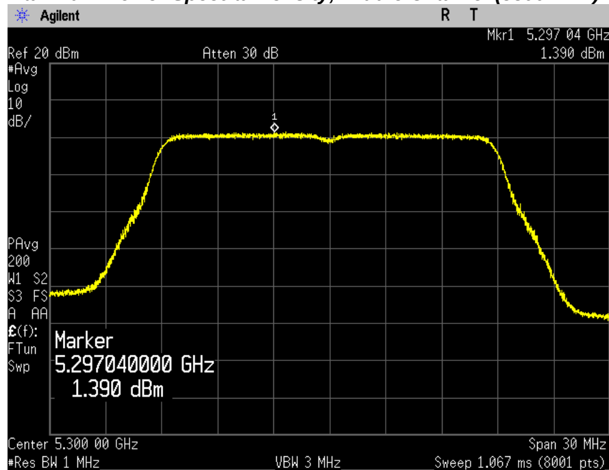
Maximum Power Spectral Density, Middle Channel (5300 MHz)
