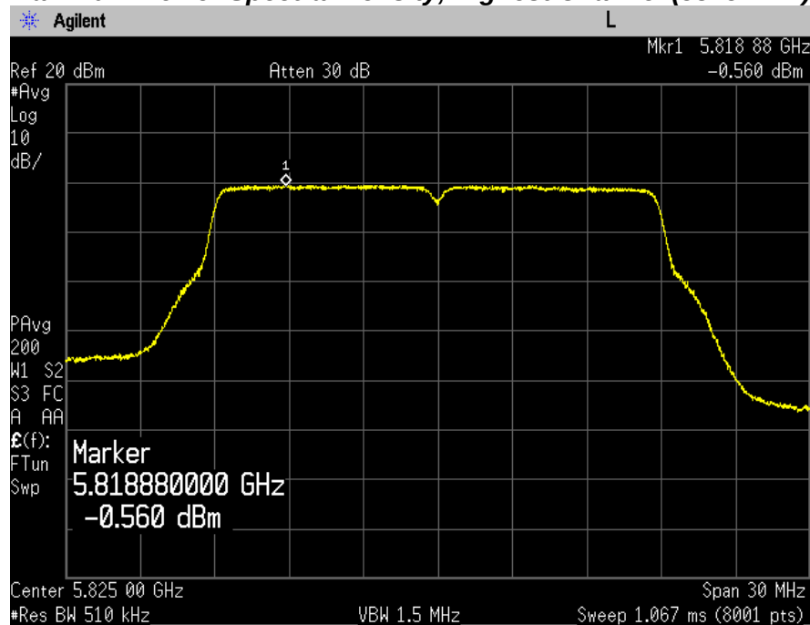
Maximum Power Spectral Density, Highest Channel (5825 MHz)
