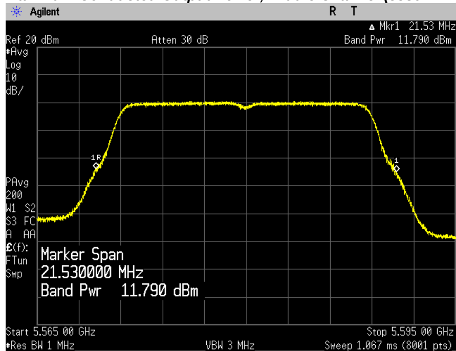
Maximum Conducted Output Power, Middle Channel (5580 MHz)
