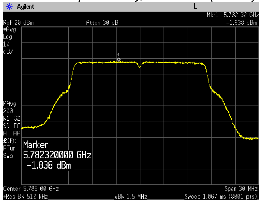
Maximum Power Spectral Density, Middle Channel (5785 MHz)
