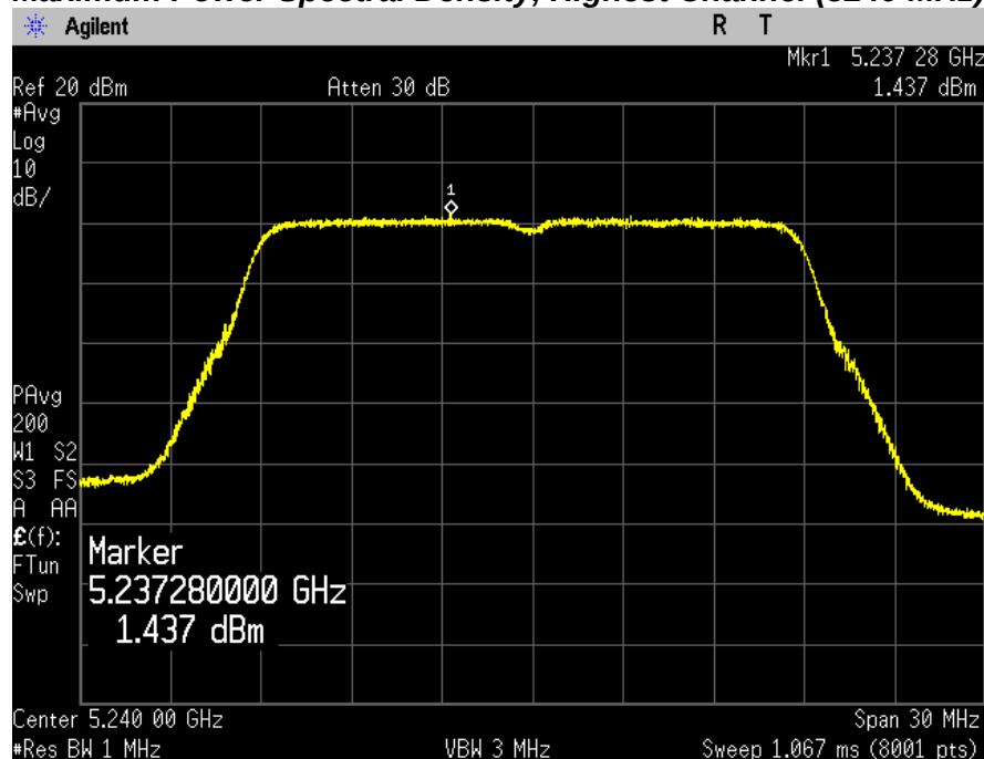
Maximum Power Spectral Density, Highest Channel (5240 MHz)
