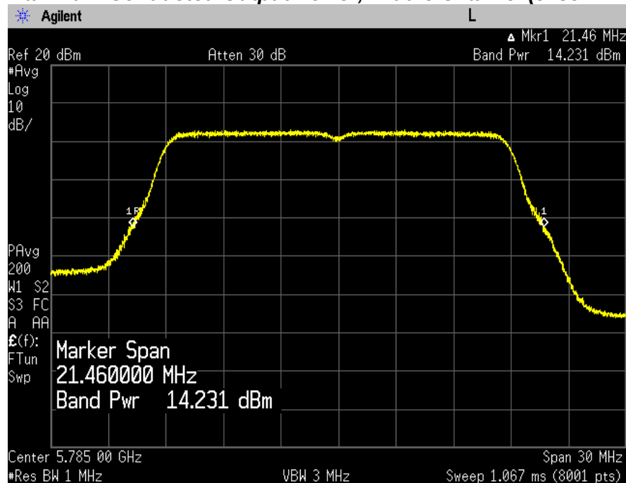
Maximum Conducted Output Power, Middle Channel (5785 MHz)
