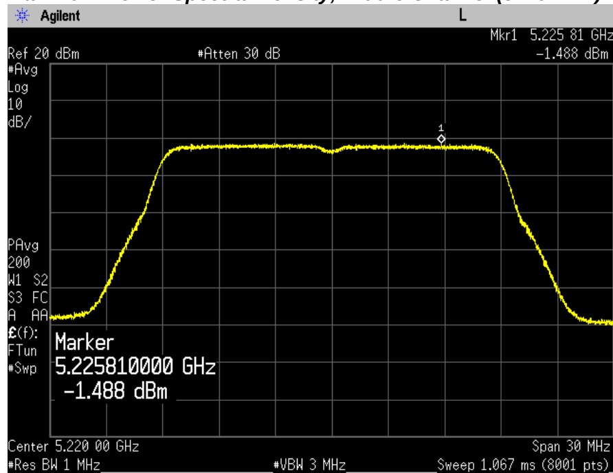
Maximum Power Spectral Density, Middle Channel (5220 MHz)
