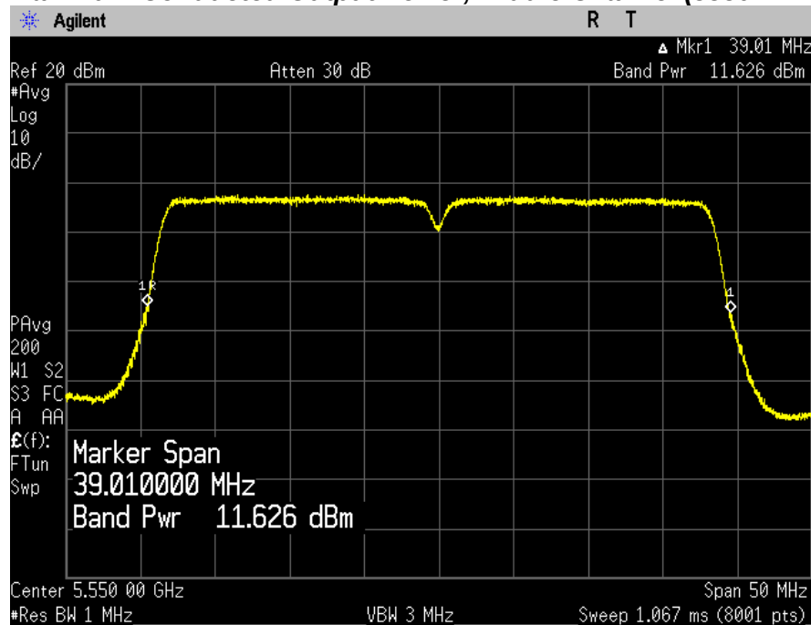
Maximum Conducted Output Power, Middle Channel (5550 MHz)
