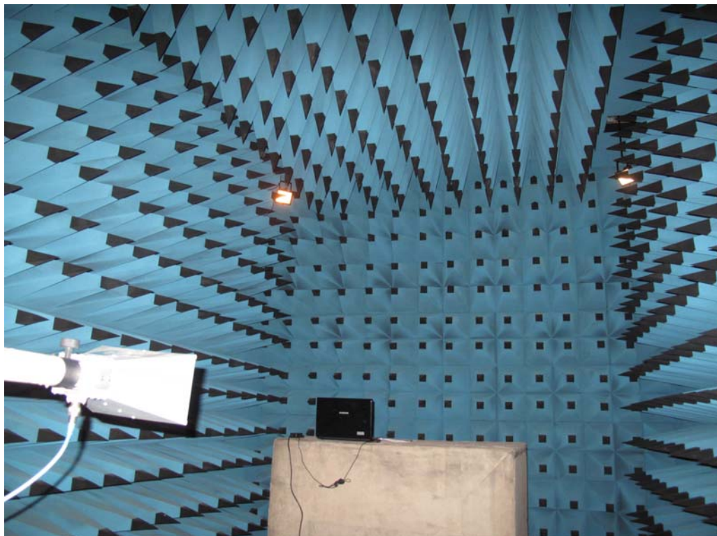
Radiated Test Picture(Rear)
