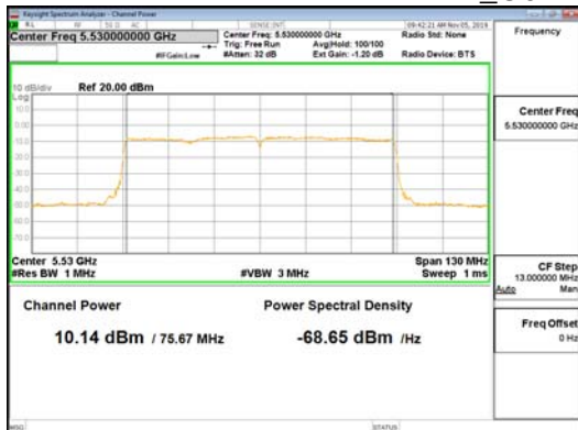
ANT-L_802.11ac_VHT80_UNII 2C
