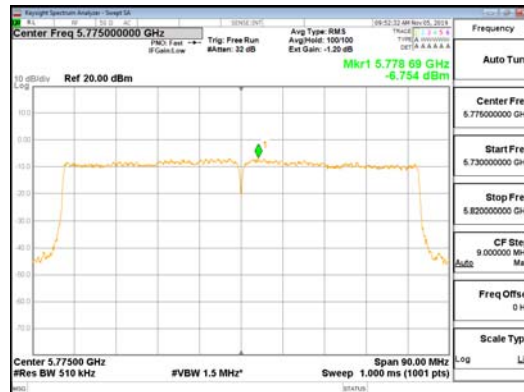
ANT-L_802.11ac_VHT80_UNII 3
