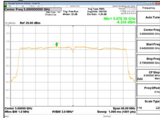
ANT-L_802.11ac_VHT80_UNII 2C
