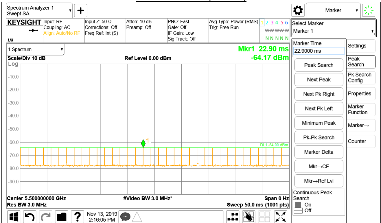
Radar Waveform (20 MHz)
