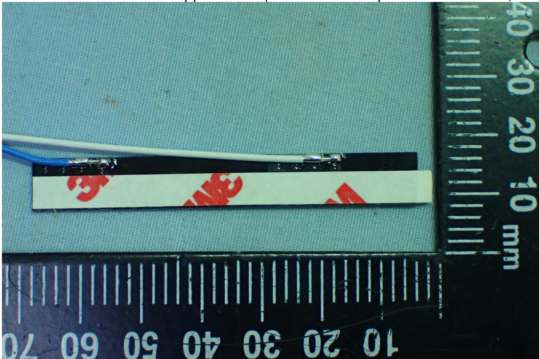
Figure 9 General Appearance (Antenna for Chipset: MT7915DUN, Back View)
