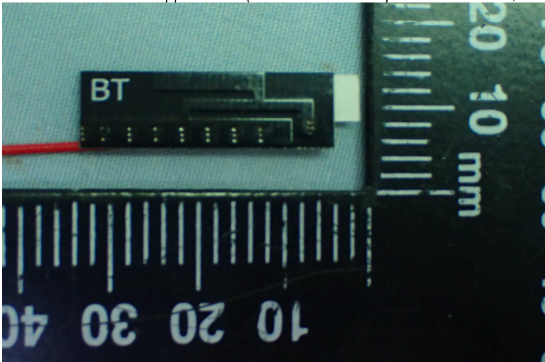
Figure 12 General Appearance (BT Antenna for Chipset:MT7668AUN, Front View)
