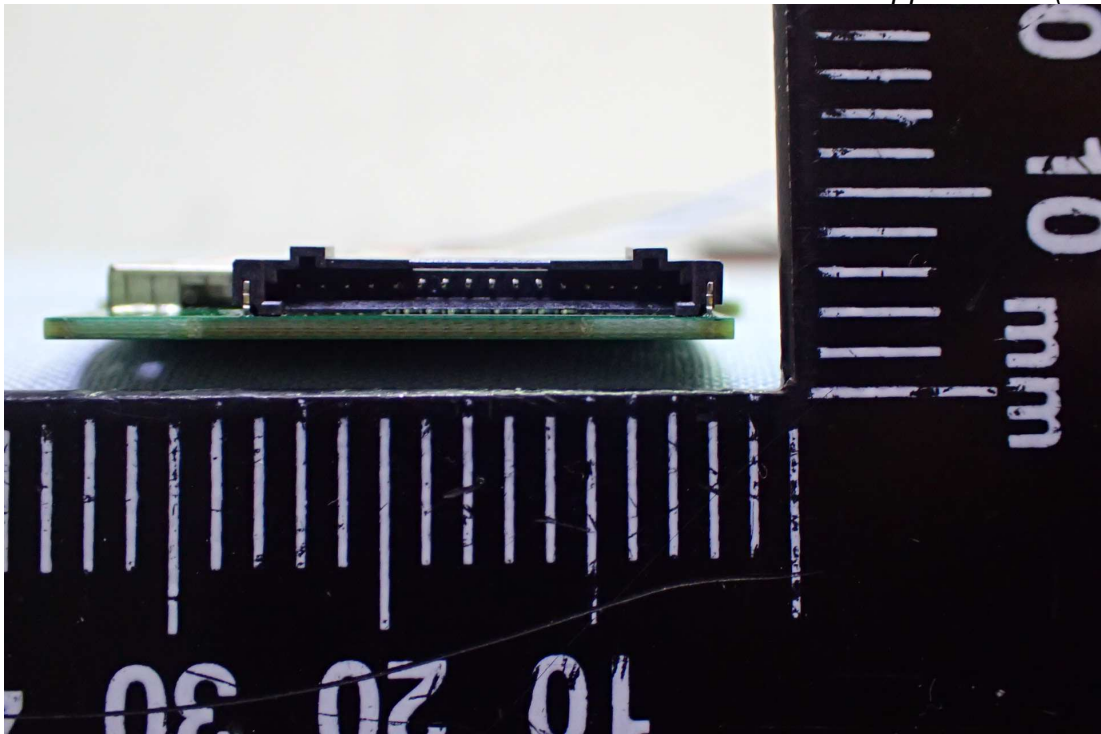
Figure 5 General Appearance (Side View)
