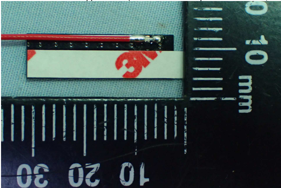
Figure 13 General Appearance (BT Antenna for Chipset:MT7668AUN, Back View)
