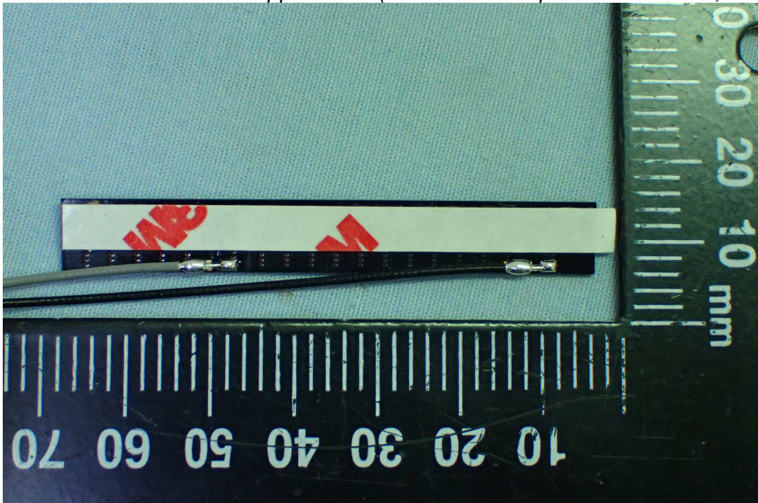
Figure 11 General Appearance (Antenna for Chipset:MT7668AUN, Back View)
