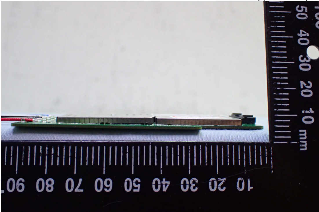
Figure 3 General Appearance (Side View)
