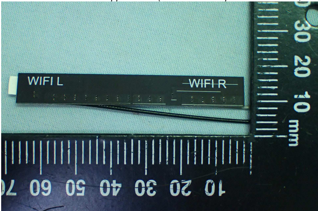
Figure 10 General Appearance (Antenna for Chipset: MT7668AUN, Front View)
