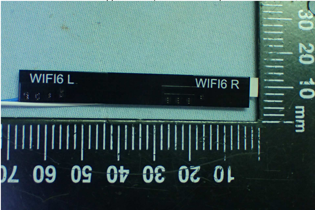
Figure 8 General Appearance (Antenna for Chipset: MT915DUN, Front View)
