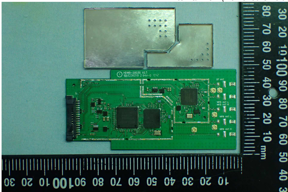
Figure 14 Internal View (Removed Shielded Case)
