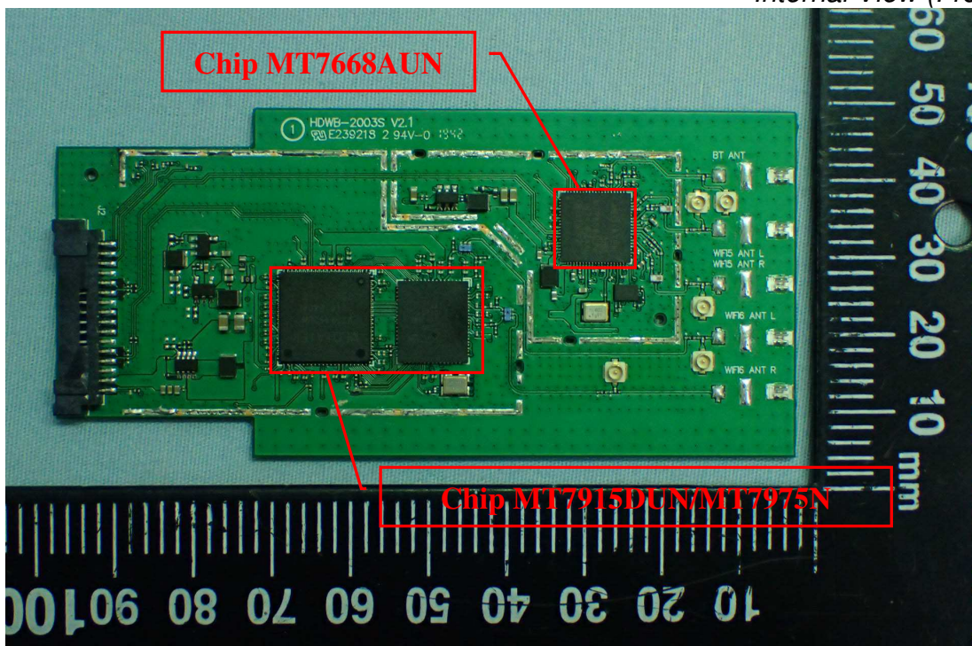
Figure 15 Internal View (Front View)
