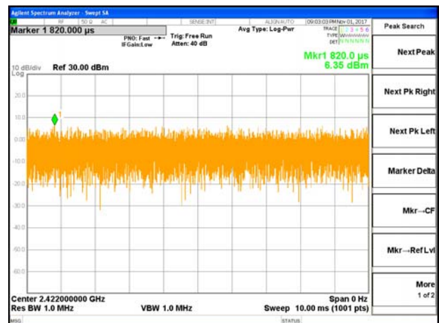
Duty Cycle_802.11n_HT40
