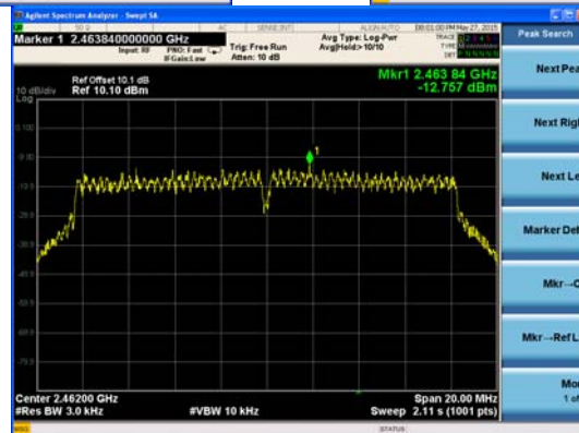
Ant : A1_802.11g
