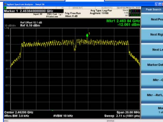
Ant : M3_802.11g
