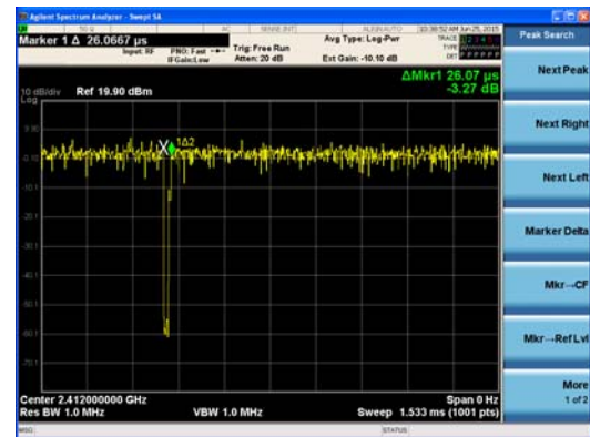
Duty Cycle_802.11g
