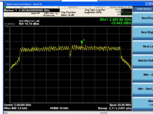
Ant : A3_802.11g
