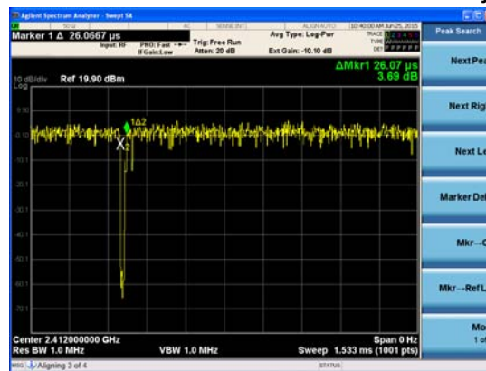
Duty Cycle_802.11n_HT20
