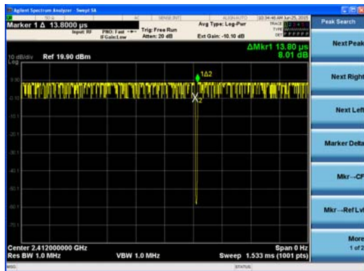
Duty Cycle_802.11b
