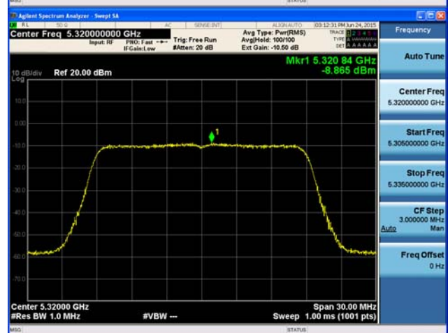
Ant : A3_802.11ac_VHT20 (1)
