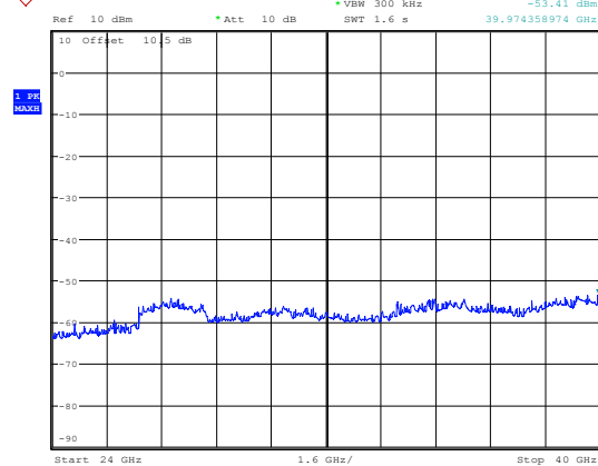
5260MHz 24GHz~40GHz
