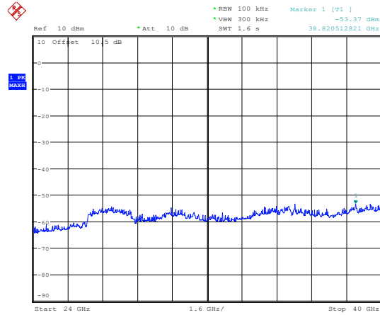
5260MHz 24GHz~40GHz
