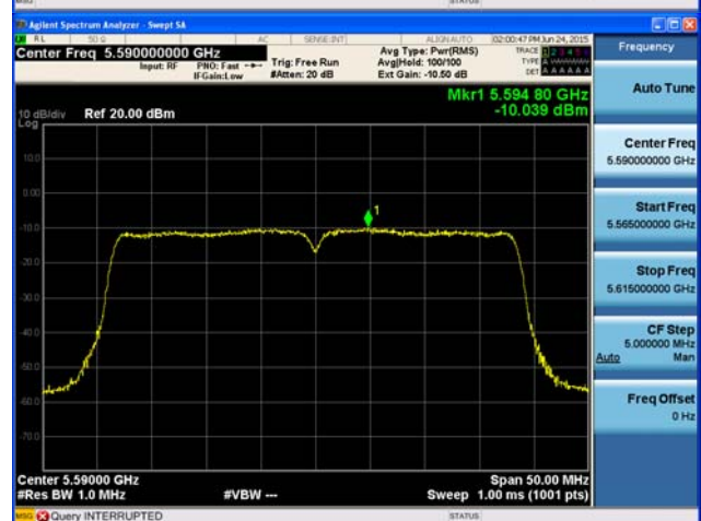
Ant : A2_802.11ac_VHT40 (1)
