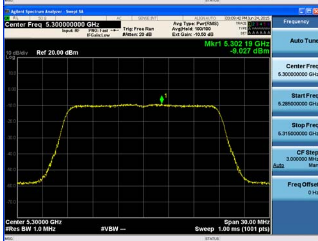
Ant : A3_802.11ac_VHT20 (1)
