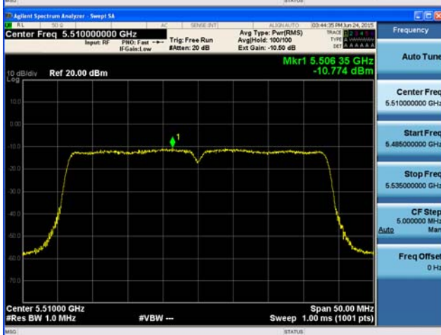
Ant : A3_802.11ac_VHT40 (1)
