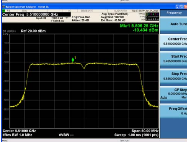
Ant : A2_802.11ac_VHT40 (1)
