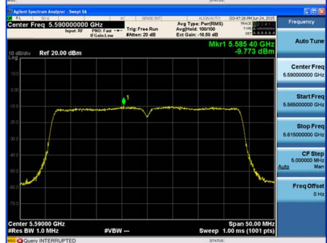
Ant : A3_802.11ac_VHT40 (1)
