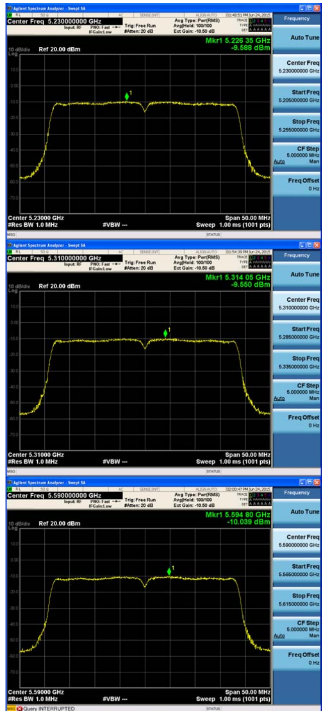
Ant : A2_802.11ac_VHT40 (1)
