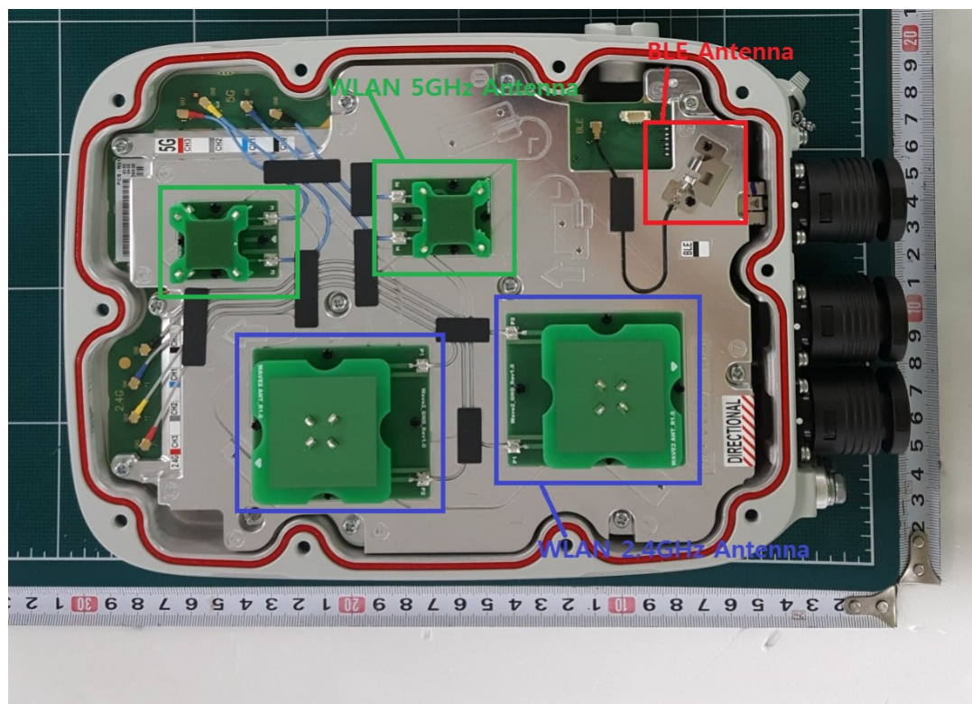
Antenna (WEA554d)
