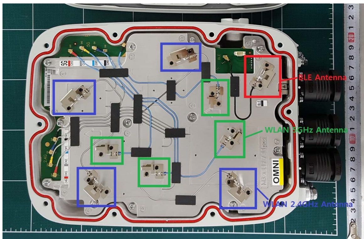
Antenna (WEA554i)
