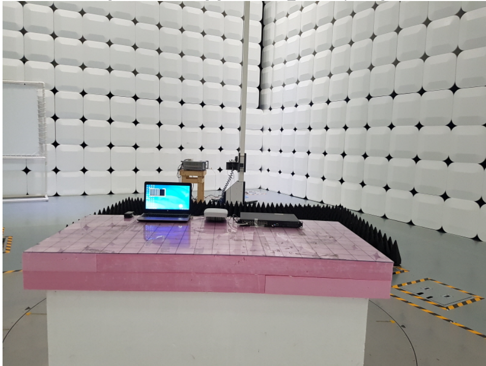
[1 GHz to 18 GHz] [WEA554d_POE, Optical]
