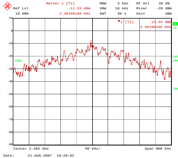
Figure 9. Plot of the Peak Power Spectral Density (Conducted)
