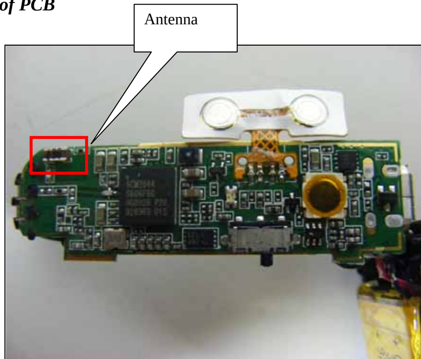
Bottom view of PCB
