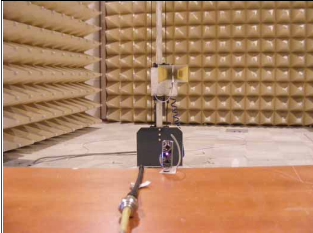
Photo of Test Set up for RSE
