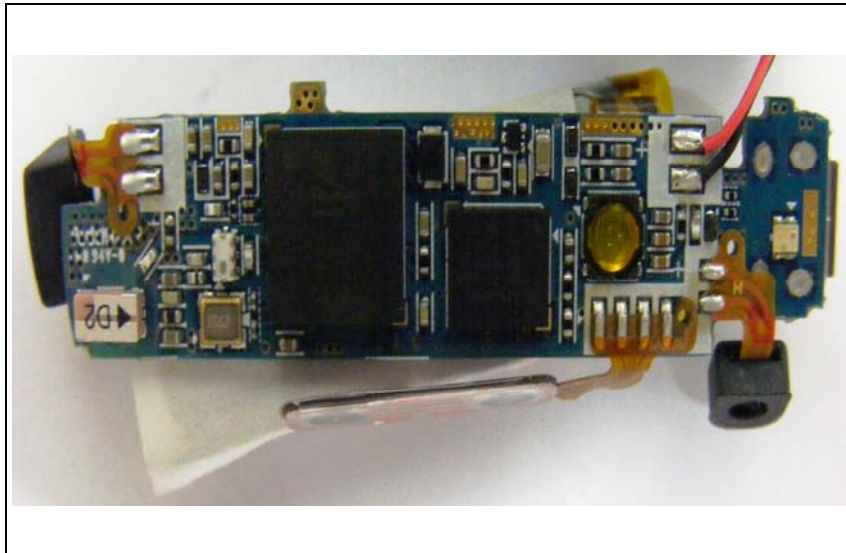
Top view of Main PCB
