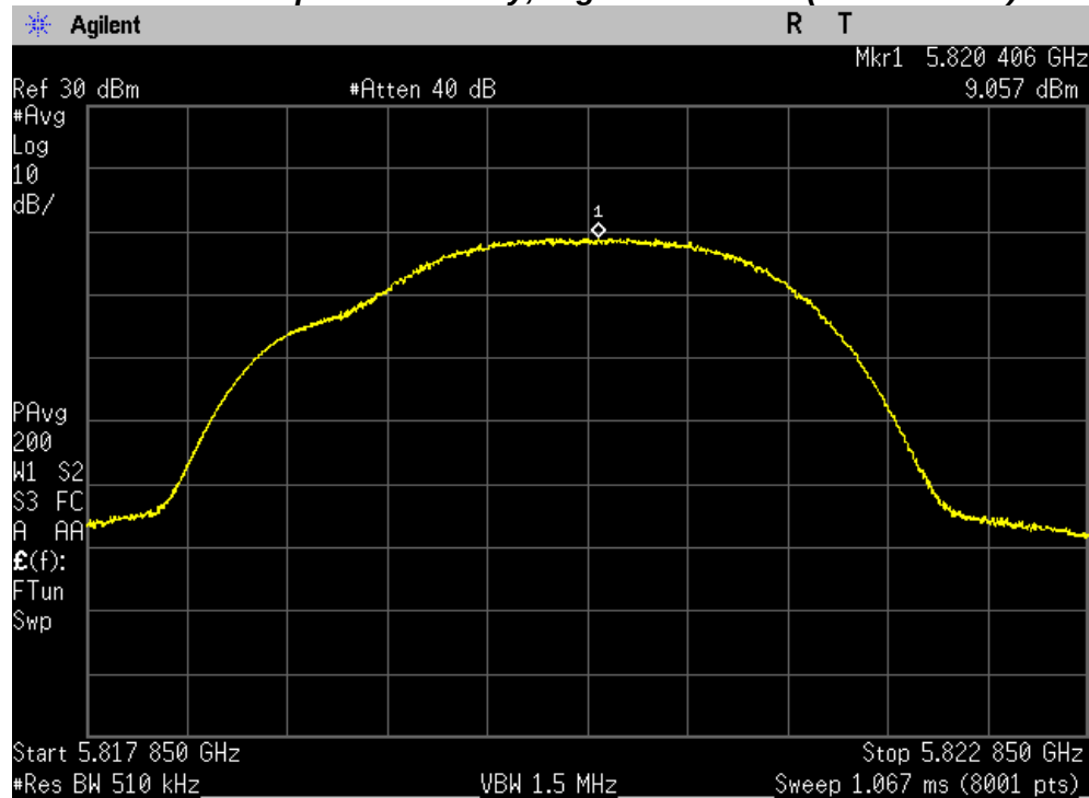
Maximum Power Spectral Density, Highest Channel (5820.35 MHz)
