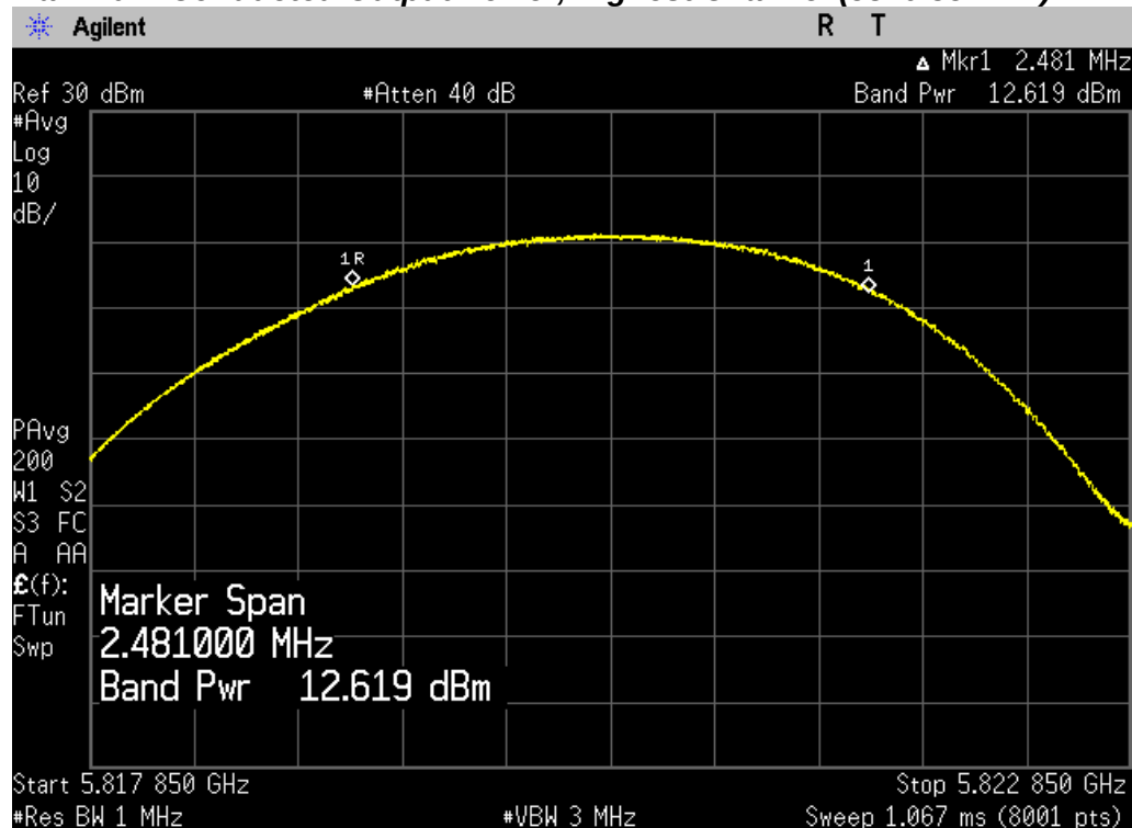
Maximum Conducted Output Power, Highest Channel (5820.35 MHz)
