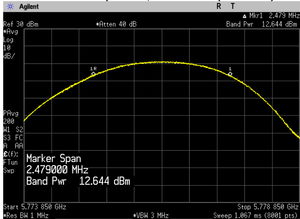
Maximum Conducted Output Power, Middle Channel (5776.35 MHz)
