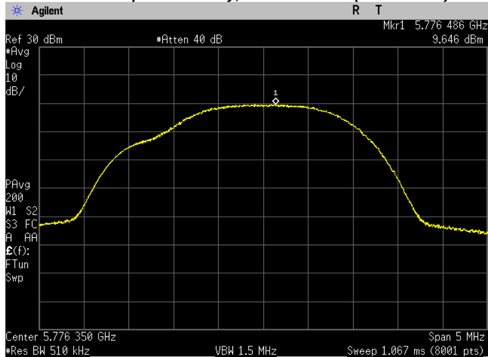
Maximum Power Spectral Density, Middle Channel (5776.35 MHz)
