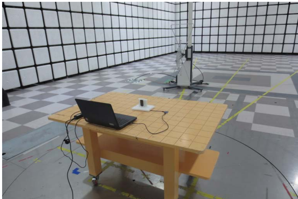
Radiated Test Picture(Rear)
