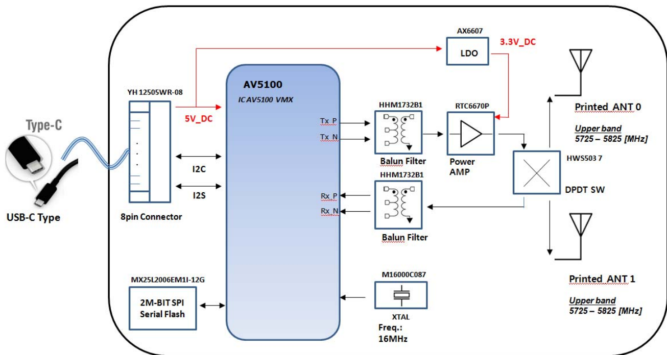
WHM520V block diagram
