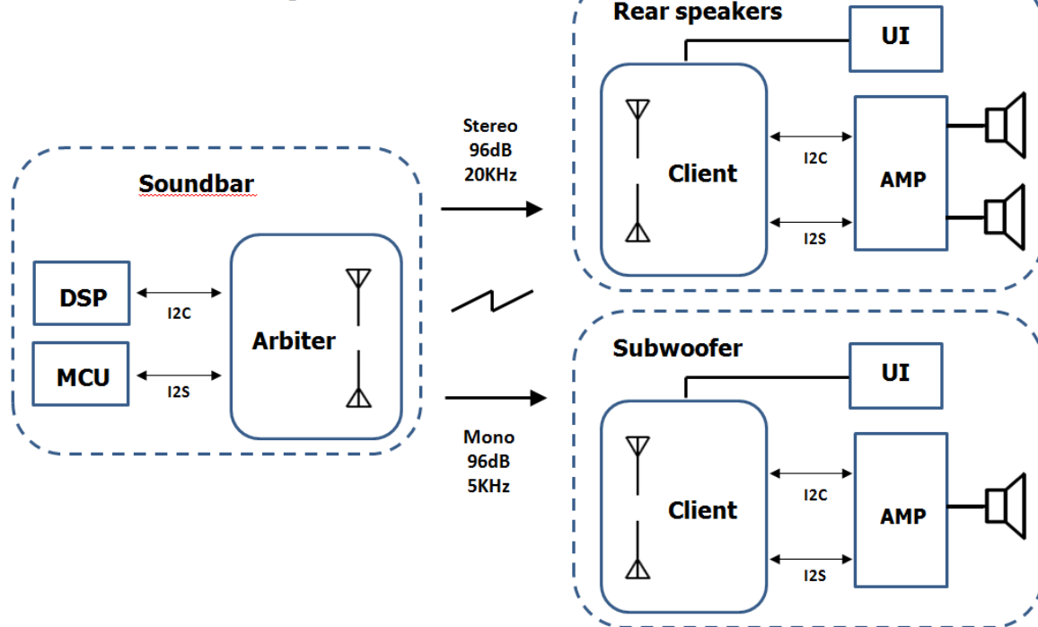
Wireless 2.1 Solution Diagram
