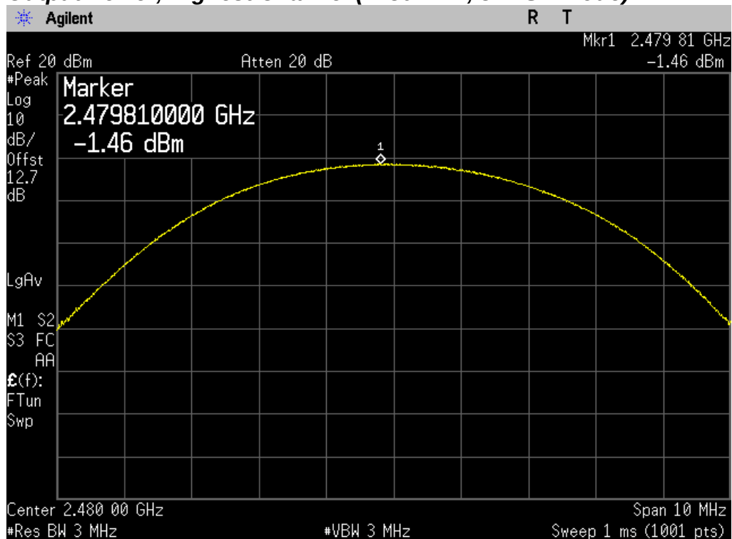
Output Power, Highest Channel (2480 MHz, 8DPSK Mode)
