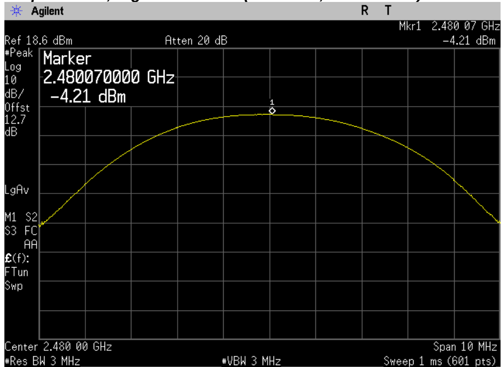
Output Power, Highest Channel (2480 MHz, GFSK Mode)
