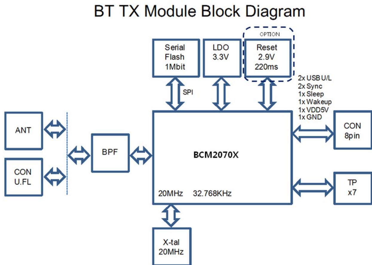
Figure 1-1 WIBT30A Major Components and System Interface
