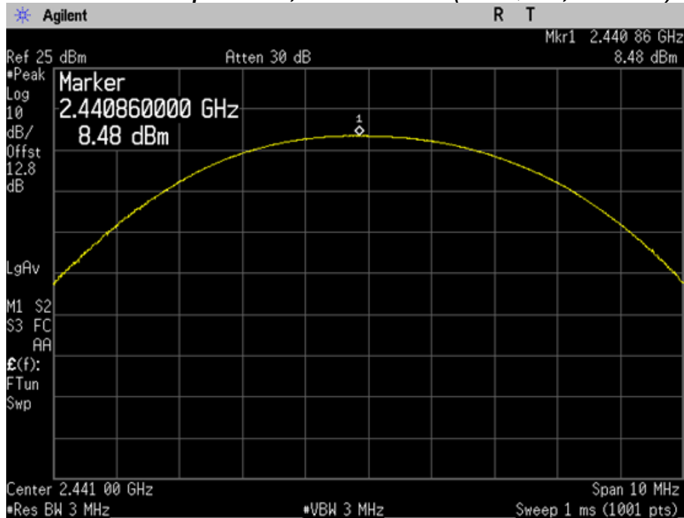
Maximum Peak Output Power, Middle channel ( \pi/4 DQPSK, 2441 MHz)
