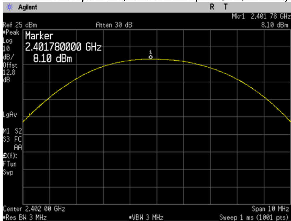
Maximum Peak Output Power, Lowest channel ( \pi/4 DQPSK, 2402 MHz)
