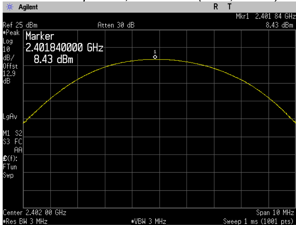
Maximum Peak Output Power, Lowest channel (8DPSK, 2402 MHz)
