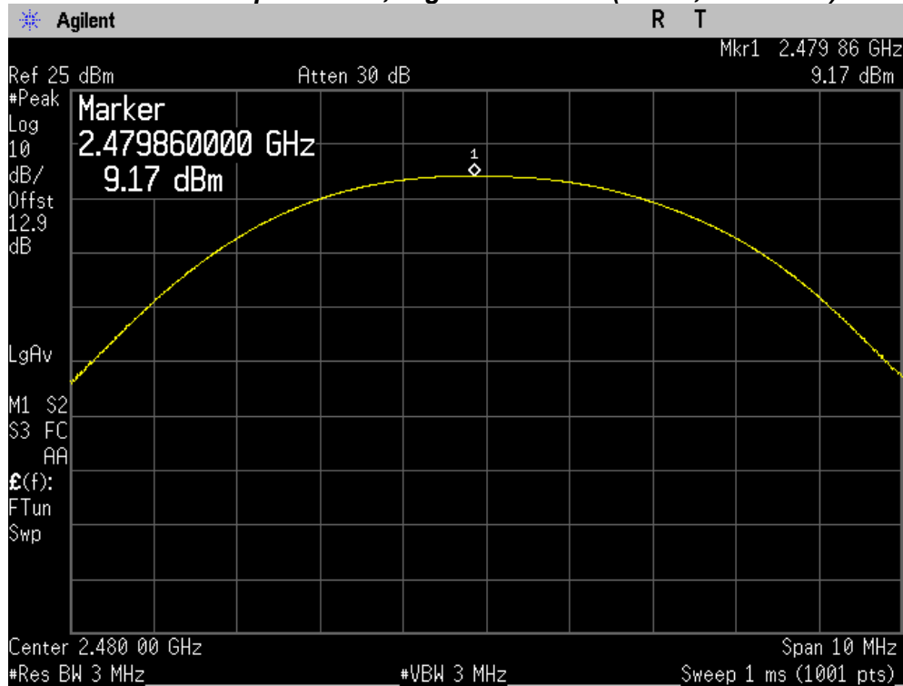
Maximum Peak Output Power, Highest channel (GFSK, 2480 MHz)
