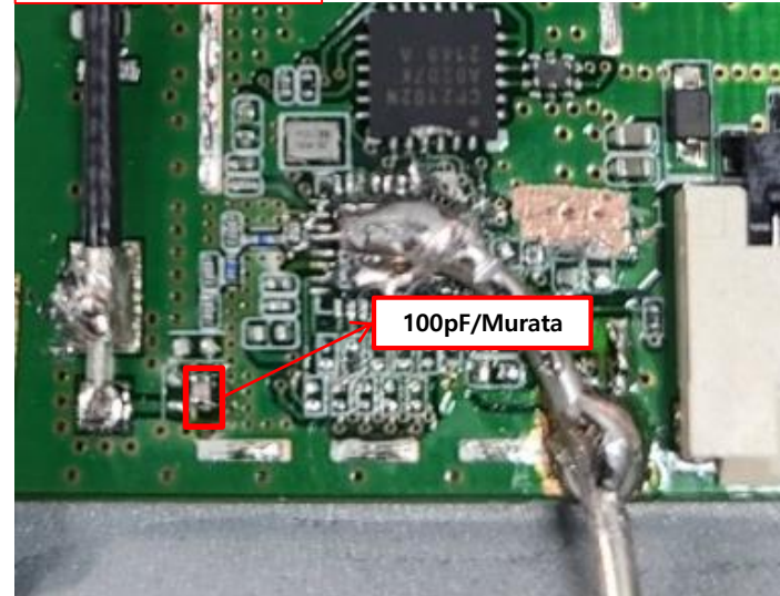
Matching Value
