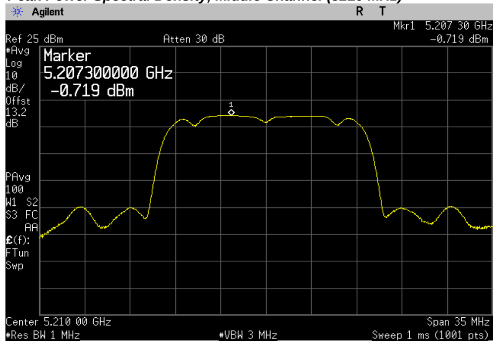
Peak Power Spectral Density, Middle Channel (5210 MHz)
