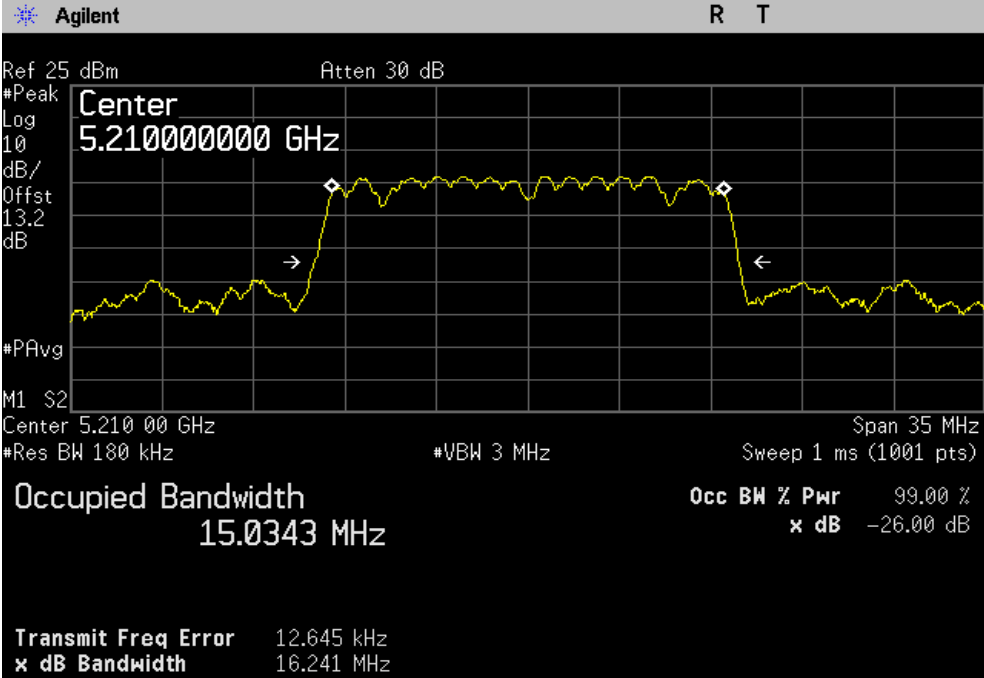
Bandwidth, Middle Channel (5210 MHz)
