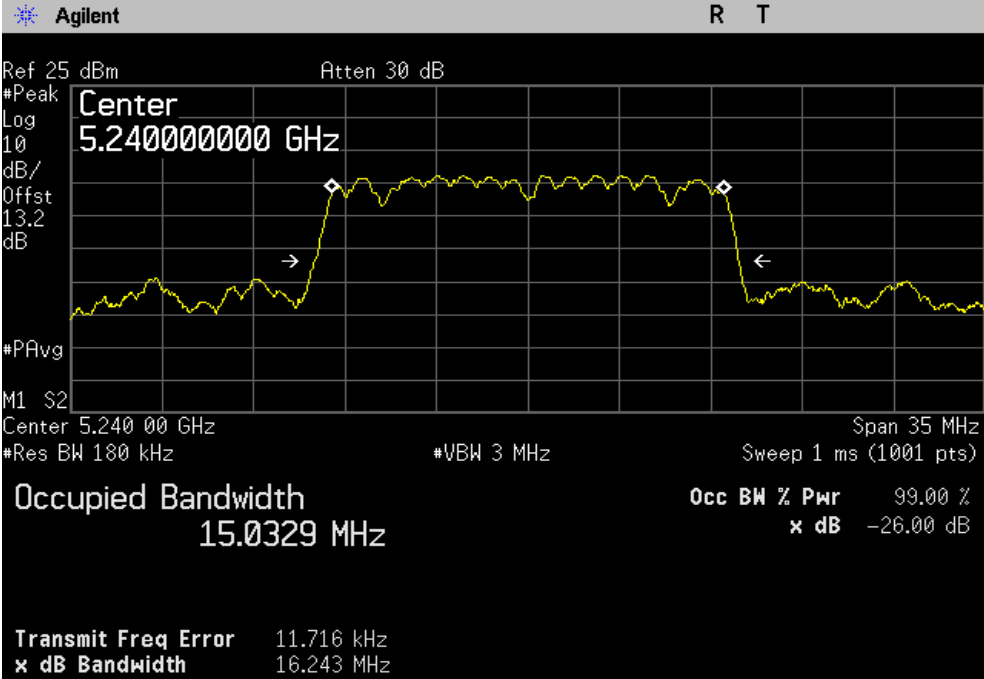
Bandwidth, Highest Channel (5240 MHz)
